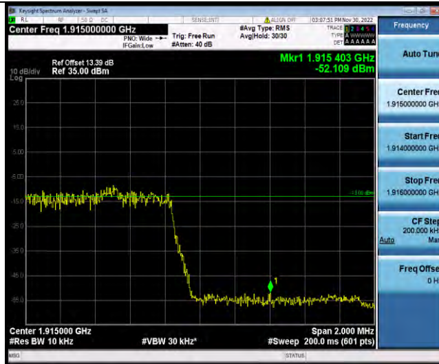
Band25-1.4MHz-QPSK-26683-1RB#5
