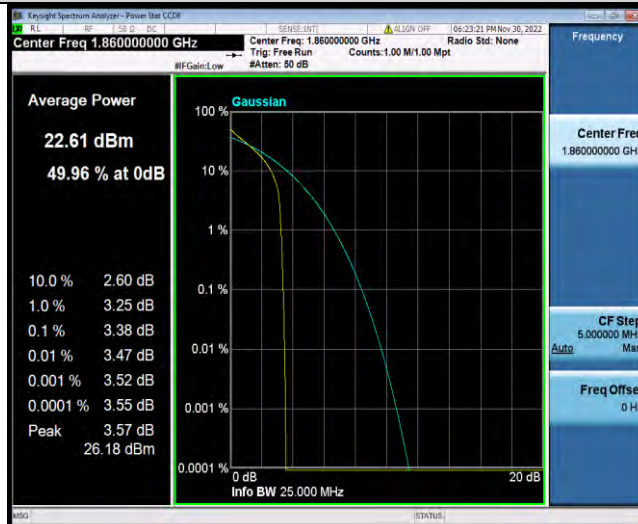
Band25-20MHz-QPSK-26140-100RB#0
