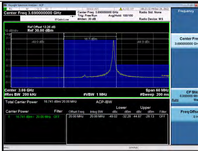
Band48-20MHz-QPSK-56640-100RB#0
