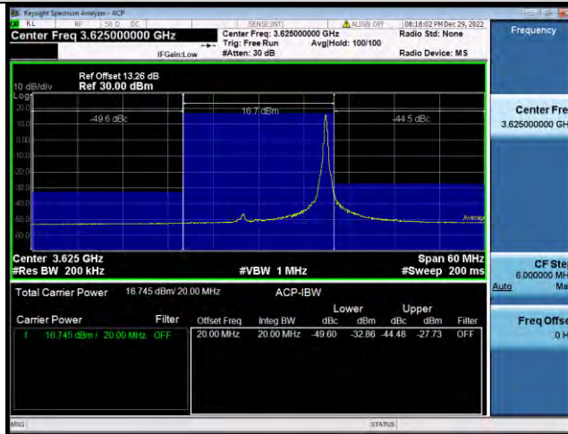
Band48-20MHz-QPSK-55990-100RB#0
