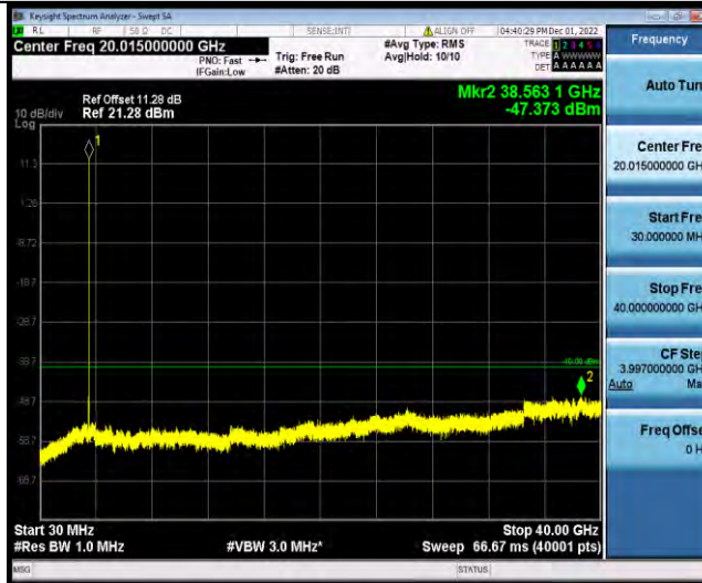
Band48-5MHz-QPSK-55990-1RB#0-Range1:30~40000MHz
