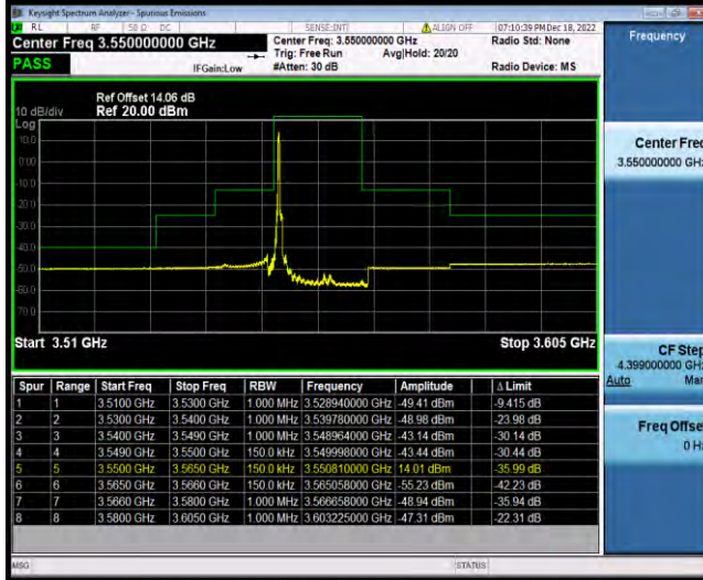
Band48-15MHz-QPSK-55315-1RB#74
