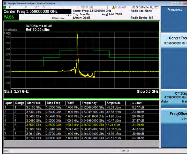
Band48-10MHz-QPSK-55290-1RB#49
