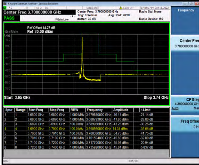
Band48-10MHz-16QAM-56690-1RB#49
