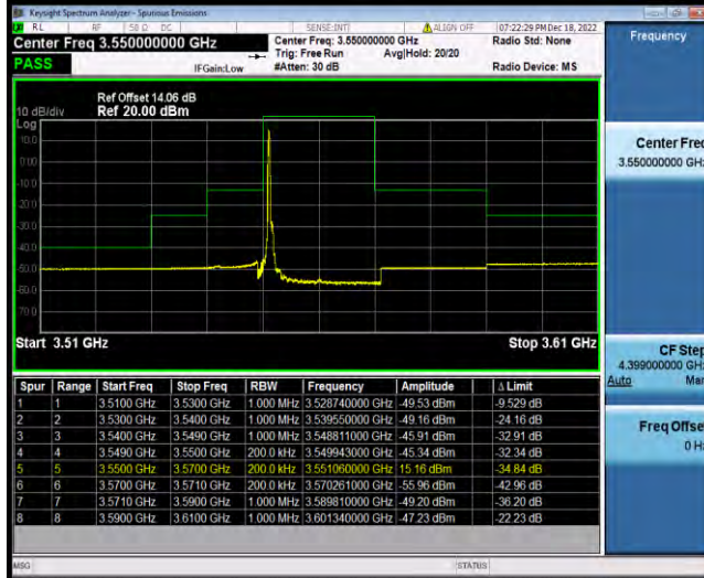
Band48-20MHz-64QAM-55340-1RB#99
