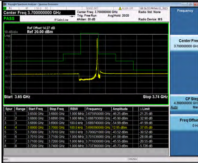
Band48-10MHz-16QAM-56690-50RB#0
