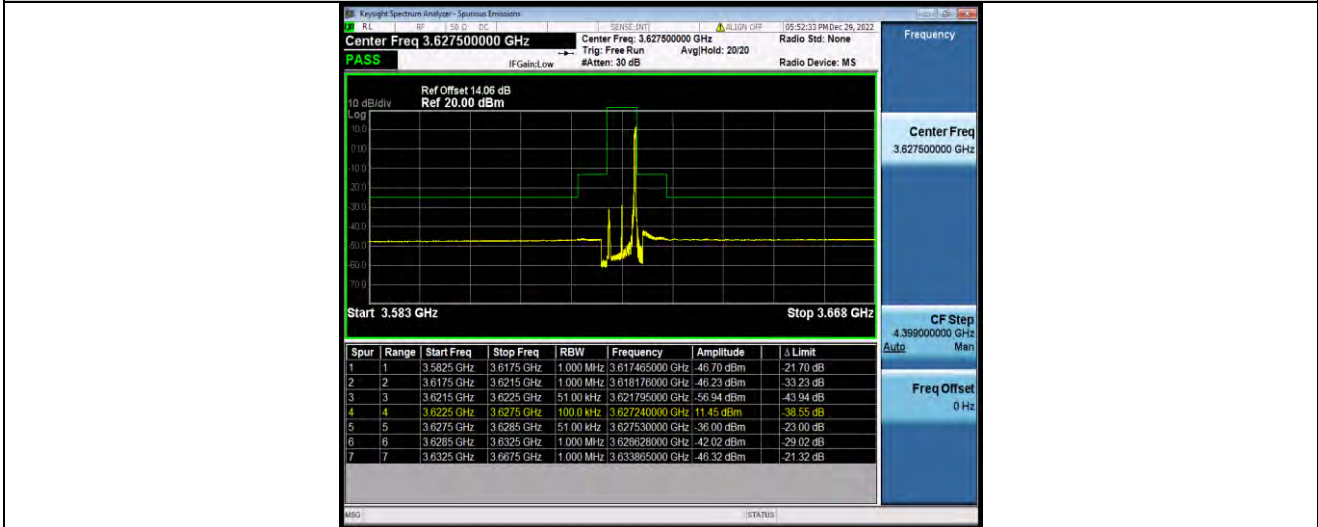
Band48-5MHz-64QAM-55990-25RB#0
