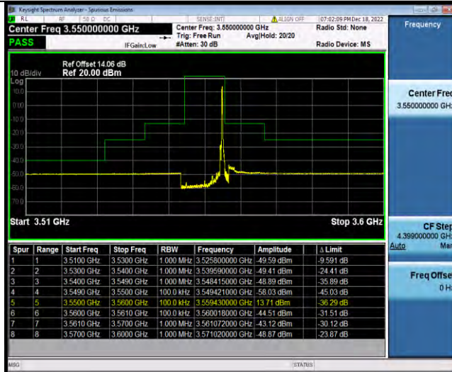
Band48-10MHz-64QAM-55290-50RB#0
