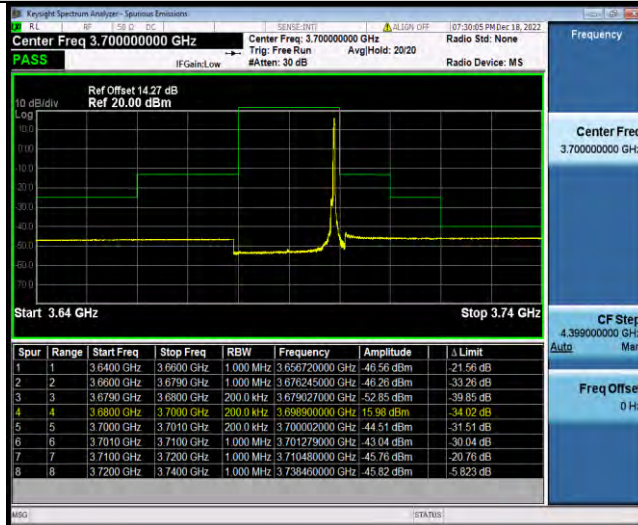
Band48-20MHz-16QAM-56640-100RB#0
