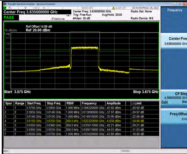
Band48-20MHz-16QAM-56640-1RB#0
