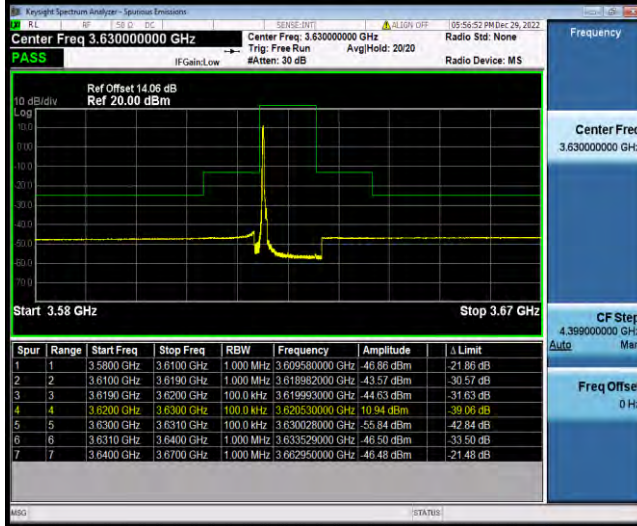
Band48-10MHz-64QAM-55990-1RB#49
