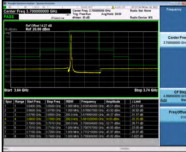
Band48-20MHz-16QAM-56640-1RB#99
