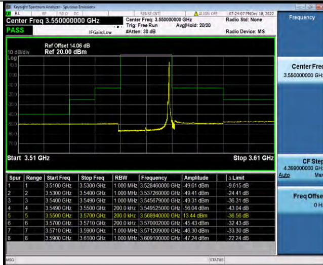
Band48-20MHz-64QAM-55340-100RB#0
