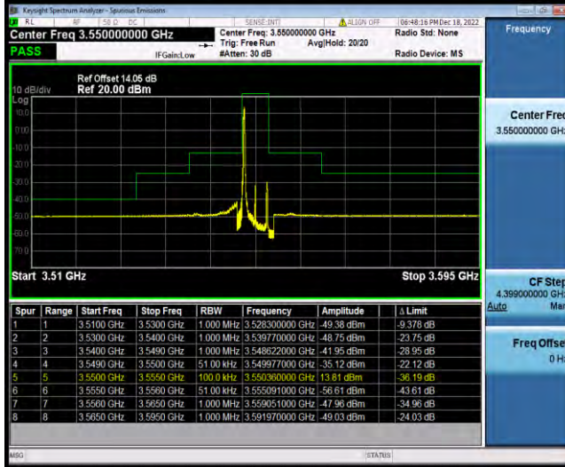
Band48-5MHz-16QAM-55265-1RB#24
