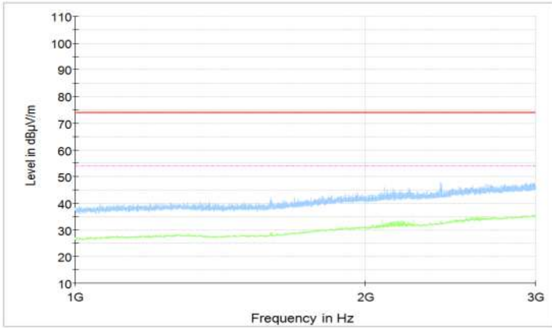
Figure A.72 Radiated Emission (Set.3, Data Transfer Mode: TF Card To PC, 1GHz to 3GHz)
