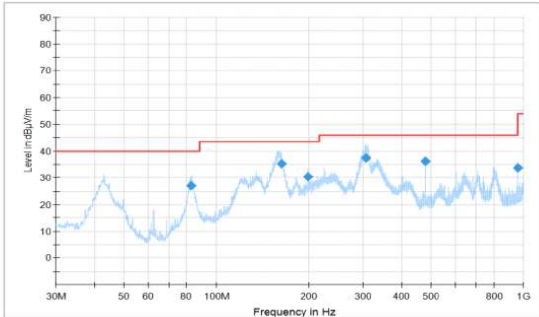
Figure A.61 Radiated Emission (Set.3, Data Transfer Mode: PC To EUT , 30MHz to 1GHz)
