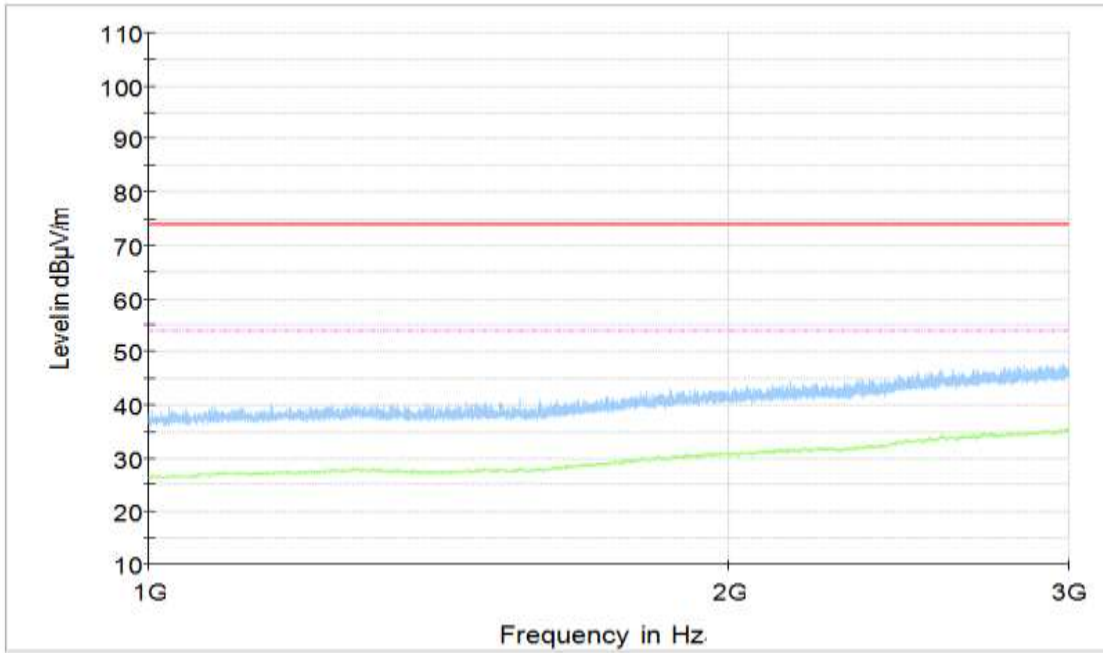
Figure A.47 Radiated Emission (Set.1, Video Player Mode , 1GHz to 3GHz)
