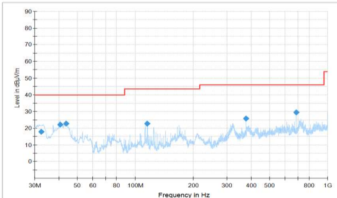
Figure A.26 Radiated Emission (Set.1, Charging and LTE Band 14 idle , 30MHz to 1GHz)
