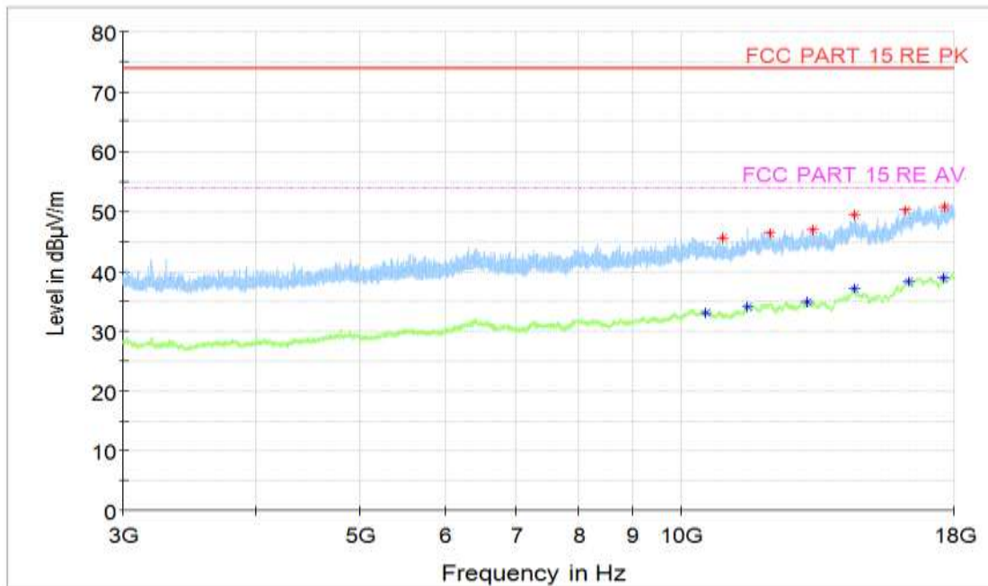
Figure A.63 Radiated Emission (Set.3, Data Transfer Mode: PC To EUT, 3GHz to 18GHz)
