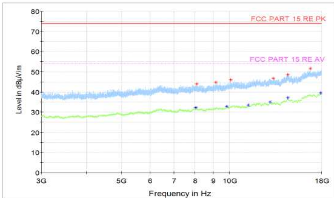
Figure A.13 Radiated Emission (Set.1, Charging and LTE Band 5 idle, 3GHz to 18GHz)
