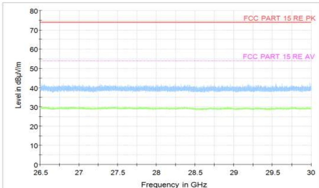
Figure A.65 Radiated Emission (Set.3, Data Transfer Mode: PC To EUT, 26.5GHz to 30GHz)
