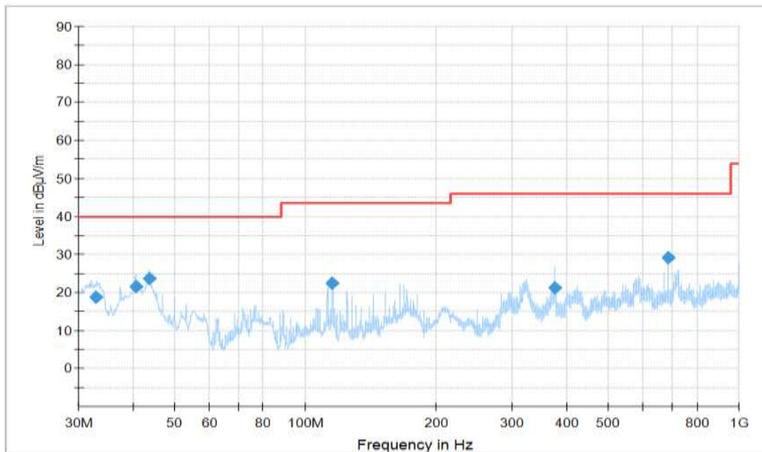
Figure A.36 Radiated Emission (Set.1, Charging and LTE Band 26 idle , 30MHz to 1GHz)
