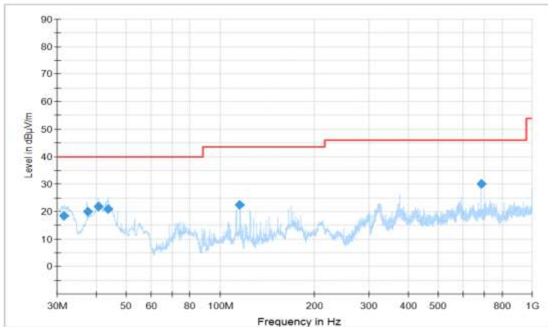
Figure A.16 Radiated Emission (Set.1, Charging and LTE Band 12 idle , 30MHz to 1GHz)
