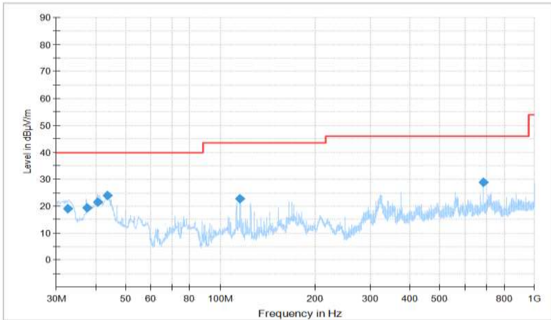
Figure A.21 Radiated Emission (Set.1, Charging and LTE Band 13 idle , 30MHz to 1GHz)
