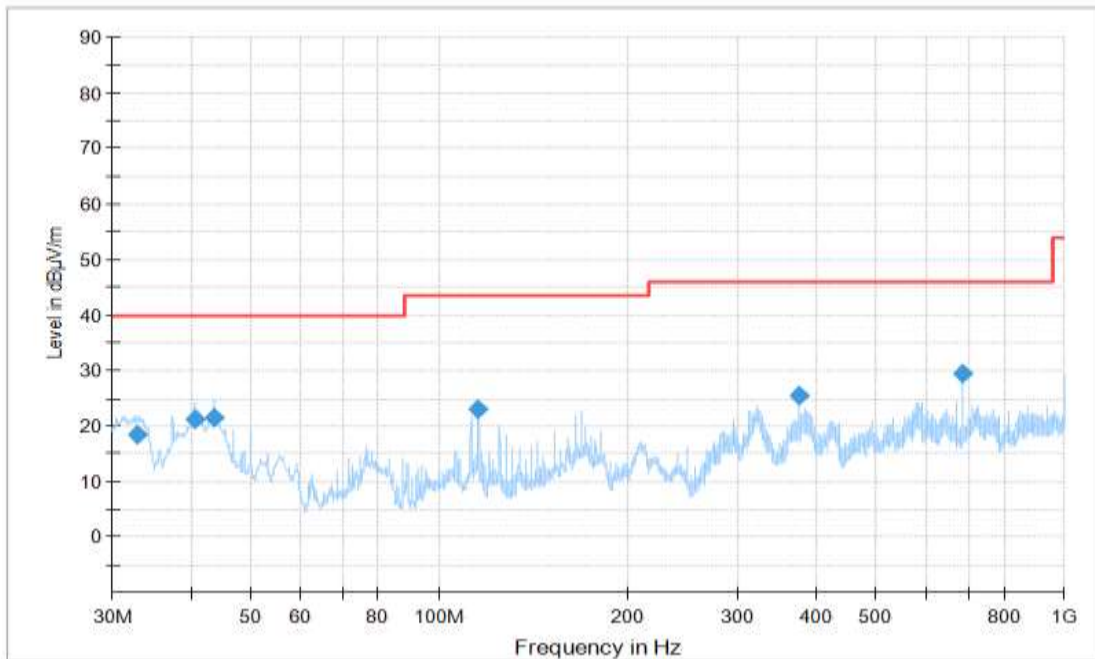
Figure A.31 Radiated Emission (Set.1, Charging and LTE Band 17 idle , 30MHz to 1GHz)
