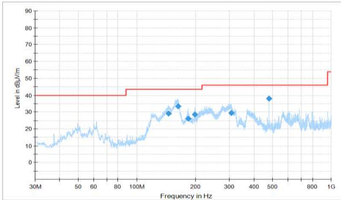
Figure A.56 Radiated Emission (Set.3, Data Transfer Mode: EUT To PC , 30MHz to 1GHz)
