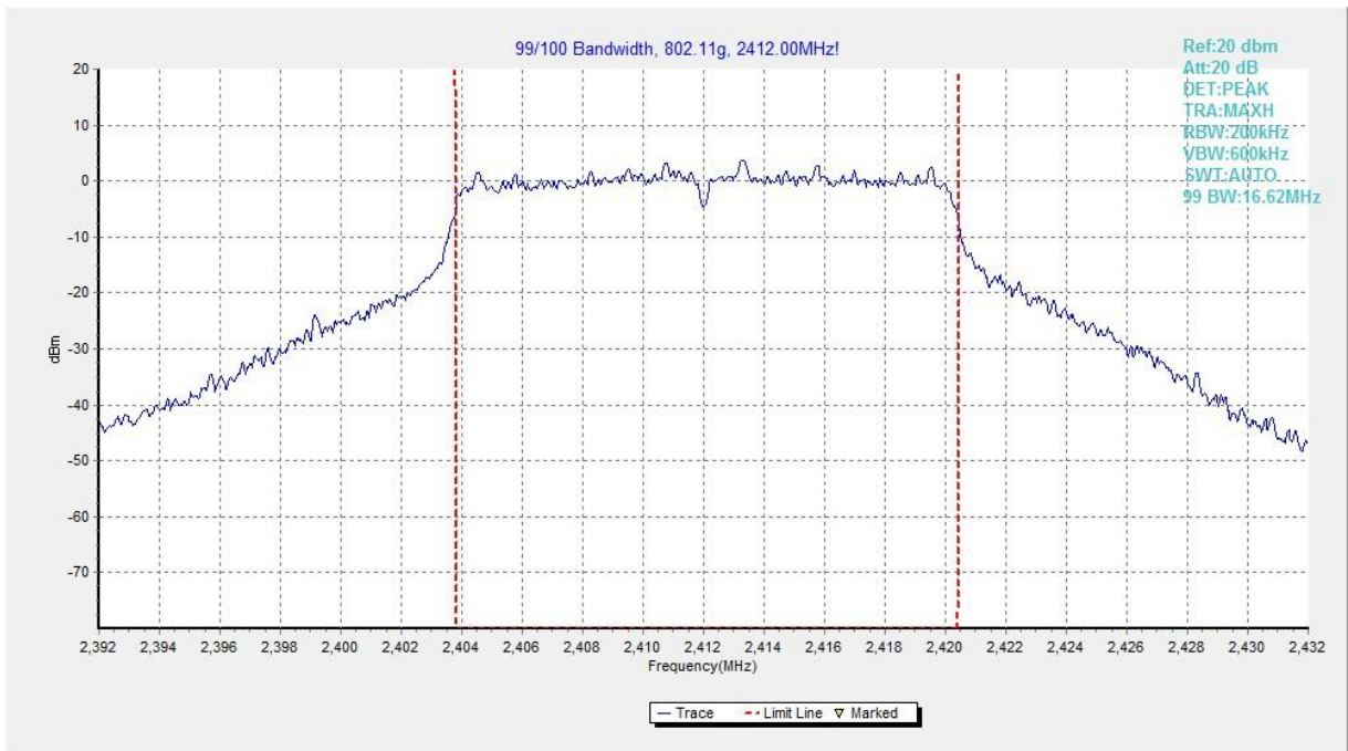
Fig.74 99% Occupied Bandwidth (802.11g, CH 1)
