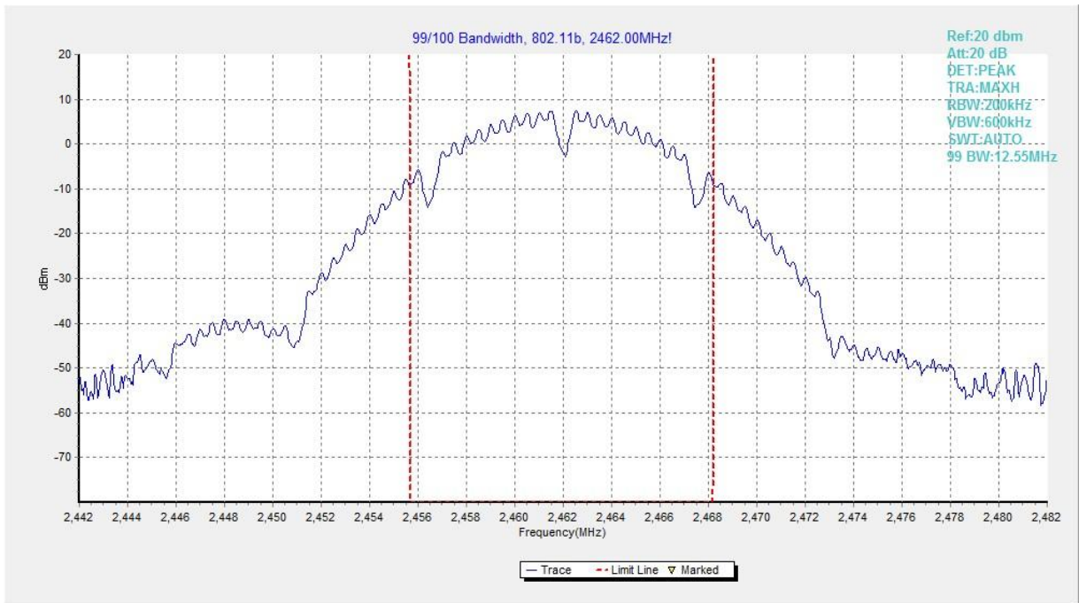
Fig.73 99% Occupied Bandwidth (802.11b, CH 11)
