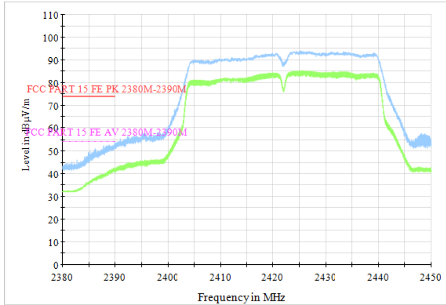
Fig.64 Radiated Restricted Band (802.11n HT40, CH3, 2.38GHz~2.45GHz)
