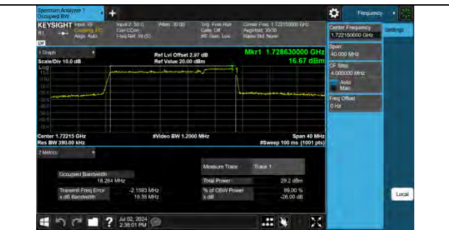
66-66-15MHz-5MHz-16QAM-16QAM-132047-132140-75 RB#0-25RB#0-PASS
