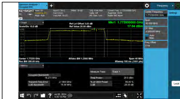
66-66-15MHz-5MHz-QPSK-QPSK-132549-132642-75R B#0-25RB#0-PASS
