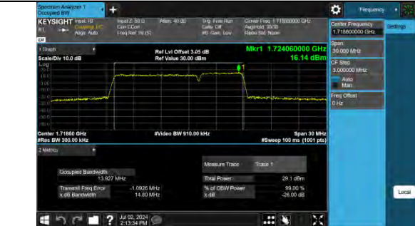
66-66-10MHz-5MHz-16QAM-16QAM-132022-132094-50 RB#0-25RB#0-PASS
