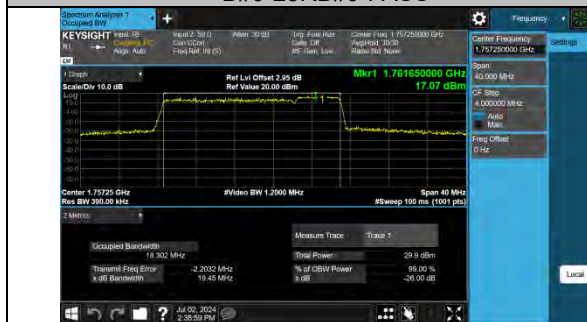
66-66-15MHz-5MHz-16QAM-16QAM-132398-132491-75 RB#0-25RB#0-PASS
