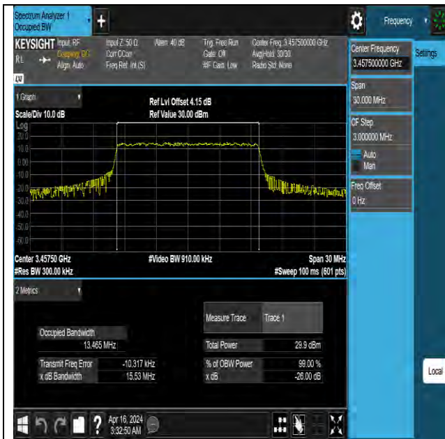
42(3450-3550)-15MHz-QPSK-42165-75RB#0-PASS
