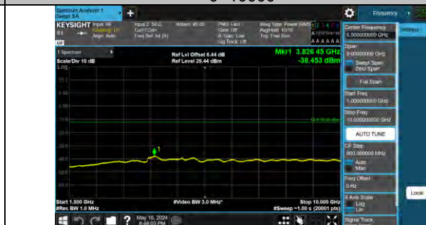
Band71_15MHz_QPSK_133297_1RB#0_1000~10000_100 0~10000
