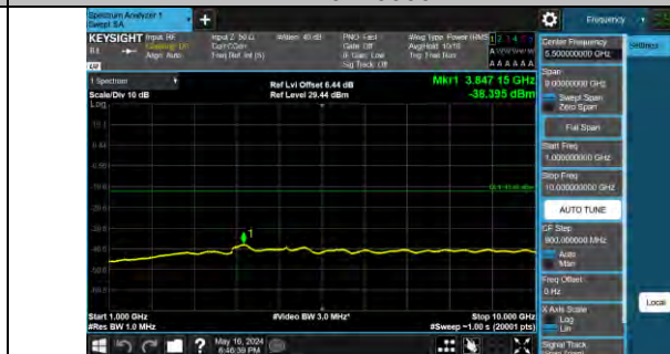
Band71_15MHz_QPSK_133197_1RB#0_1000~10000_100 0~10000
