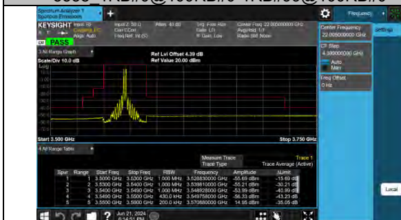
20MHz-20MHz_QPSK@QPSK-QPSK@QPSK_55340-5 5538 1RB#99@100RB#0-1RB#0@100RB#0
