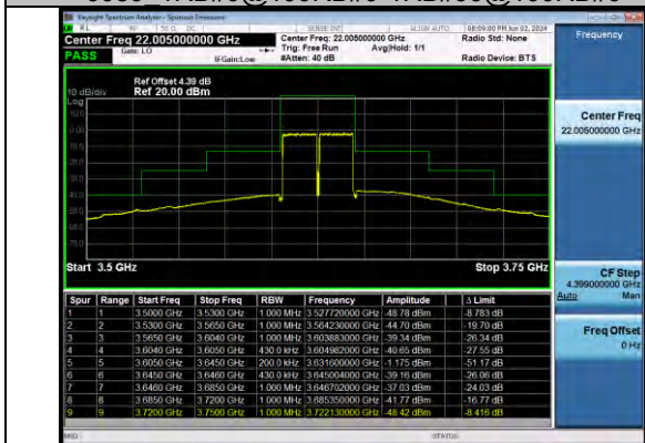
20MHz-20MHz_QPSK@QPSK-QPSK@QPSK_55891-5 6089 100RB#0@100RB#0-100RB#0@100RB#0
