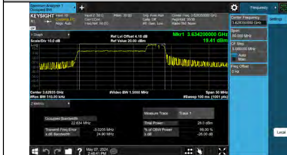
48-48-20MHz-5MHz-16QAM-16QAM-55965-56082-100R B#0-25RB#0-PASS
