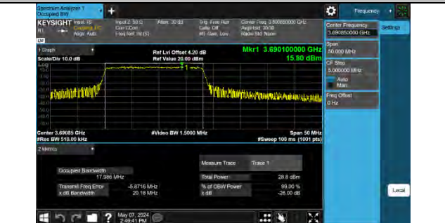
48-48-20MHz-5MHz-16QAM-16QAM-56590-56707-100R B#0-25RB#0-PASS
