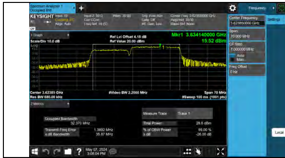
48-48-15MHz-20MHz-16QAM-16QAM-55893-56064-75R B#0-100RB#0-PASS
