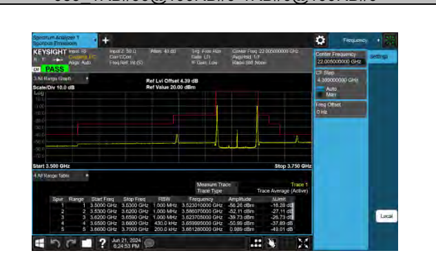
20MHz-20MHz_QPSK@QPSK-QPSK@QPSK_56442-56 640 1RB#0@100RB#0-1RB#99@100RB#0
