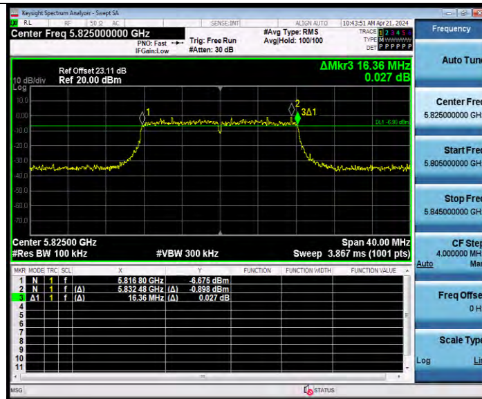
11A-CDD Ant9 5825
