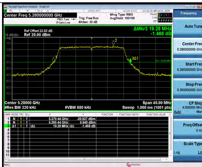
11A-CDD Ant9 5280
