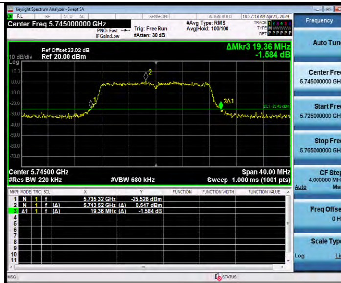
11A-CDD Ant9 5745
