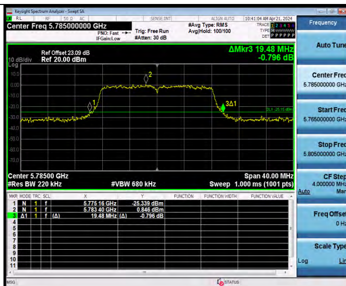
11A-CDD Ant9 5785
