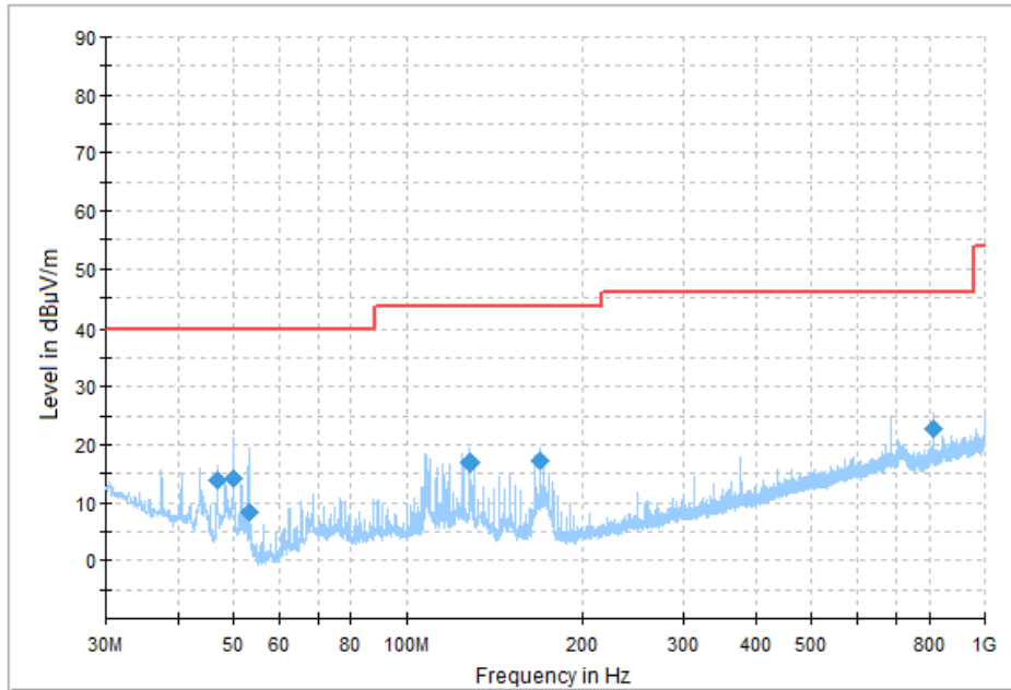
Fig.53 Radiated Spurious Emission (Ch19, 30 MHz - 1 GHz), 2M
