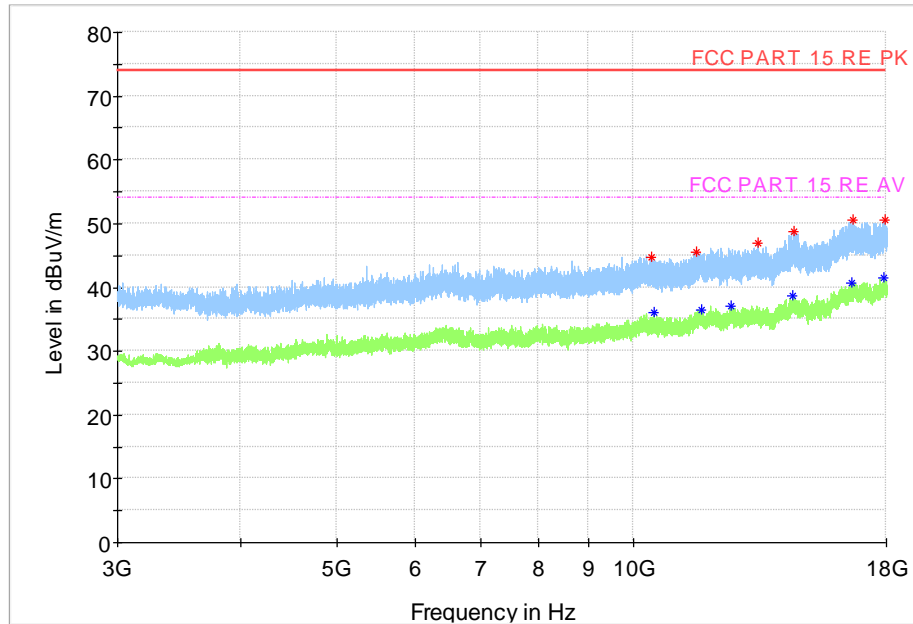
Fig.55 Radiated Spurious Emission (Ch19, 3 GHz - 18 GHz), 2M
