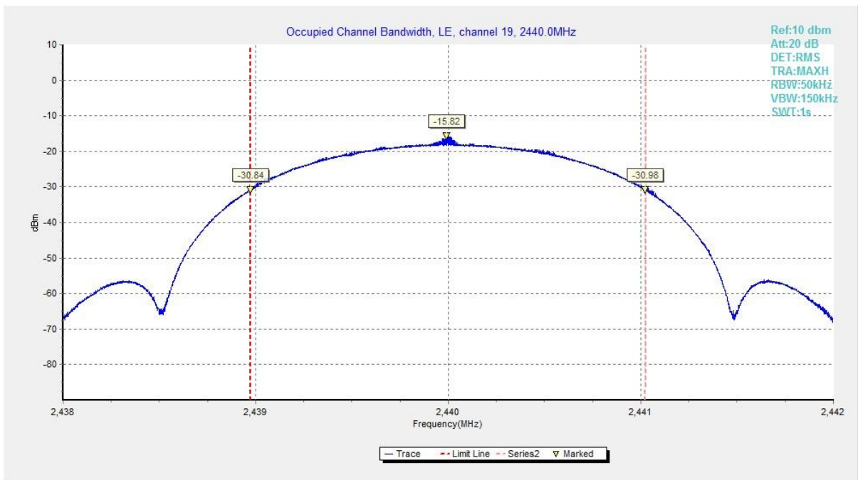
Fig.69 Occupied Bandwidth (Ch 19), 2M
