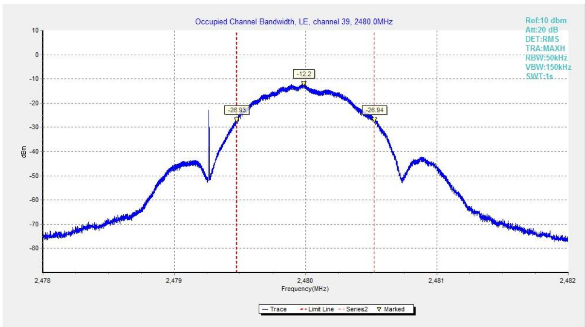
Fig.67 Occupied Bandwidth (Ch 39), 1M
