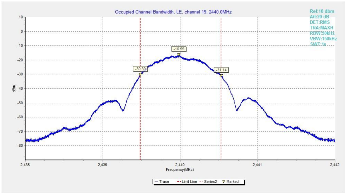
Fig.66 Occupied Bandwidth (Ch 19), 1M
