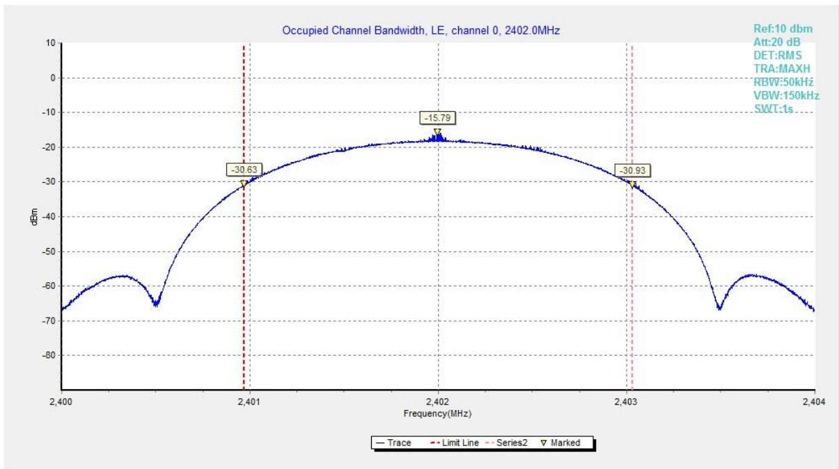
Fig.68 Occupied Bandwidth (Ch 0), 2M
