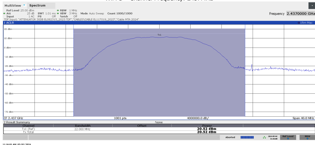
WiFi b – Channel Frequency: 2437MHz
