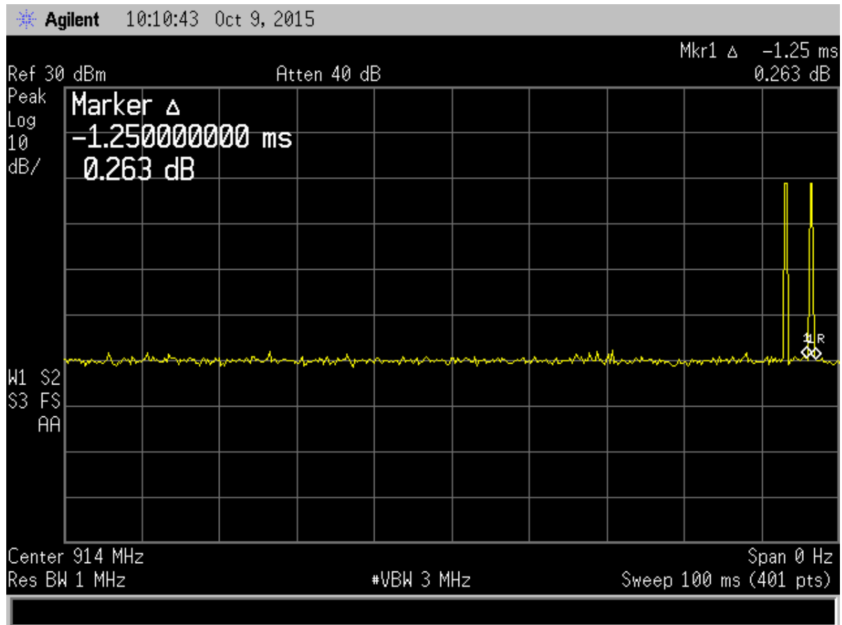
Figure 3. Pulse Width #2
