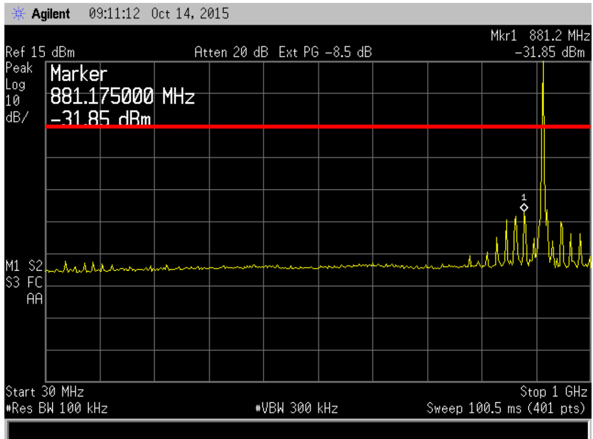
Figure 6. Antenna Conducted Emissions Mid, Part 1
