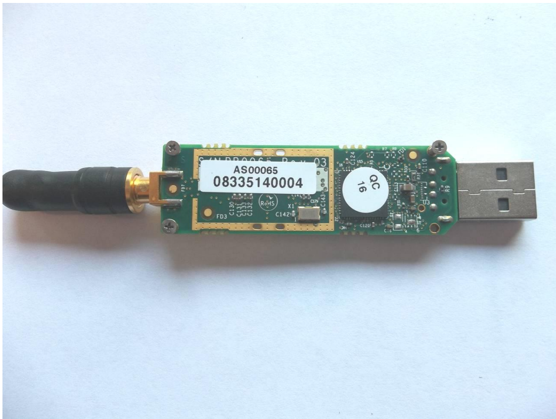
Figure 2. Back of Zigbee Radio Removed from Case
