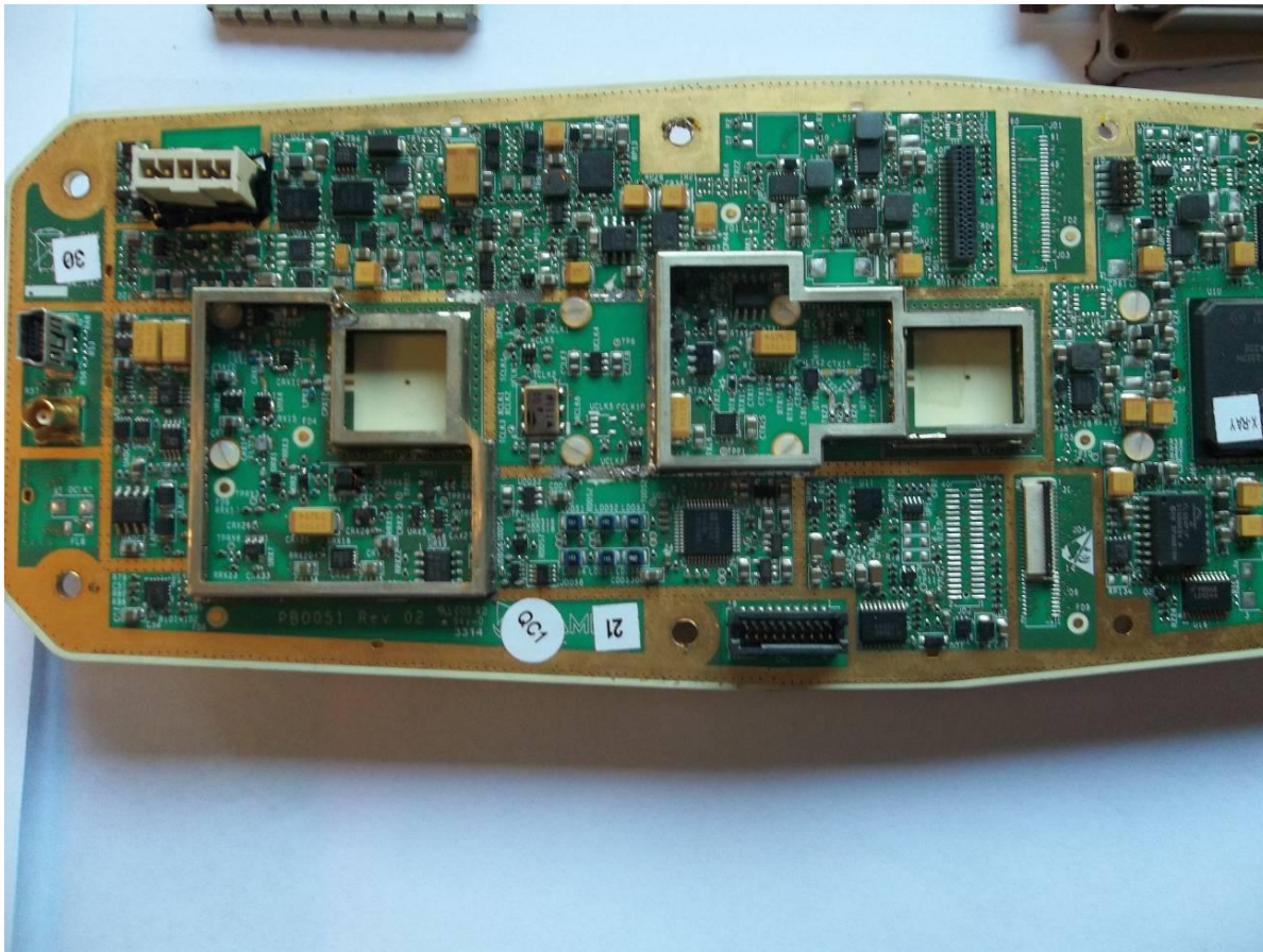
Figure 2. Component Side of PCB
