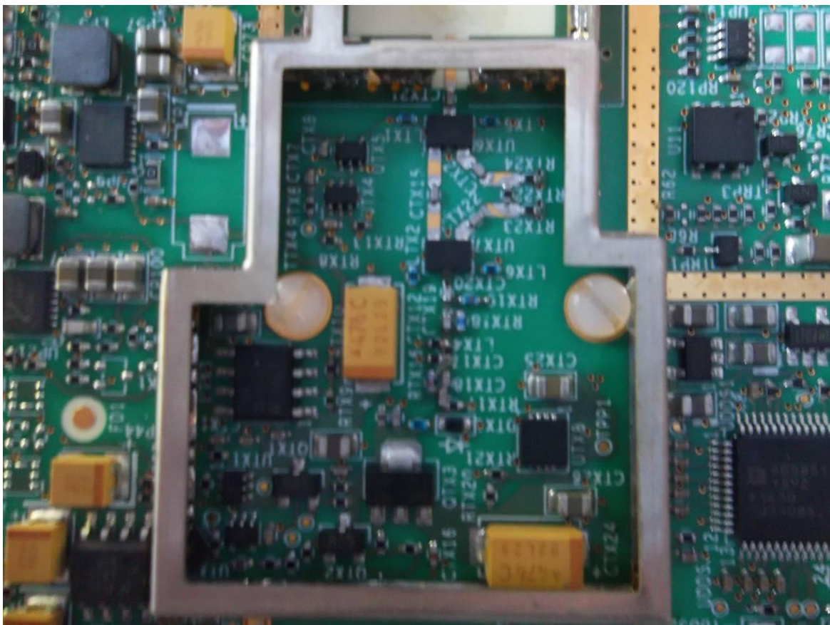
Figure 5. UWB Radio #2
