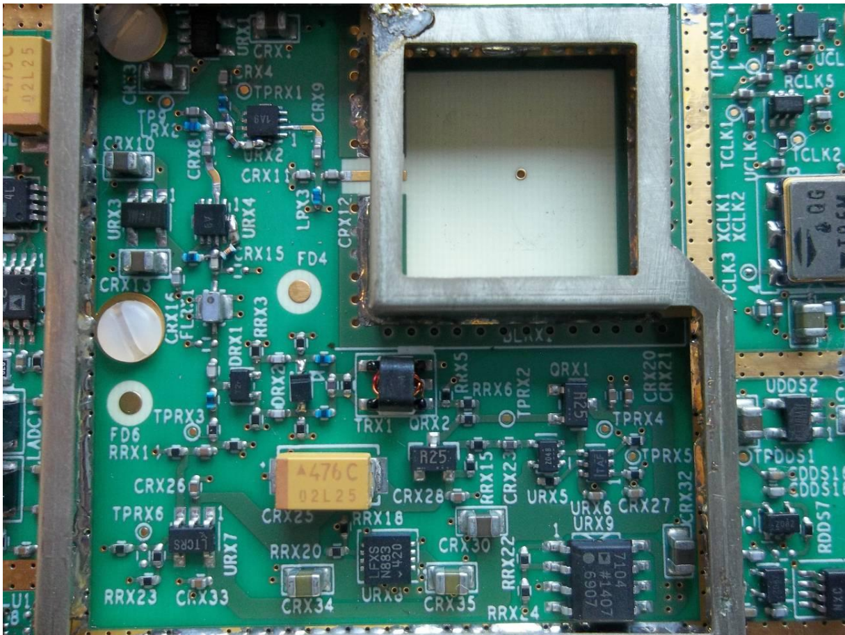
Figure 4. UWB Radio # 1
