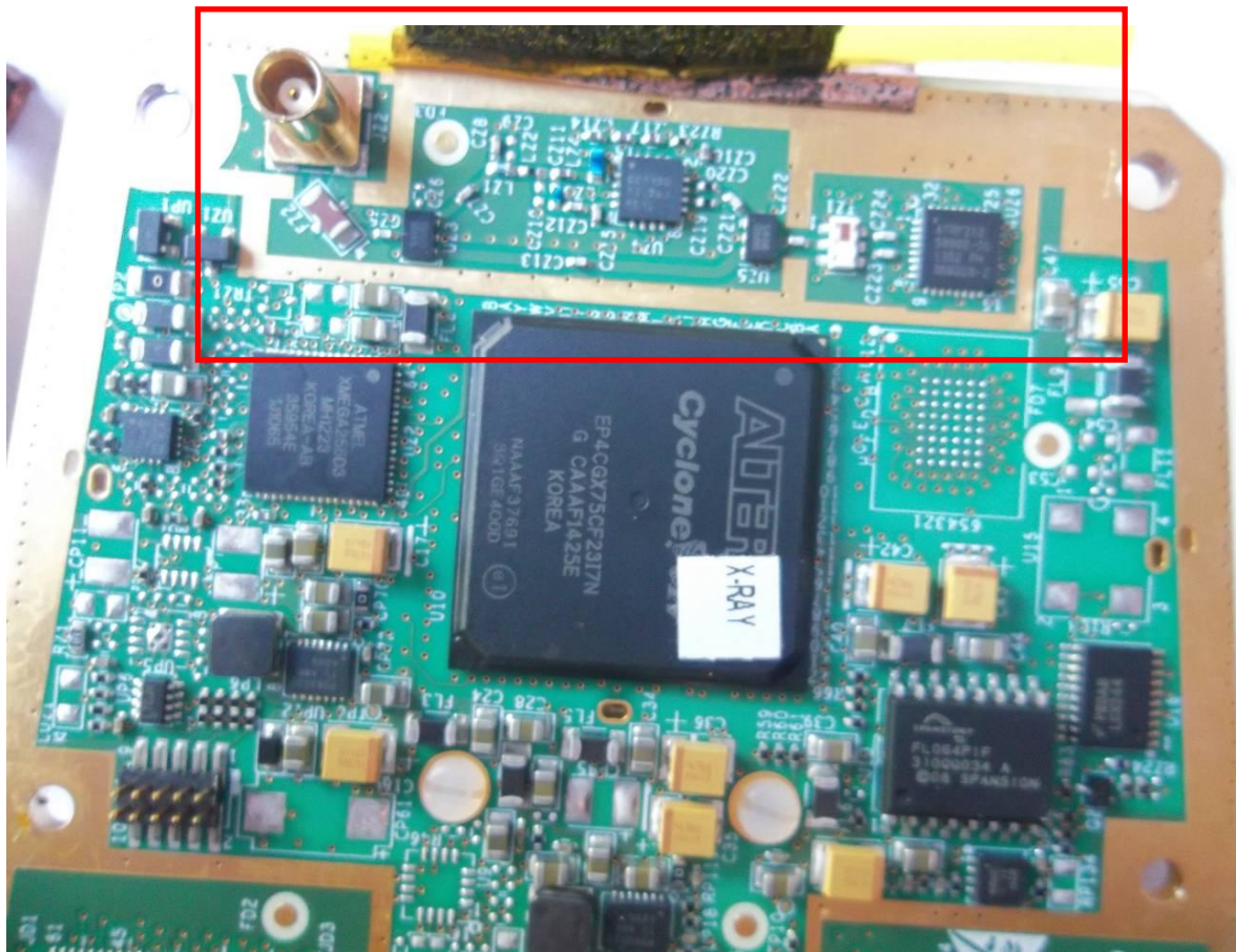
Figure 3. Zigbee Radio
