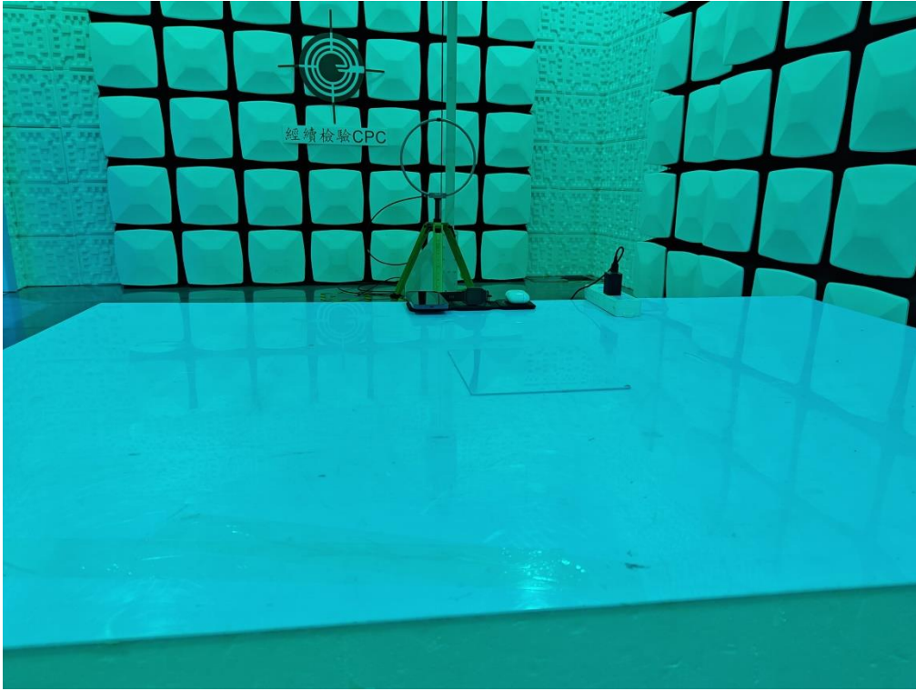
Setup Photo FCC ID: 2BBEH-W374
