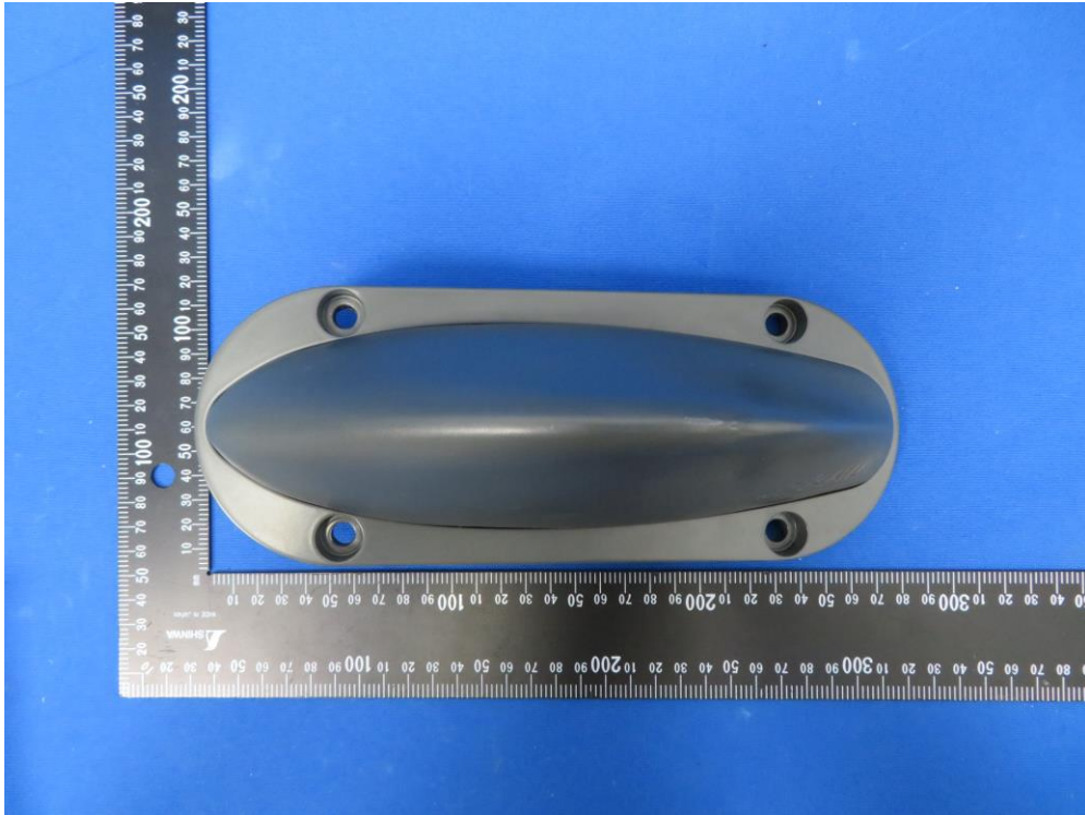
(11) EUT Photo (Antenna 3#, Gain=12dBi)
