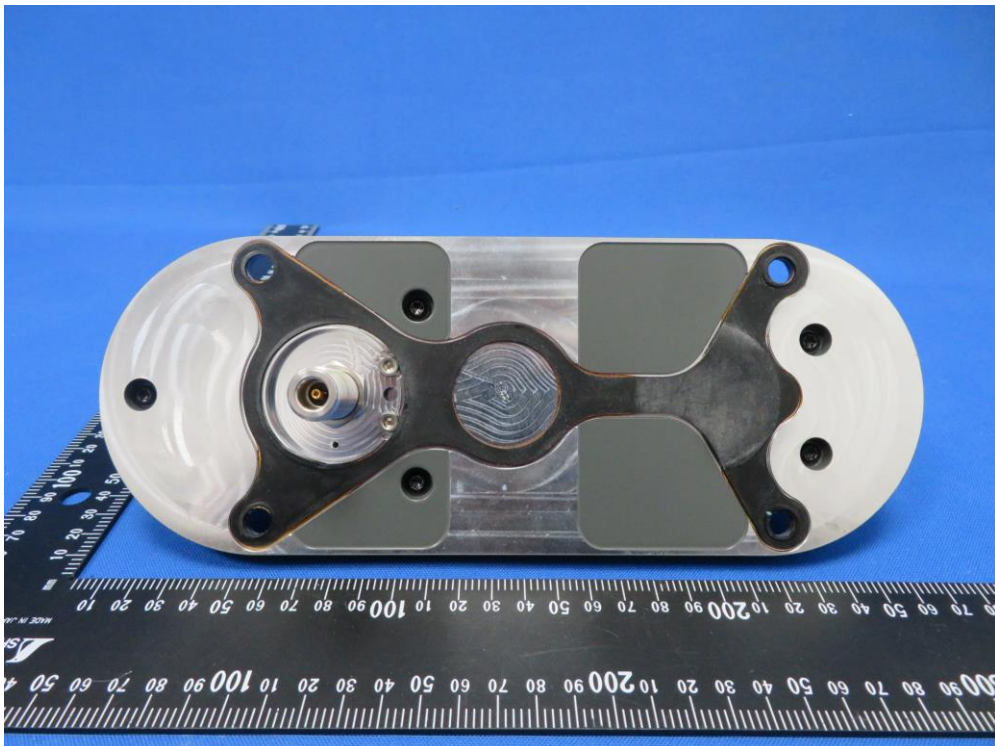
(12) EUT Photo (Antenna 3#, Gain=12dBi)
