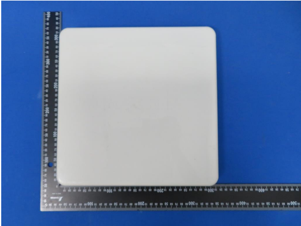
(9) EUT Photo (Antenna 2#, Gain=23dBi)
