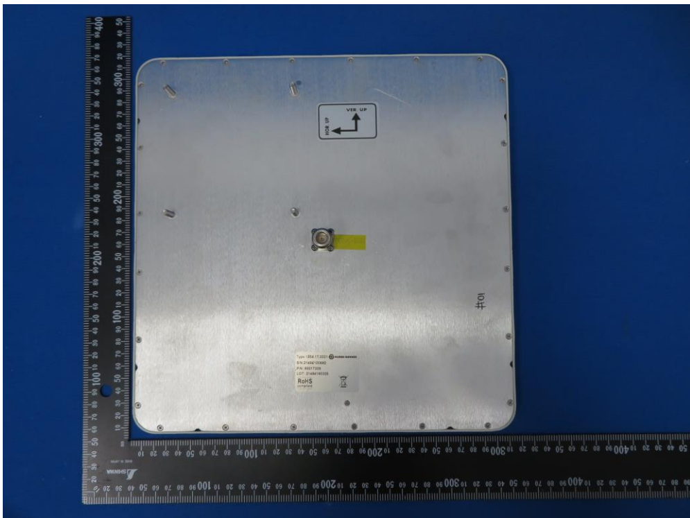
(10) EUT Photo (Antenna 2#, Gain=23dBi)
