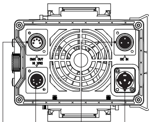
DMX OUT Port DMX IN Port Battery Input (DC) Neutrik® powerCON Power Input
