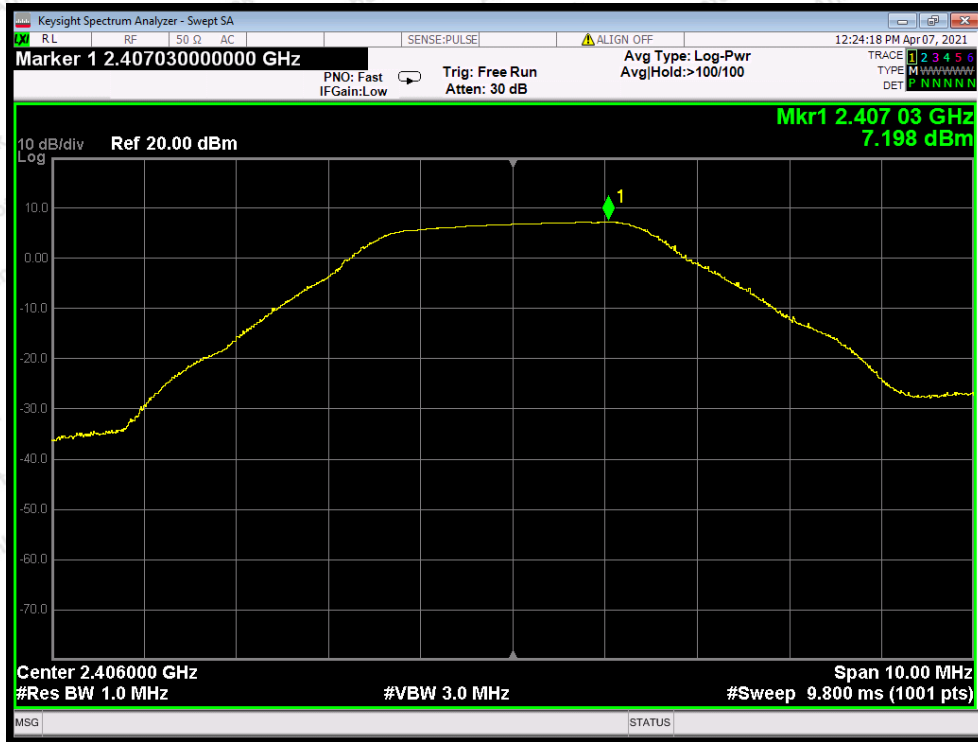
Test Mode: shaped-2FSK ---Low
