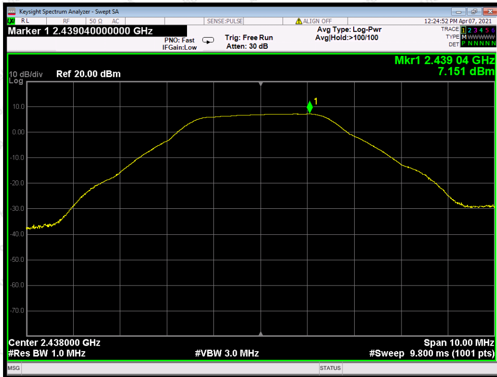
Test Mode: shaped-2FSK ---Middle
