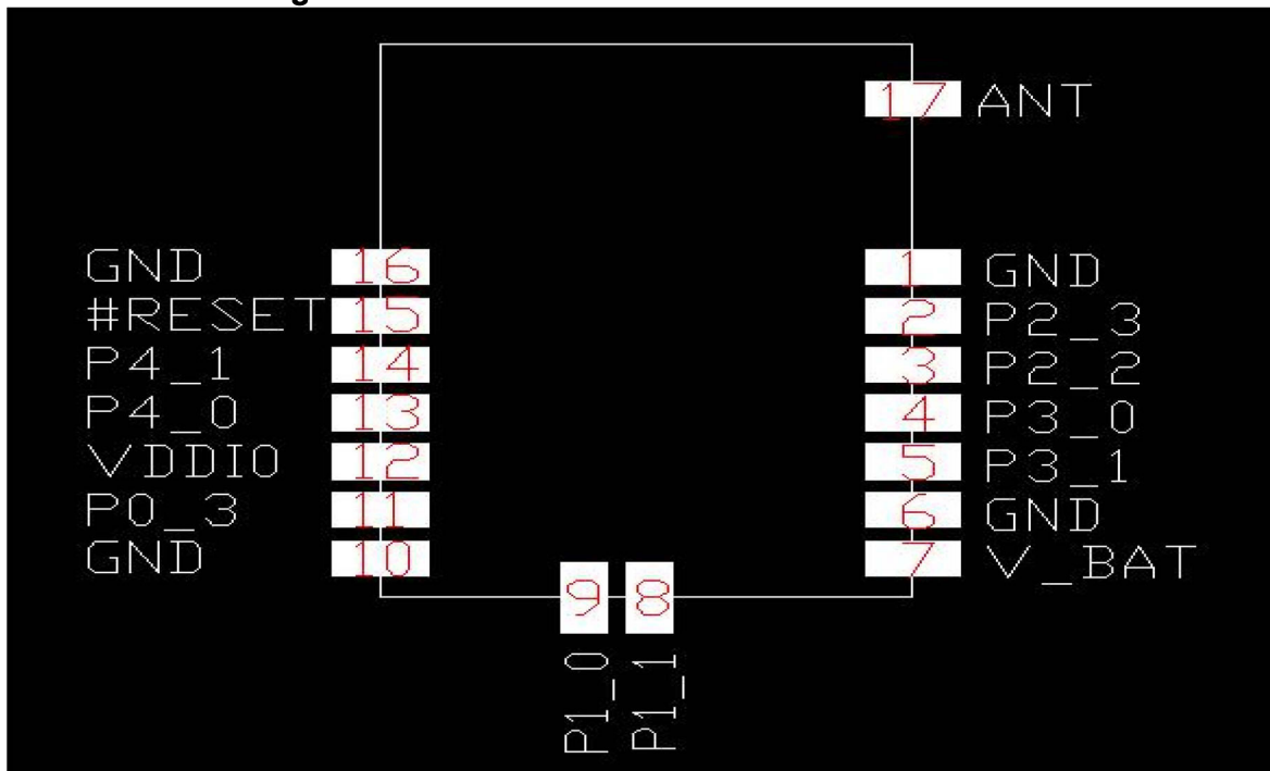
Figure 2. Pin Diagram of RB8762-17
