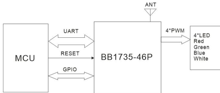
Mesh LED block diagram
