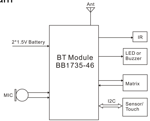
Remote control block diagram
