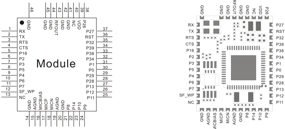
module pin assignments
