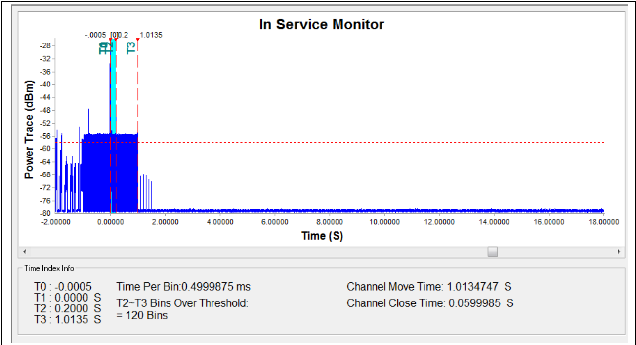
(5280MHz, 802.11n (HT20))
