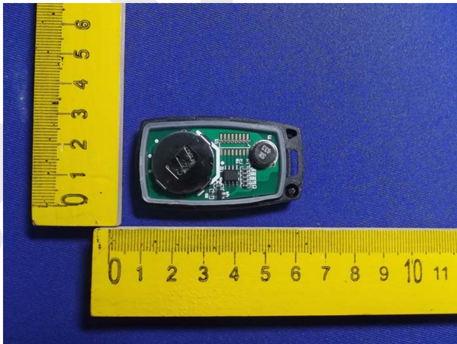
Figure 4 PCB of the EUT-Inside View
