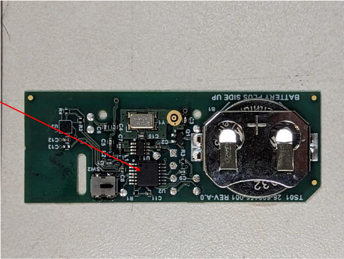
Photograph 2 – Back view of the PCB
