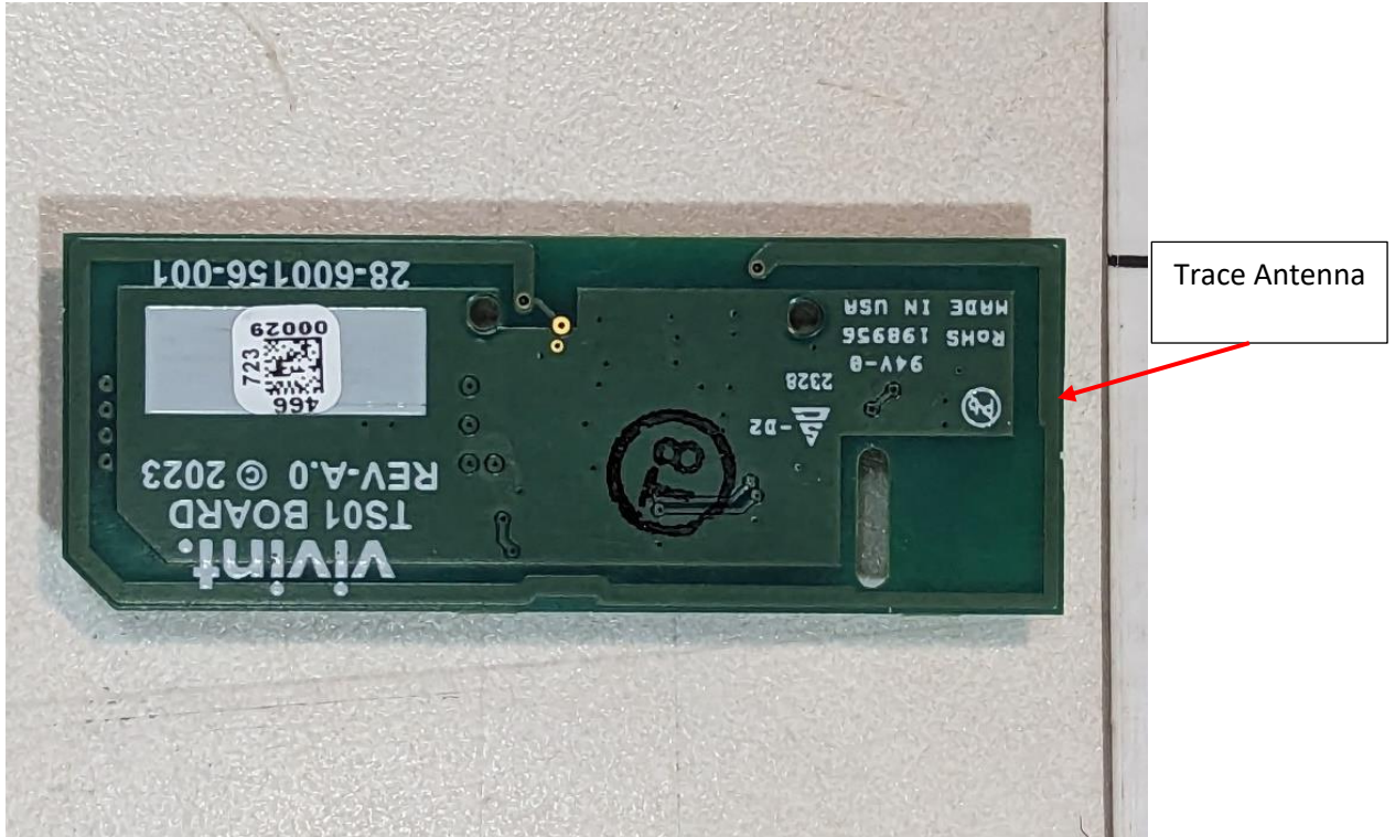
Photograph 1 –View of the Front Side of the PCB
