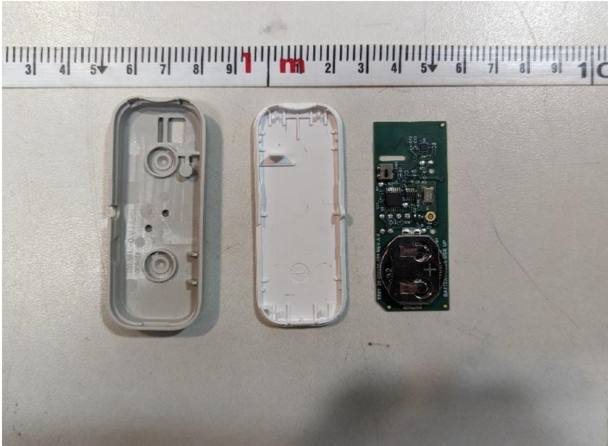
Photograph 4 – Breakout View of PCB and Housing
