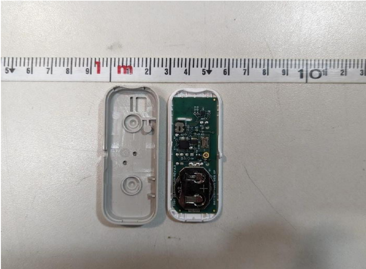
Photograph 3 – View of the PCB Mounted in the Housing
