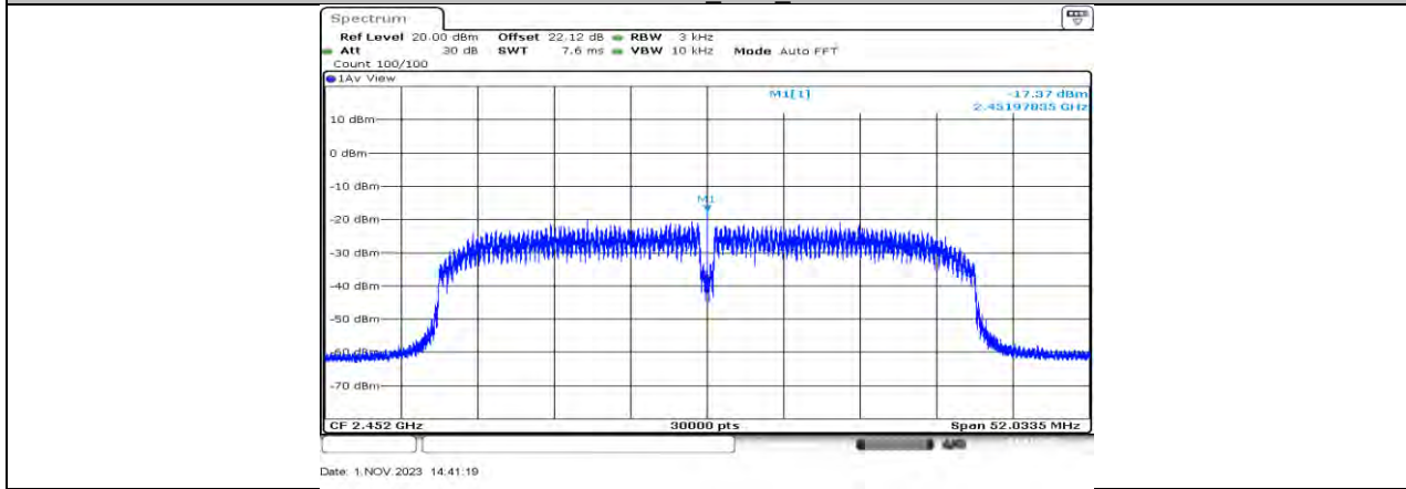
11N40SISO_Ant1_2452
