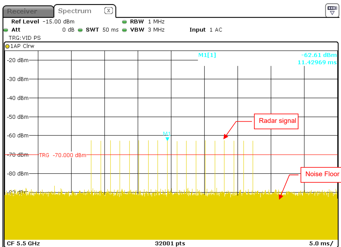
Radar Signal 0
