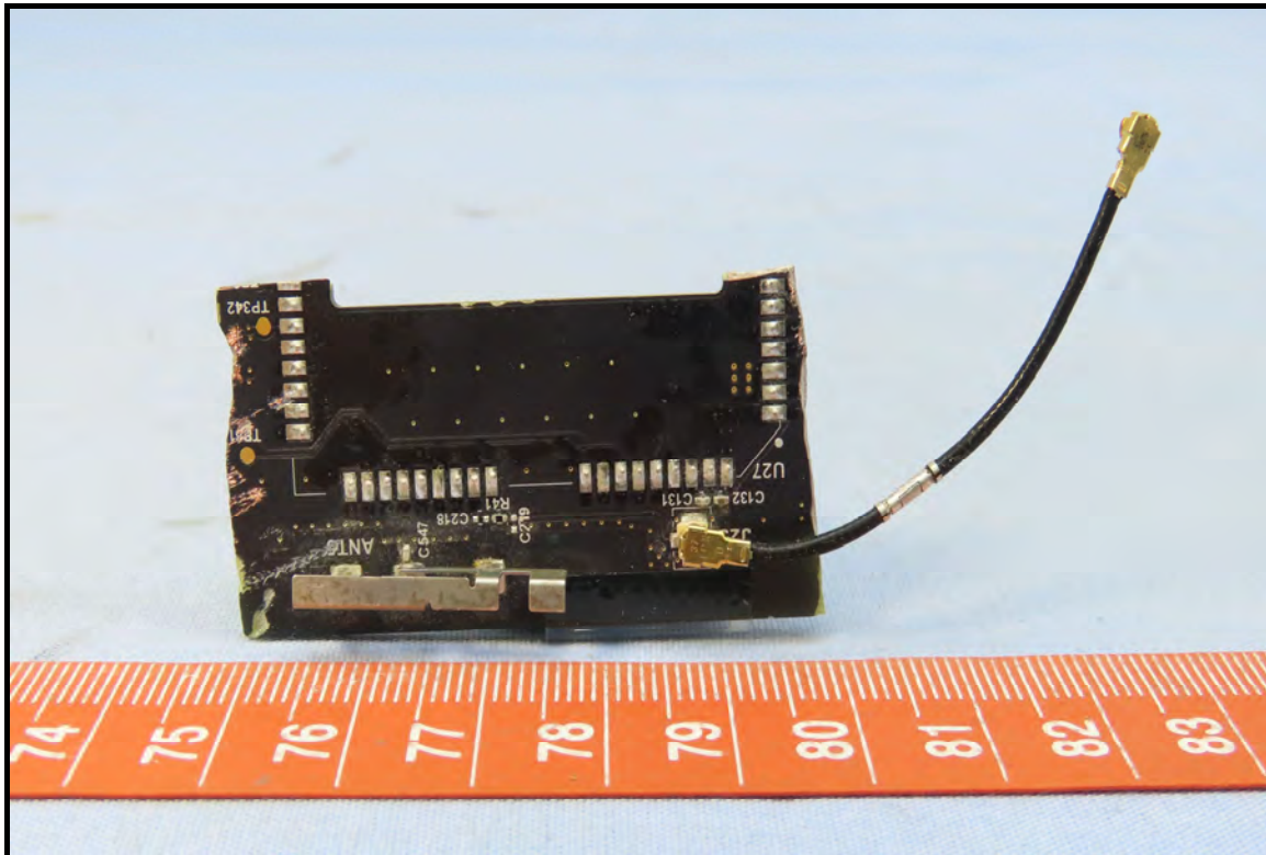
Antenna 1
