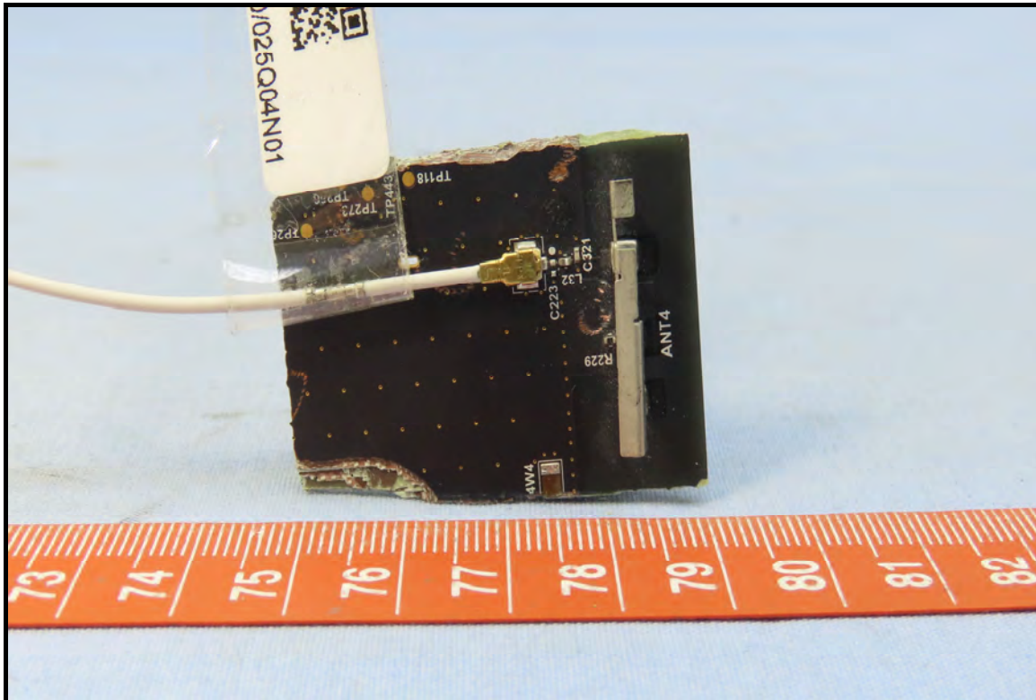
Antenna 2
