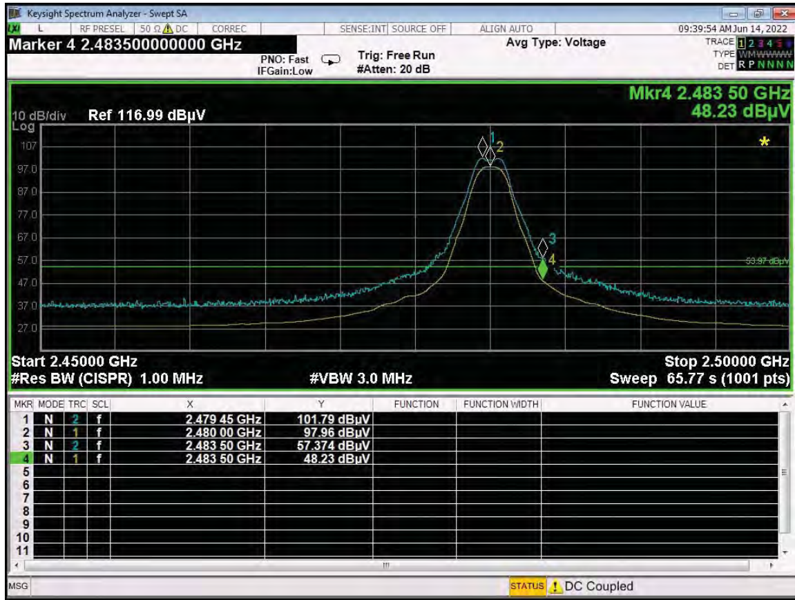
BE – 2480 MHz - Vertical - Z-Axis - Worst Case
