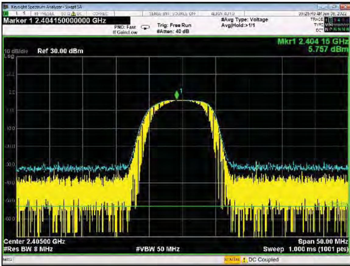
Peak Power Output - 2405 MHz
