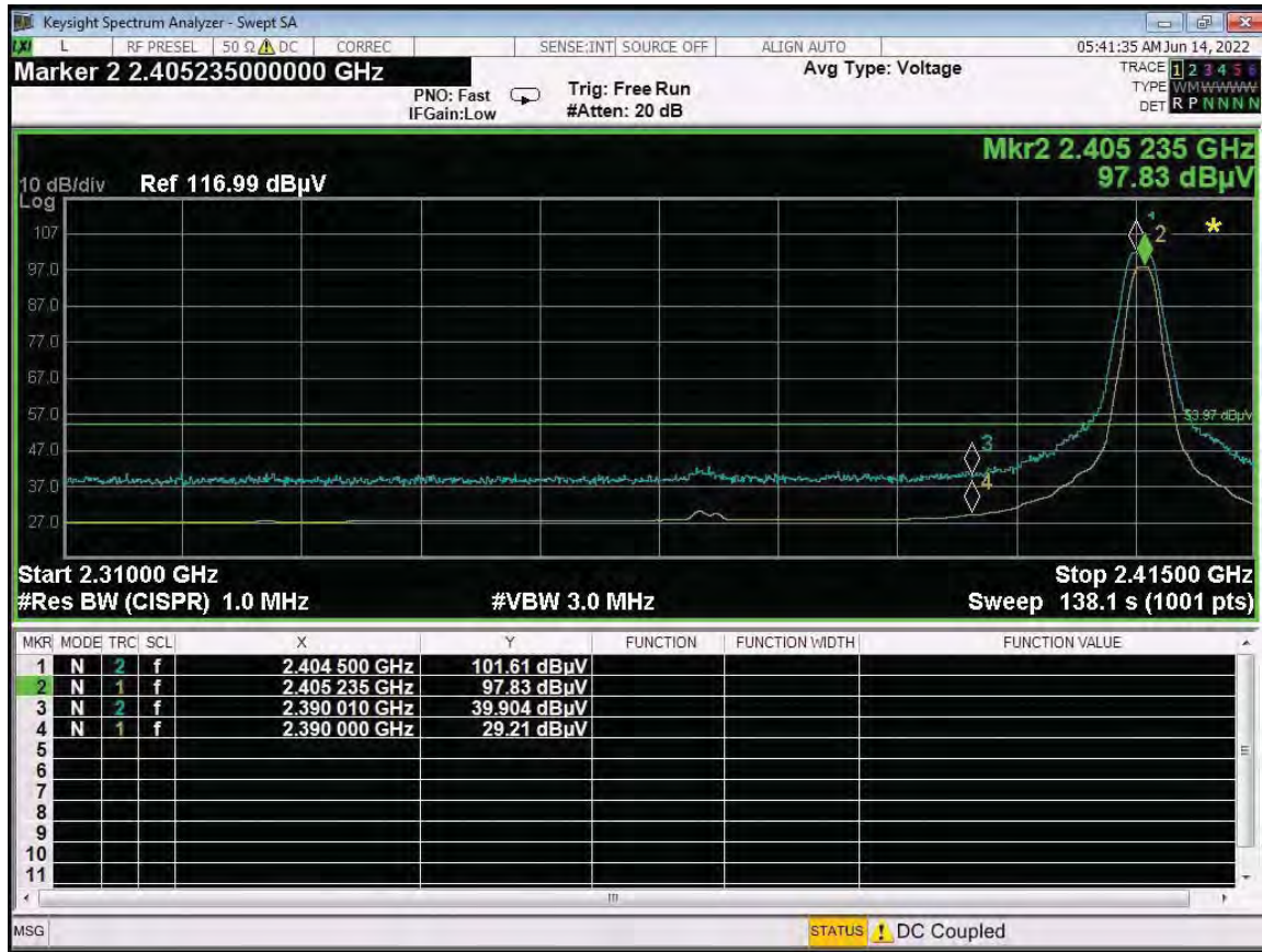
BE - 2405 MHz - Vertical - Z-Axis - Worst Case
