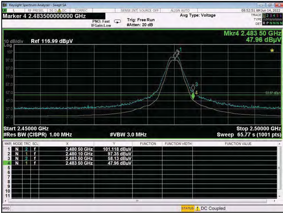
BE – 2480 MHz - Horizontal - Y-Axis - Worst Case
