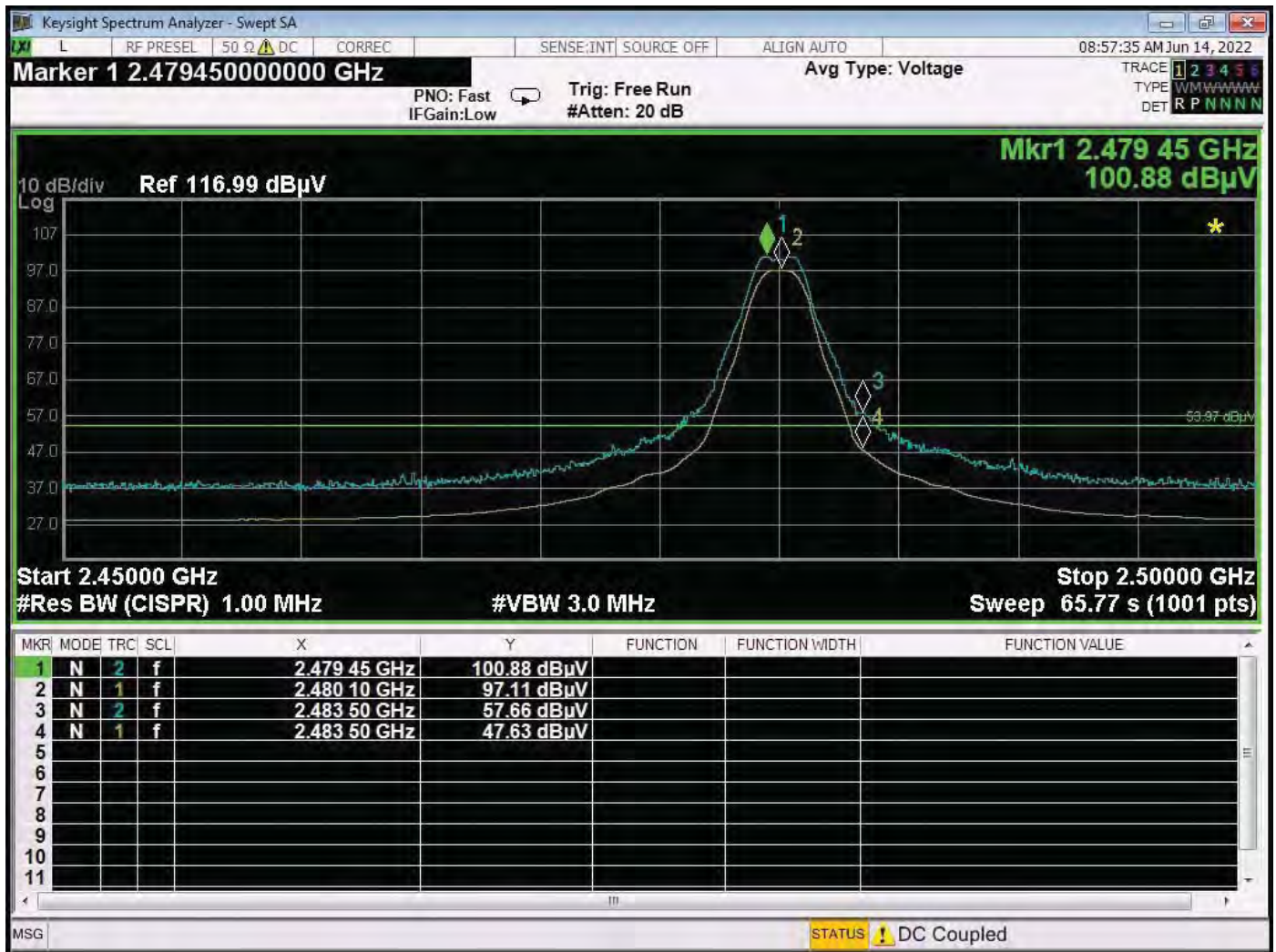
BE – 2480 MHz - Vertical - Z-Axis - Worst Case
