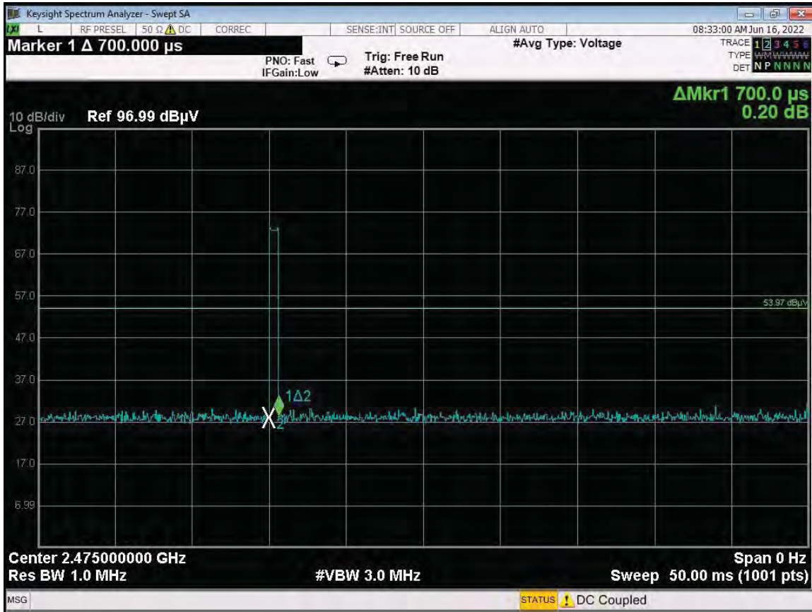
Time of One Pulse 700 μs
