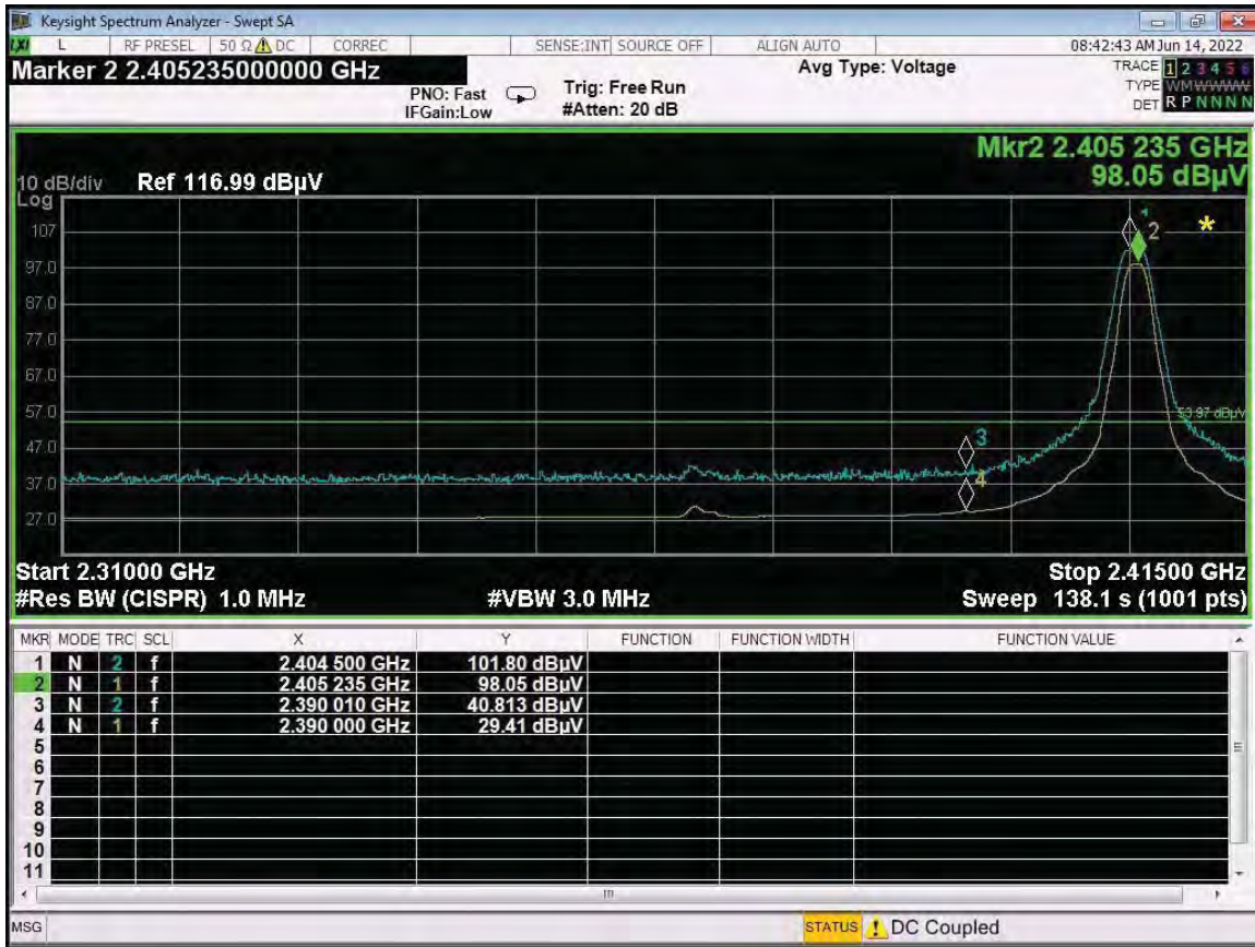
BE - 2405 MHz - Horizontal - Y-Axis - Worst Case
