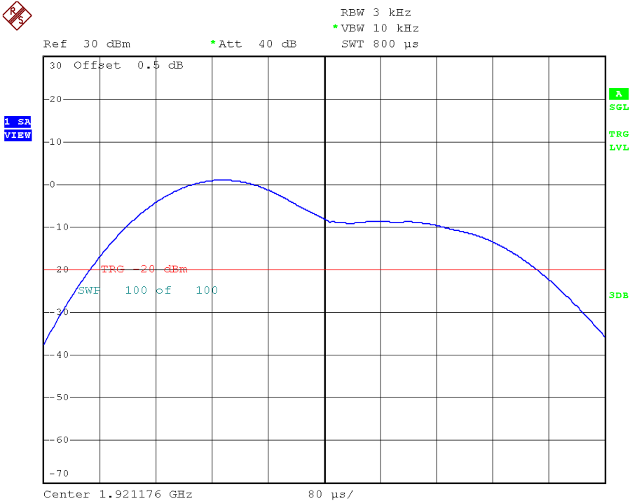
Smart Screen, Lowest channel, Traffic carrier
