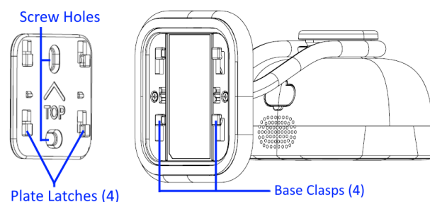
Wall Mount Back Plate and Camera Base (bottom view) —
