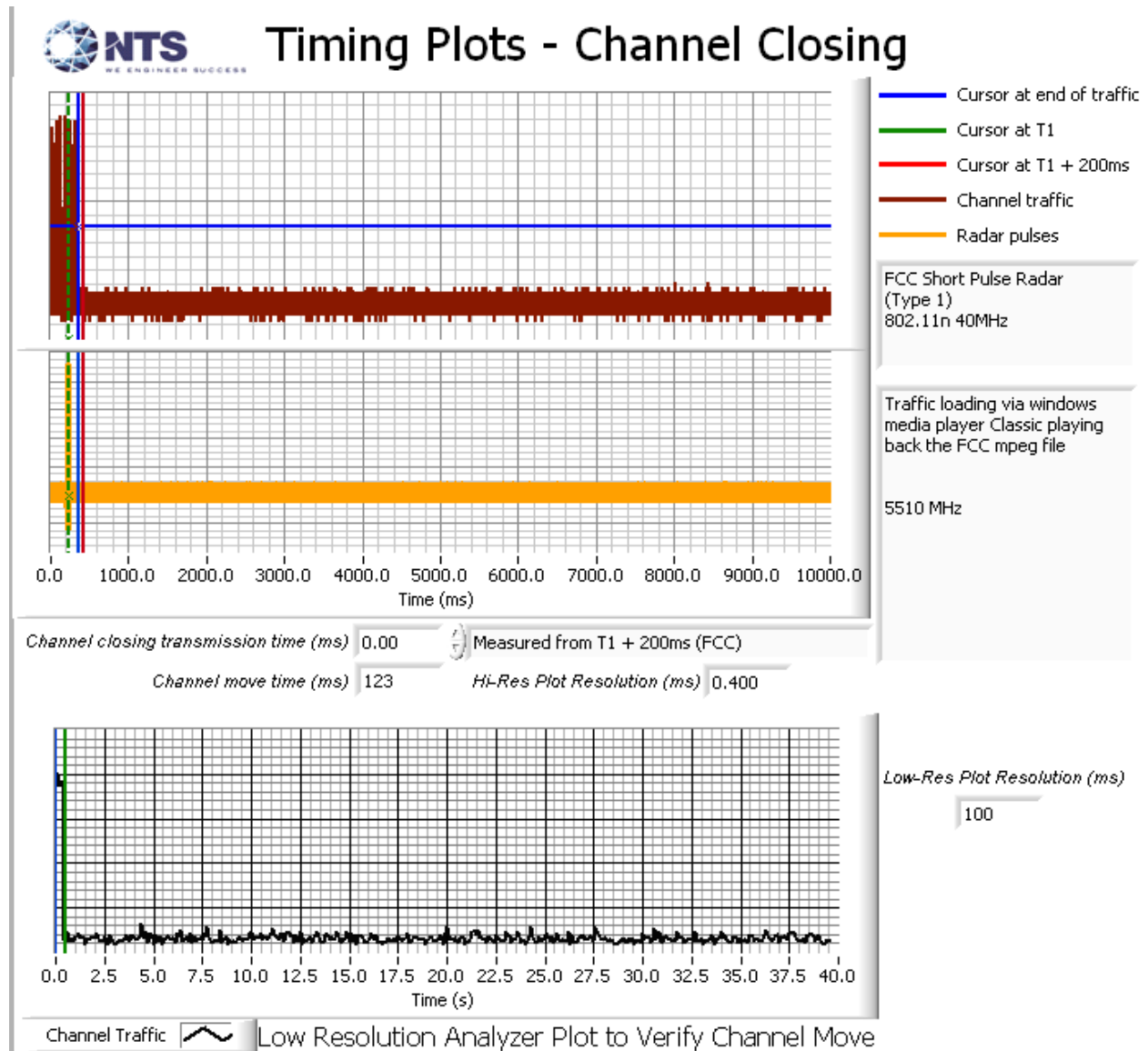
Figure 9 Channel Closing Time and Channel Move Time – 40 second plot
