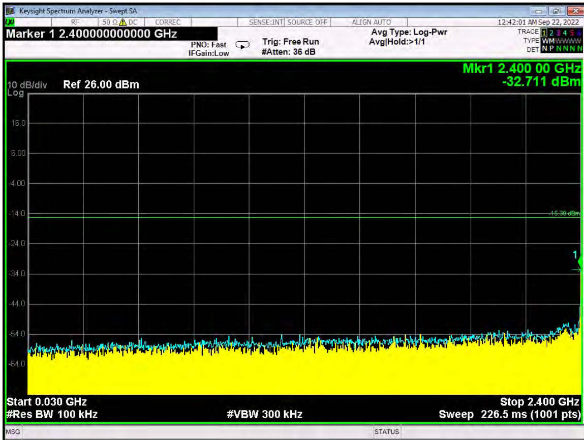
RF Antenna Conducted Test – ANT 1 – Low Channel – 30 MHz to 2.4 GHz
