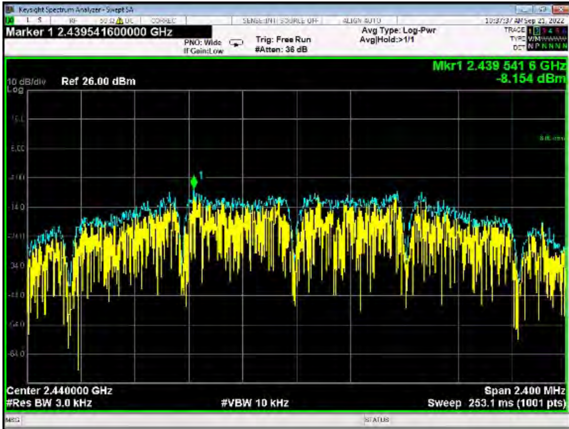
Special Density Output - ANT 0 - 2440 MHz
