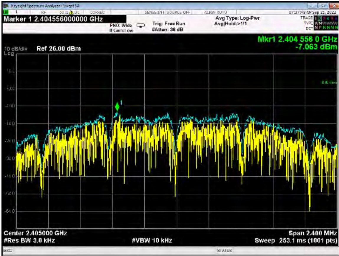
Special Density Output - ANT 0 - 2405 MHz
