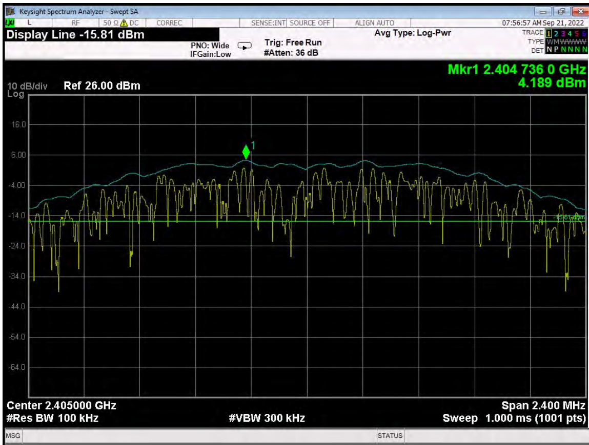
RF Antenna Conducted Test – ANT 0 – Low Channel – Reference Level
