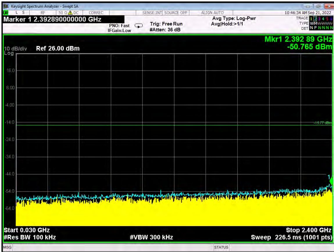
RF Antenna Conducted Test – ANT 0 – Mid Channel – 30 MHz to 2.4 GHz
