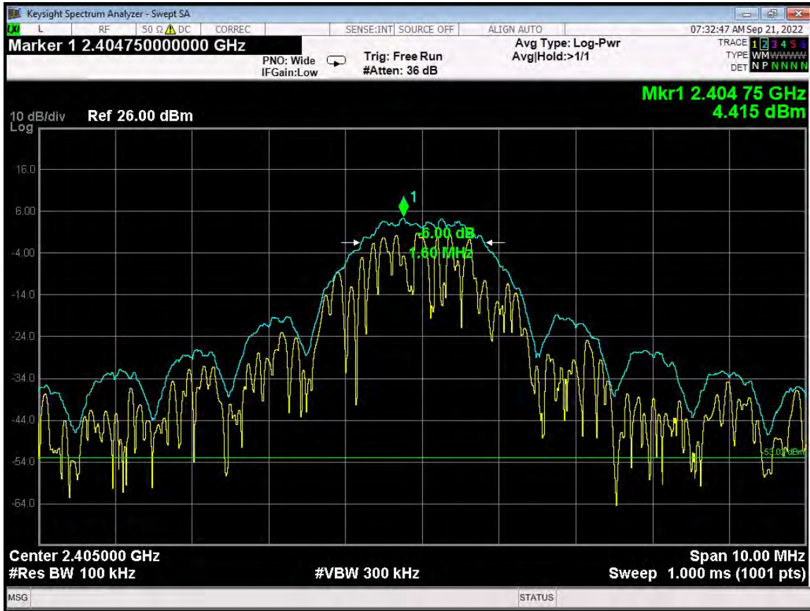
Bandwidth 6 dB - ANT 0 - 2405 MHz
