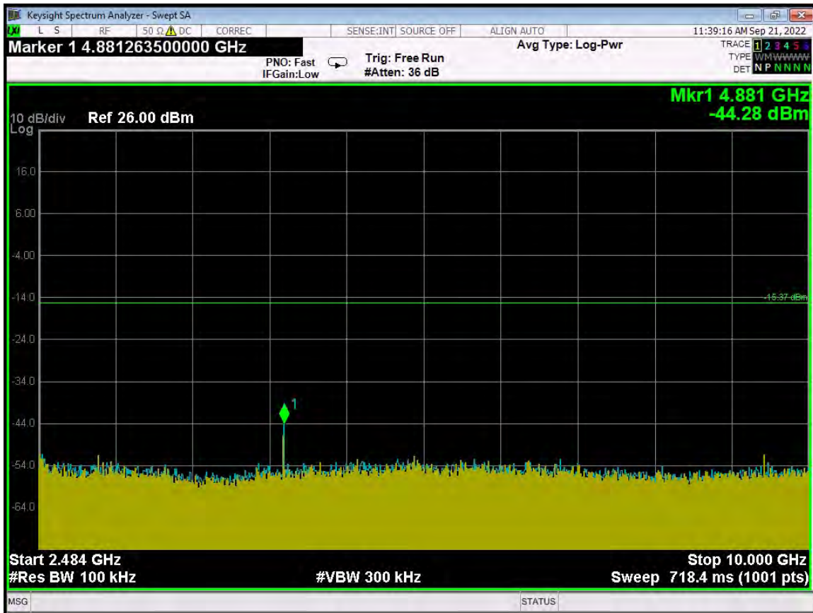
RF Antenna Conducted Test – ANT 1 – Mid Channel – 2483.5 MHz to 10 GHz
