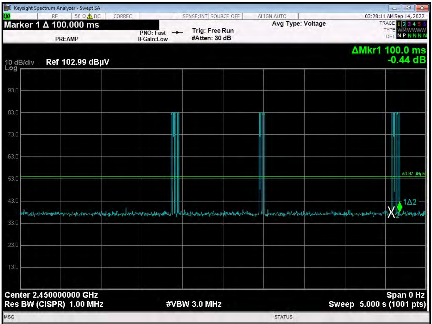
The pulse train only once per 100 ms – Light off Mode Worst Case
