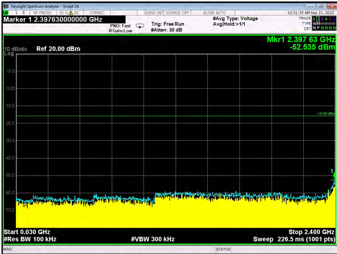
RF Antenna Conducted Test – ANT 0 – High Channel – 30 MHz to 2.4 GHz
