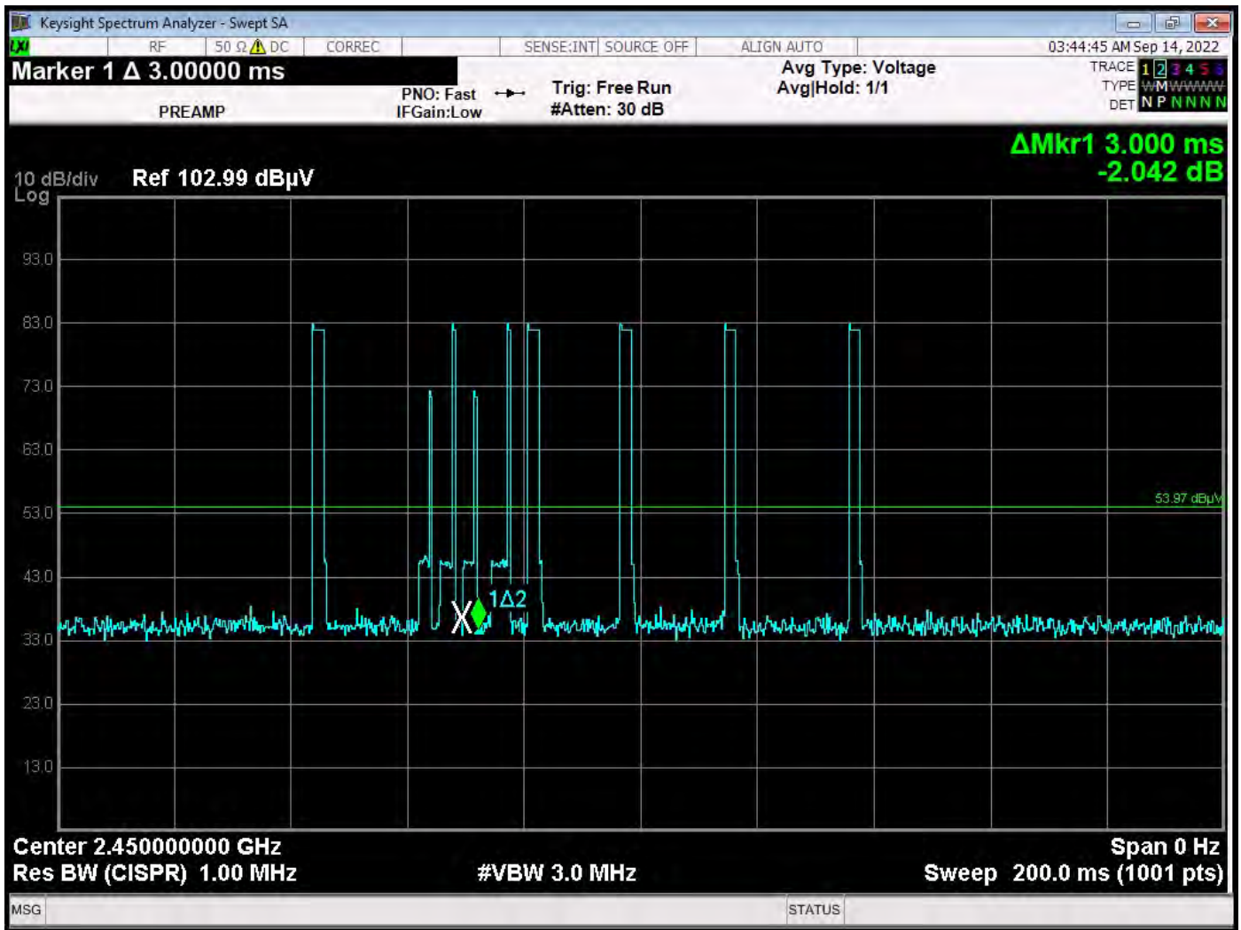
Time of Fourth Pulse = 3.0 ms – Light off Mode Worst Case
