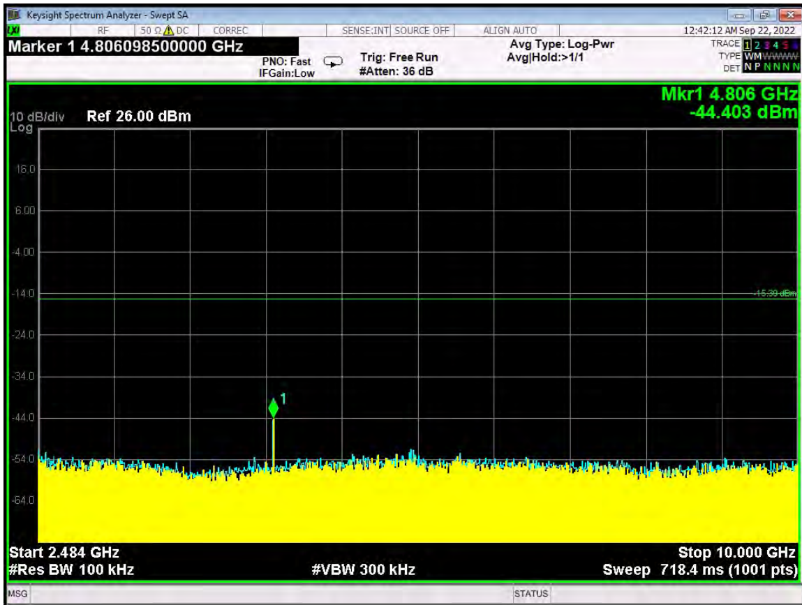
RF Antenna Conducted Test – ANT 1 – Low Channel – 2483.5 MHz to 10 GHz
