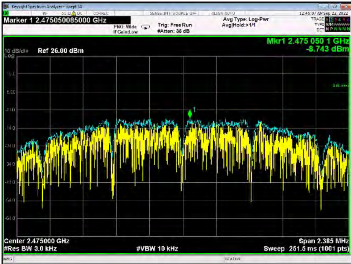
Special Density Output - ANT 1 - 2475 MHz
