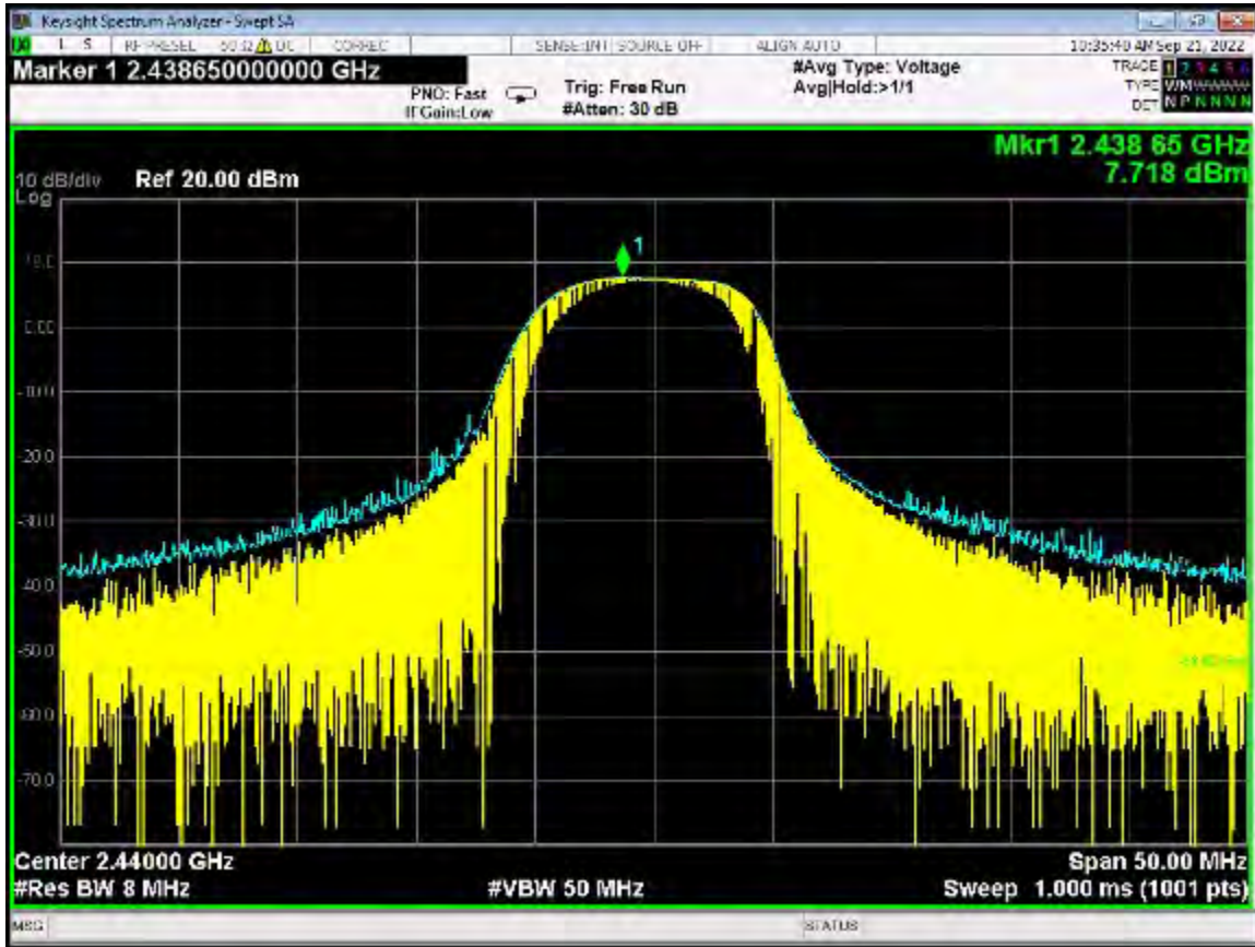
Peak Power Output – ANT 0 – 2440 MHz
