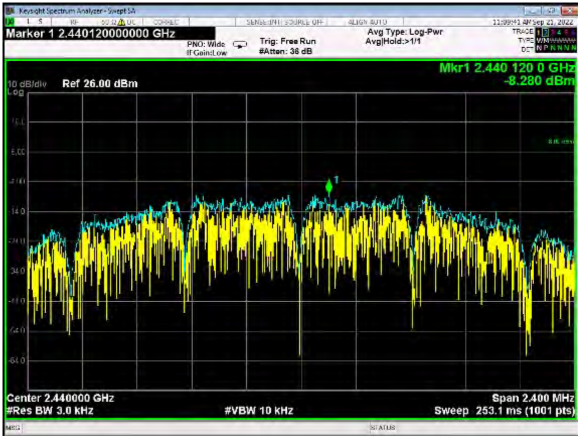
Special Density Output - ANT 1 - 2440 MHz
