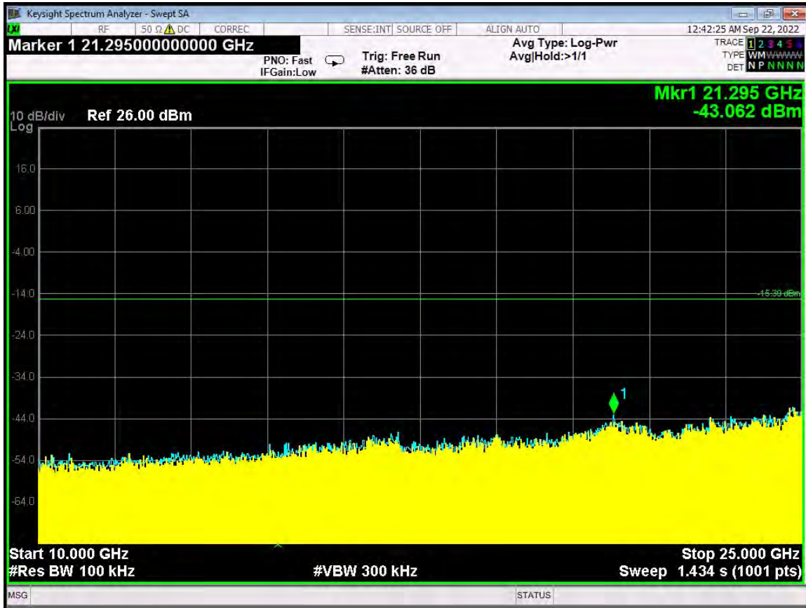
RF Antenna Conducted Test – ANT 1 – Low Channel – 10 GHz to 25 GHz
