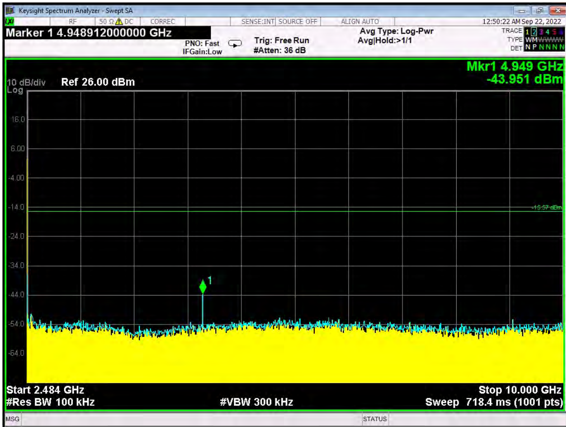
RF Antenna Conducted Test – ANT 1 – High Channel – 2483.5 MHz to 10 GHz
