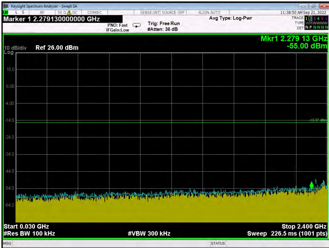
RF Antenna Conducted Test – ANT 1 – Mid Channel – 30 MHz to 2.4 GHz
