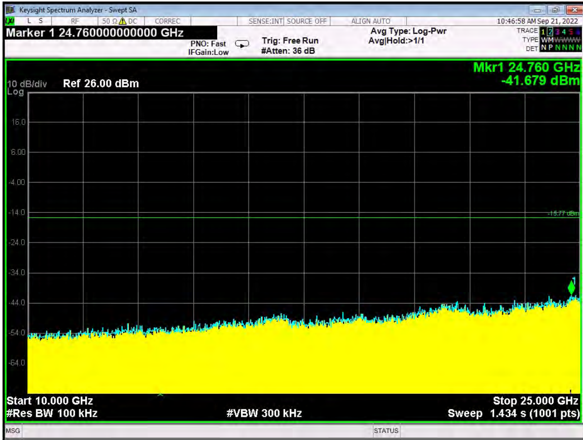
RF Antenna Conducted Test – ANT 0 – Mid Channel – 10 GHz to 25 GHz
