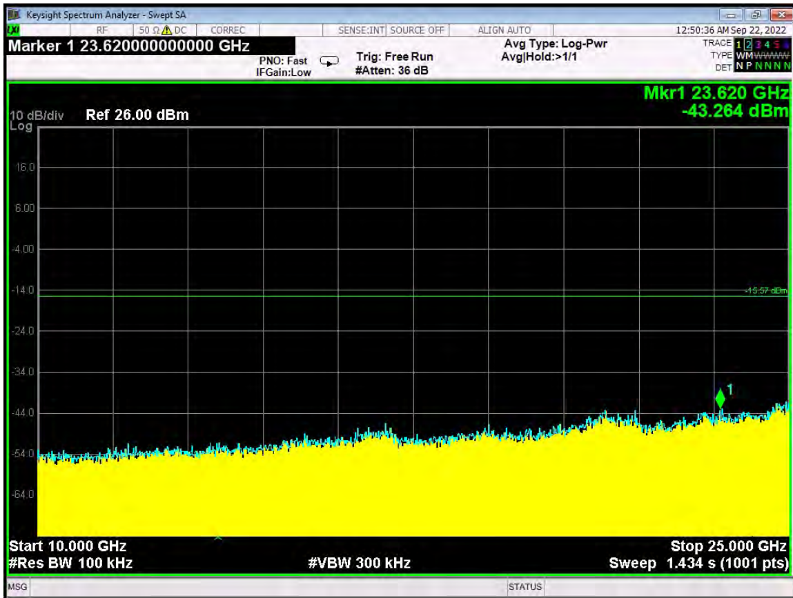
RF Antenna Conducted Test – ANT 1 – High Channel – 10 GHz to 25 GHz
