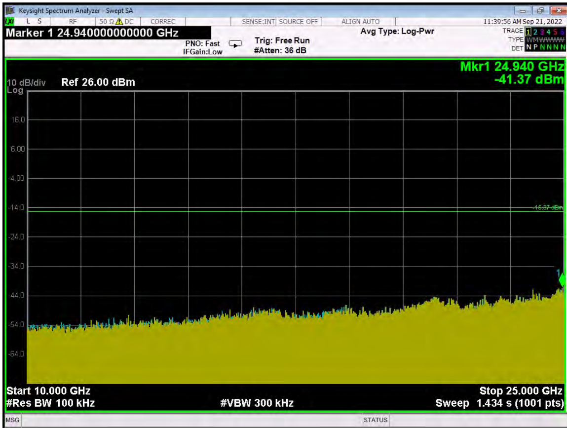
RF Antenna Conducted Test – ANT 1 – Mid Channel – 10 GHz to 25 GHz
