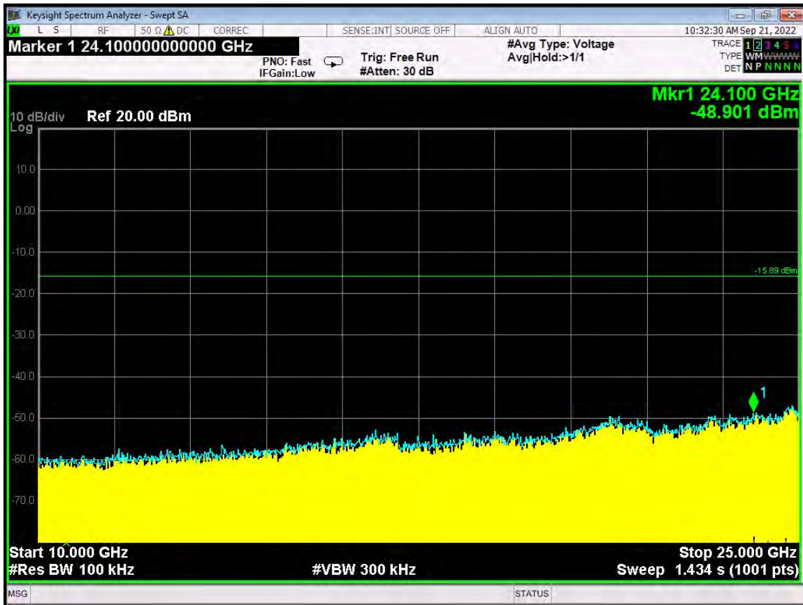
RF Antenna Conducted Test – ANT 0 – High Channel – 10 GHz to 25 GHz
