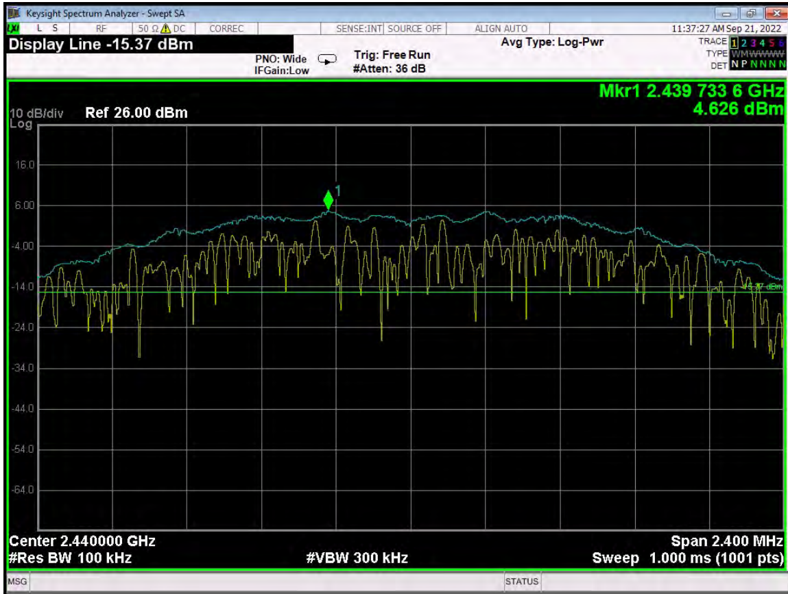
RF Antenna Conducted Test – ANT 1 – Mid Channel – Reference Level
