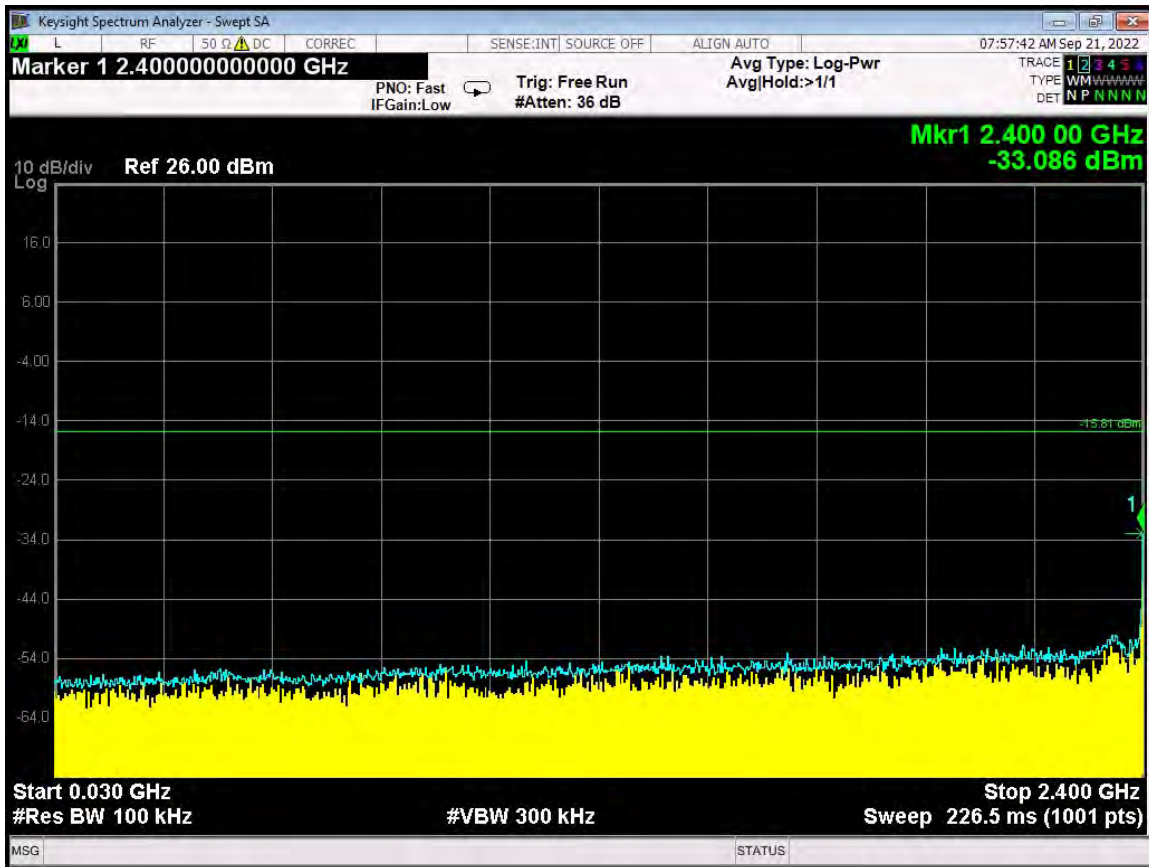
RF Antenna Conducted Test – ANT 0 – Low Channel – 30 MHz to 2.4 GHz
