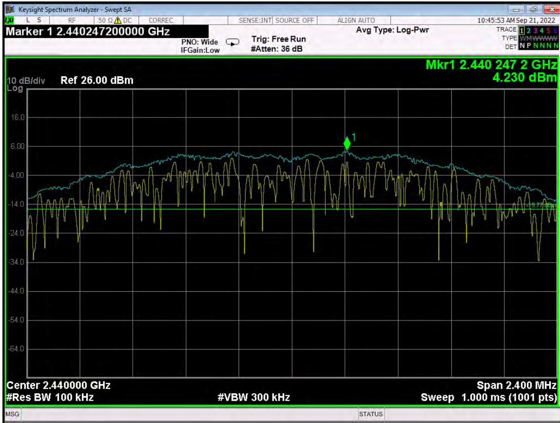
RF Antenna Conducted Test – ANT 0 – Mid Channel – Reference Level
