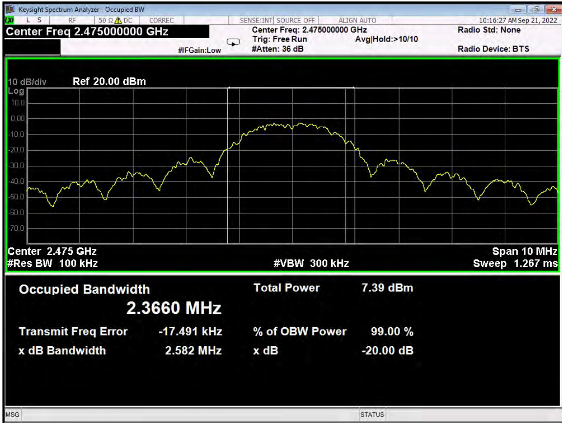
99% Bandwidth - ANT 0 - 2475 MHz
