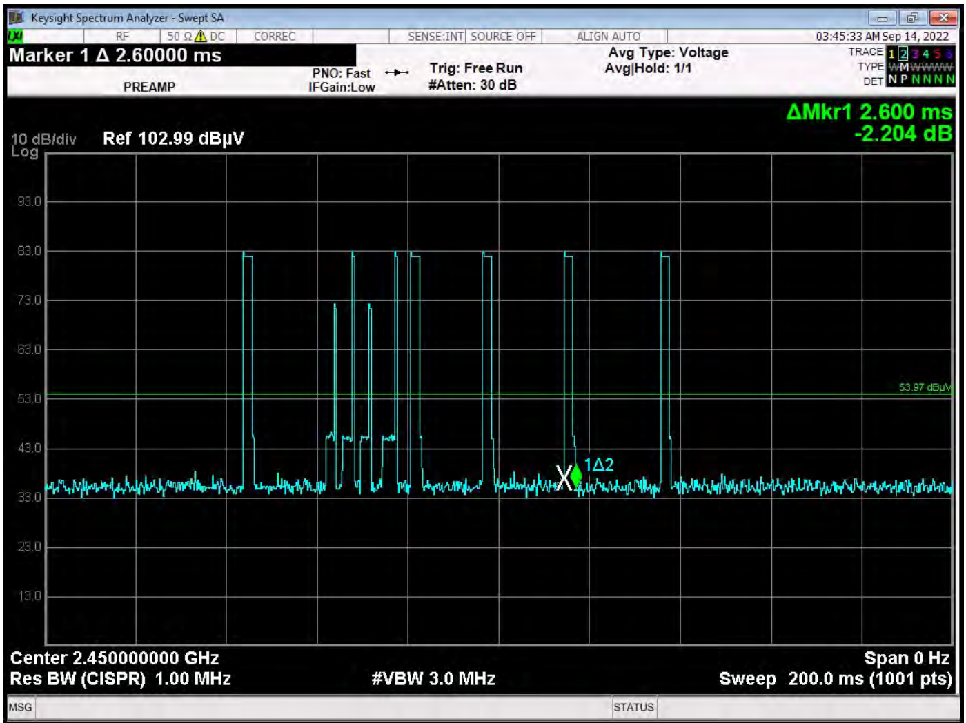
Time on Eighth Pulse = 2.6 ms – Light off Mode Worst Case
