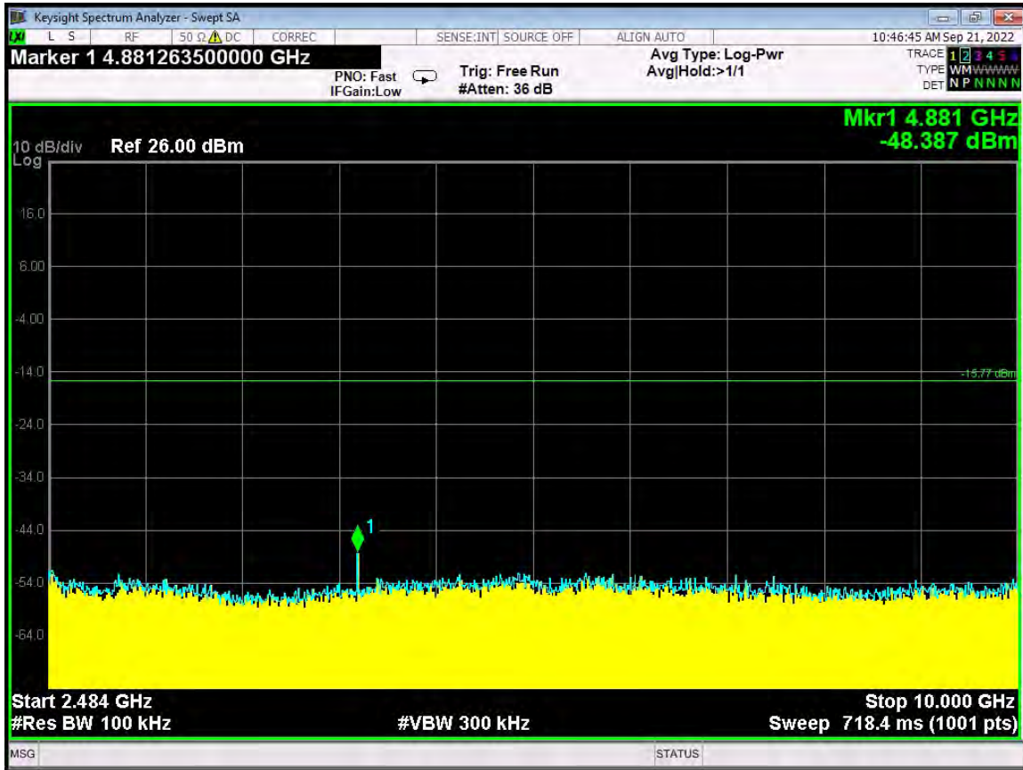
RF Antenna Conducted Test – ANT 0 – Mid Channel – 2483.5 MHz to 10 GHz
