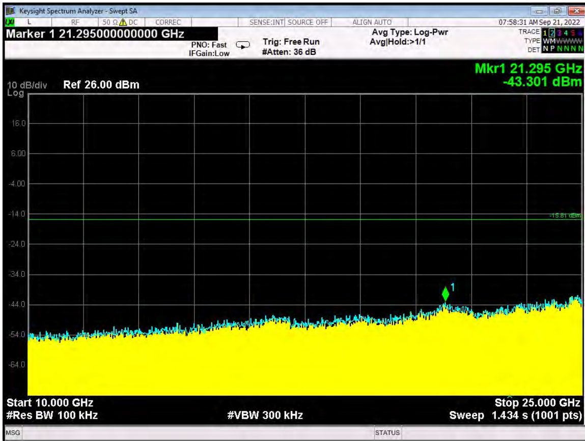
RF Antenna Conducted Test – ANT 0 – Low Channel – 10 GHz to 25 GHz
