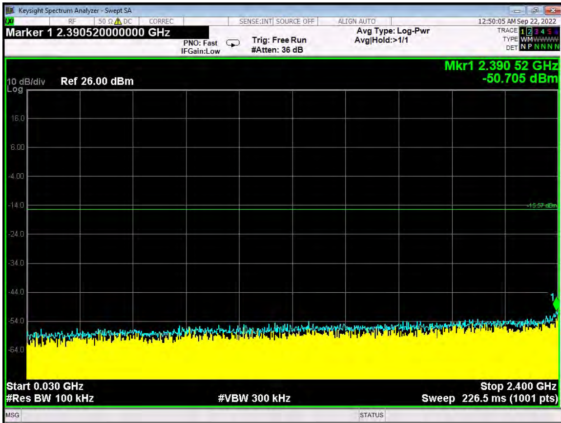
RF Antenna Conducted Test – ANT 1 – High Channel – 30 MHz to 2.4 GHz
