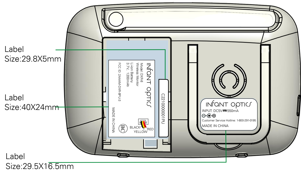
DXR-8 Date code and serial no. label
