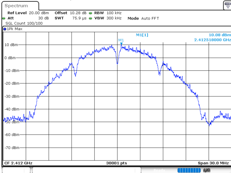
Tx. Spurious NVNT b 2412MHz Ant 4 Emission
