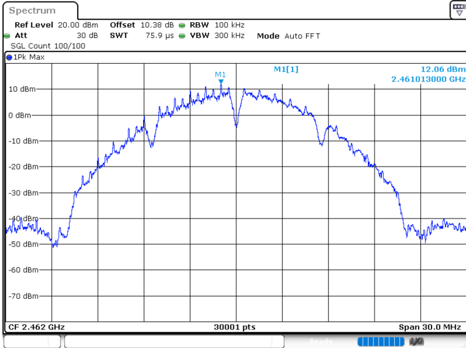
Tx. Spurious NVNT b 2462MHz Ant 4 Ref
