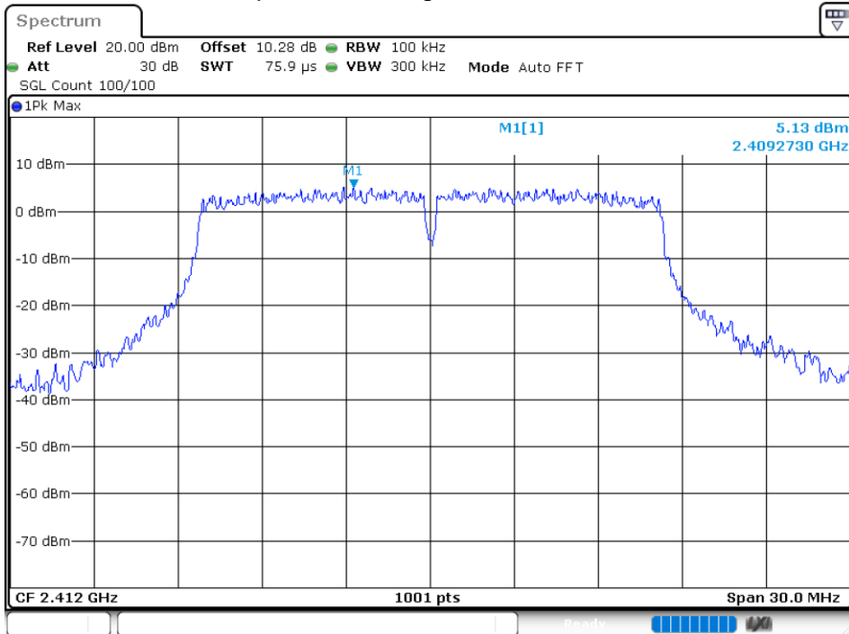
Tx. Spurious NVNT g 2412MHz Ant 4 Emission
