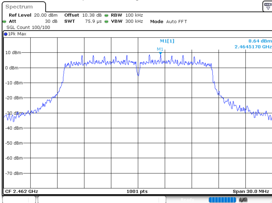
Tx. Spurious NVNT g 2462MHz Ant 4 Emission
