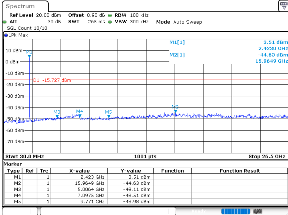
Tx. Spurious NVNT n20 2437MHz Ant 3 Ref
