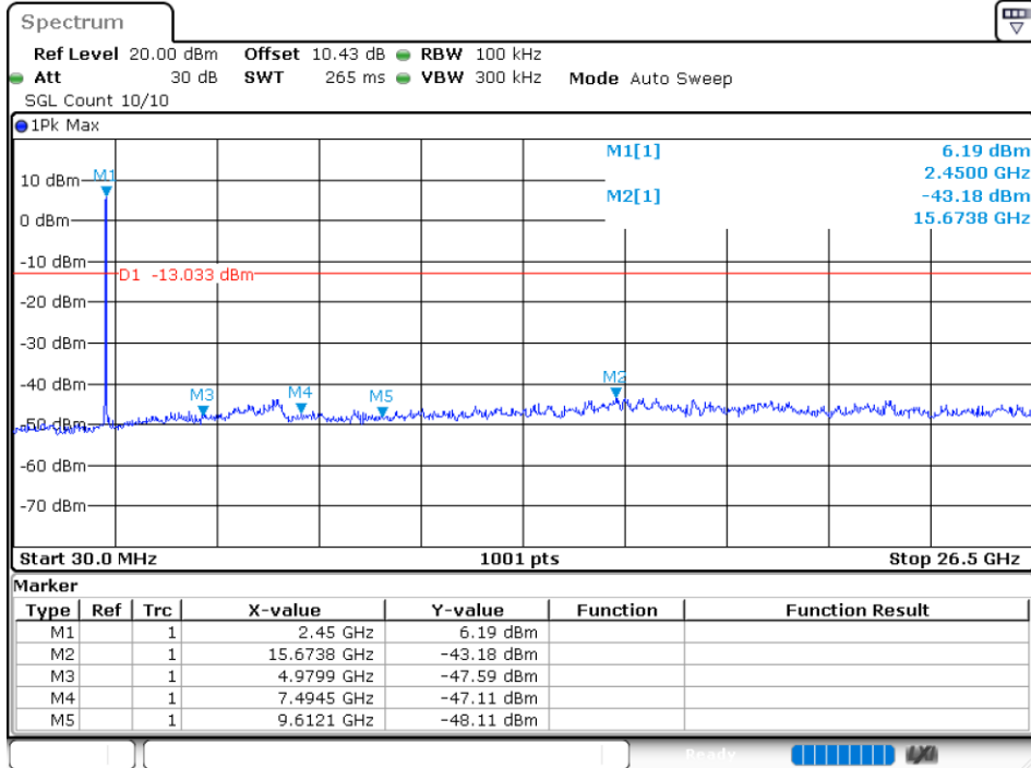
Tx. Spurious NVNT g 2462MHz Ant 4 Ref
