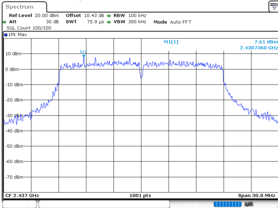
Tx. Spurious NVNT n20 2437MHz Ant 4 Emission
