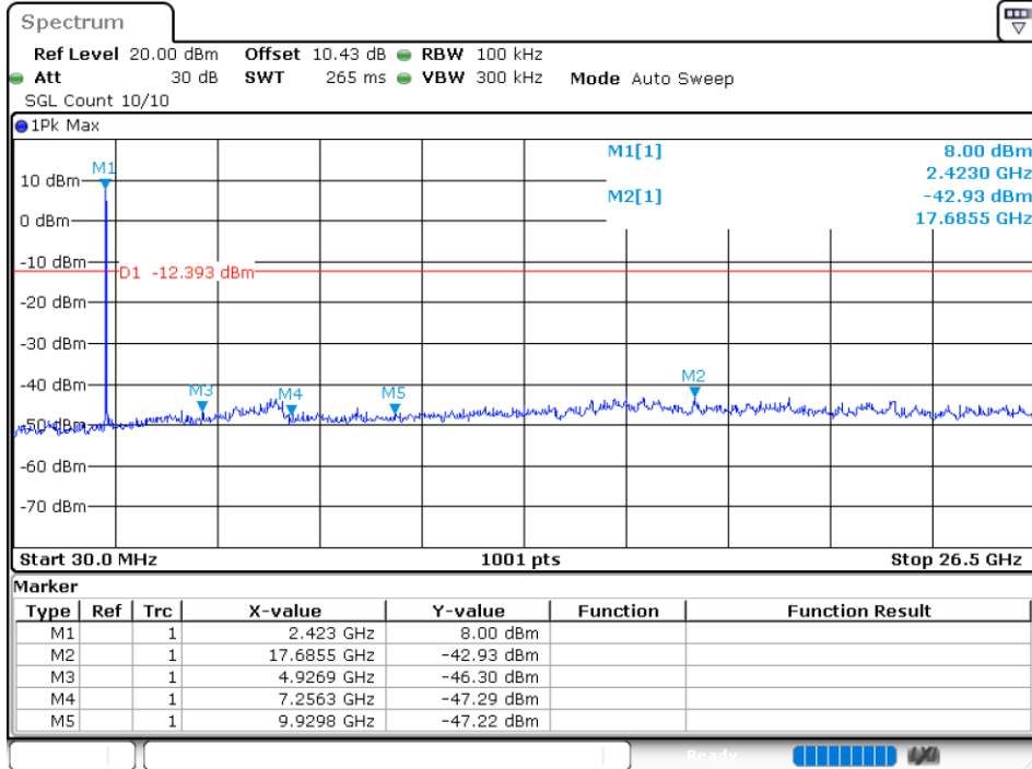
Tx. Spurious NVNT n20 2462MHz Ant 4 Ref
