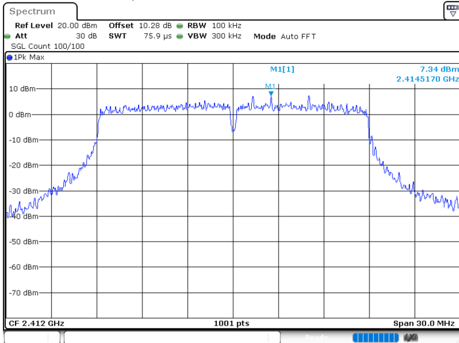
Tx. Spurious NVNT n20 2412MHz Ant 4 Emission
