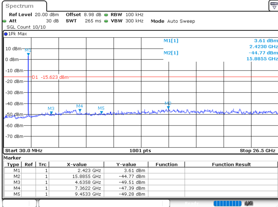
Tx. Spurious NVNT g 2437MHz Ant 3 Ref
