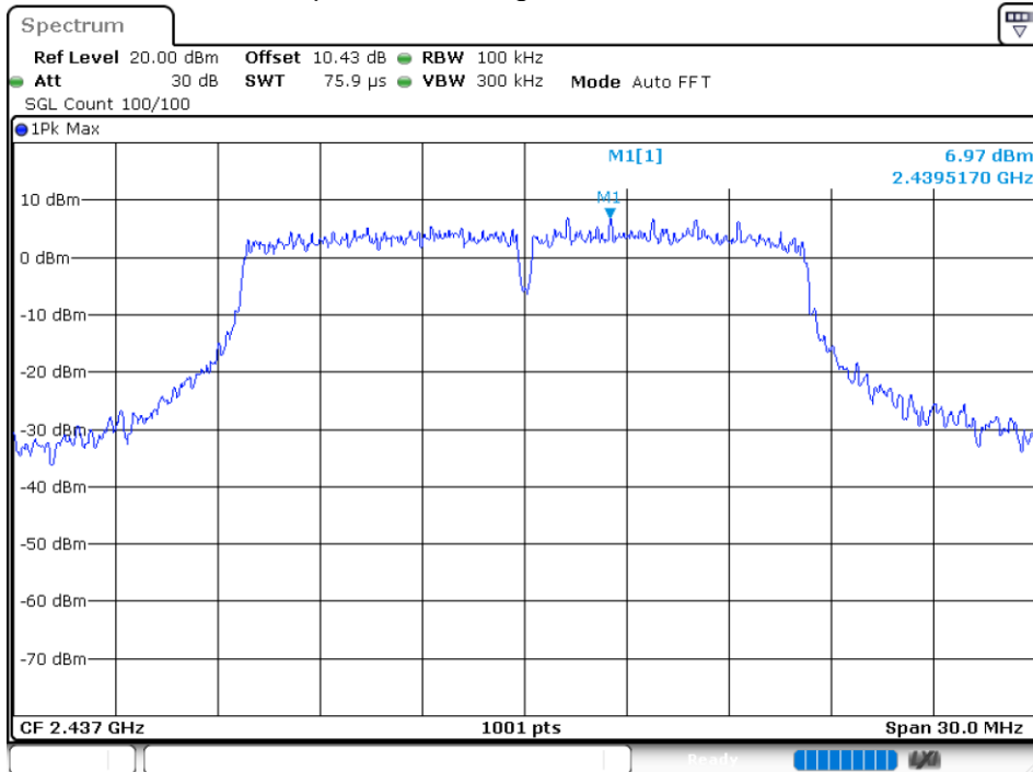
Tx. Spurious NVNT g 2437MHz Ant 4 Emission
