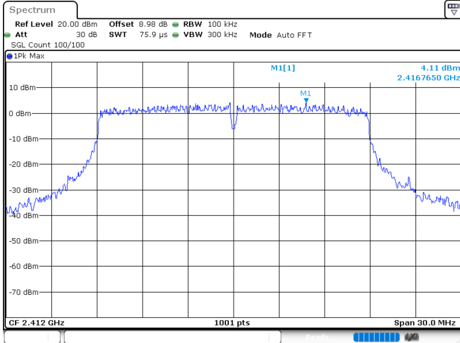
Band Edge NVNT n20 2412MHz Ant 3 Emission
