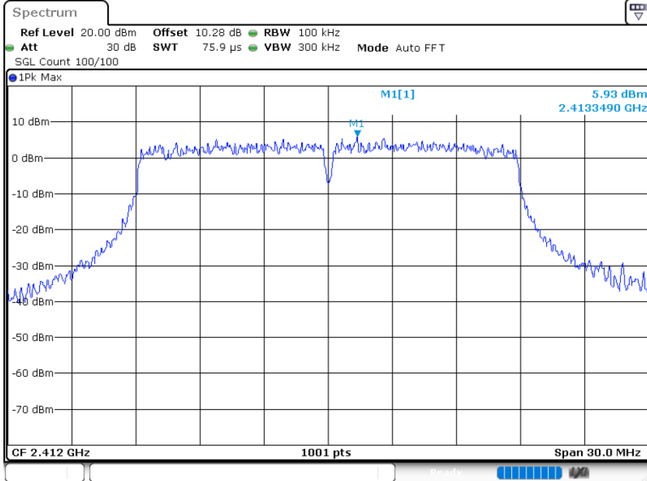
Band Edge NVNT n20 2412MHz Ant 4 Emission
