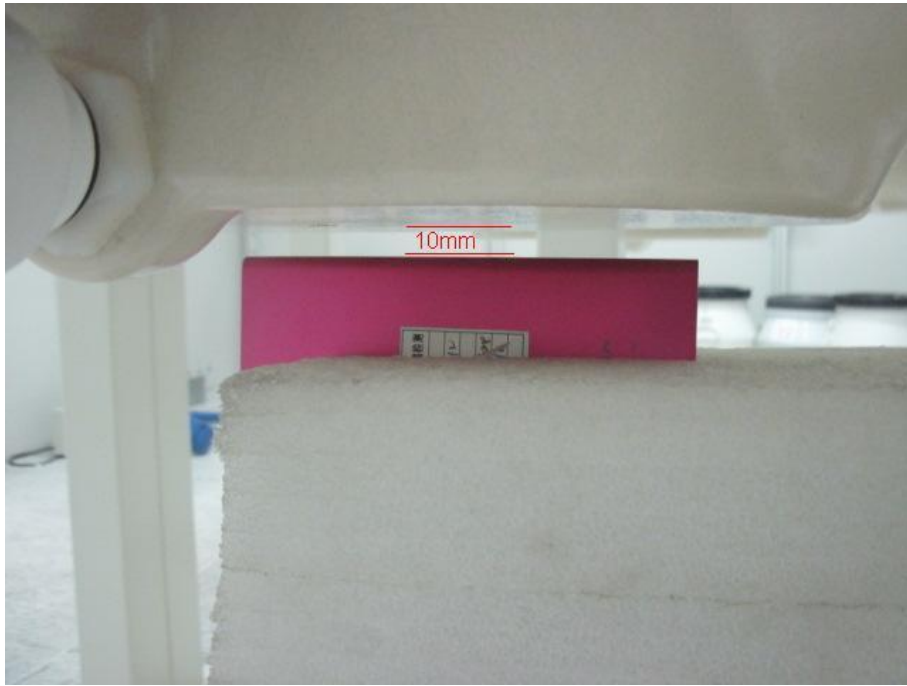
Body SAR Left Side 10mm for WLAN
