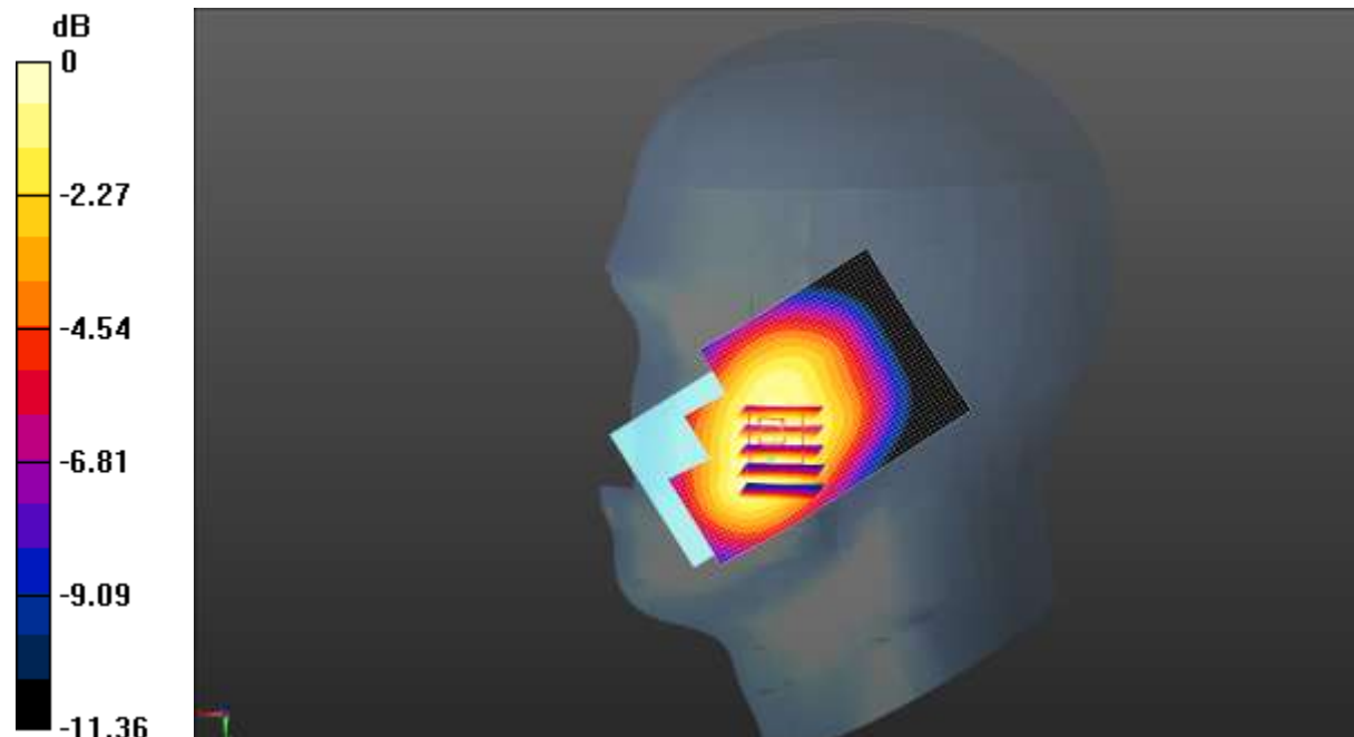
0 dB = 0.498 W/kg = -3.03 dBW/kg
