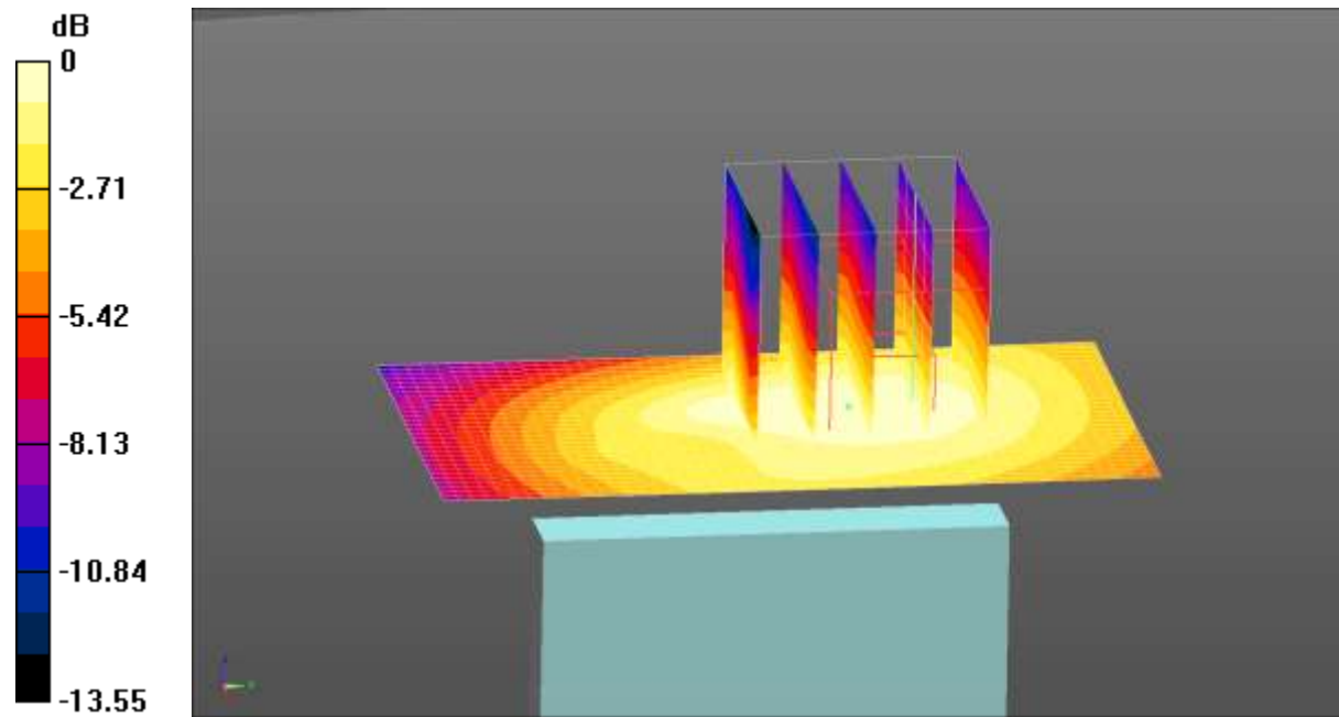
0 dB = 0.0405 W/kg = -13.93 dBW/kg
