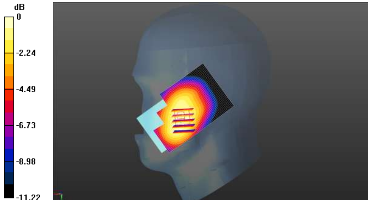
0 dB = 0.279 W/kg = -5.54 dBW/kg
