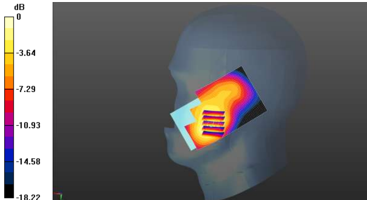
0 dB = 0.907 W/kg = -0.42 dBW/kg
