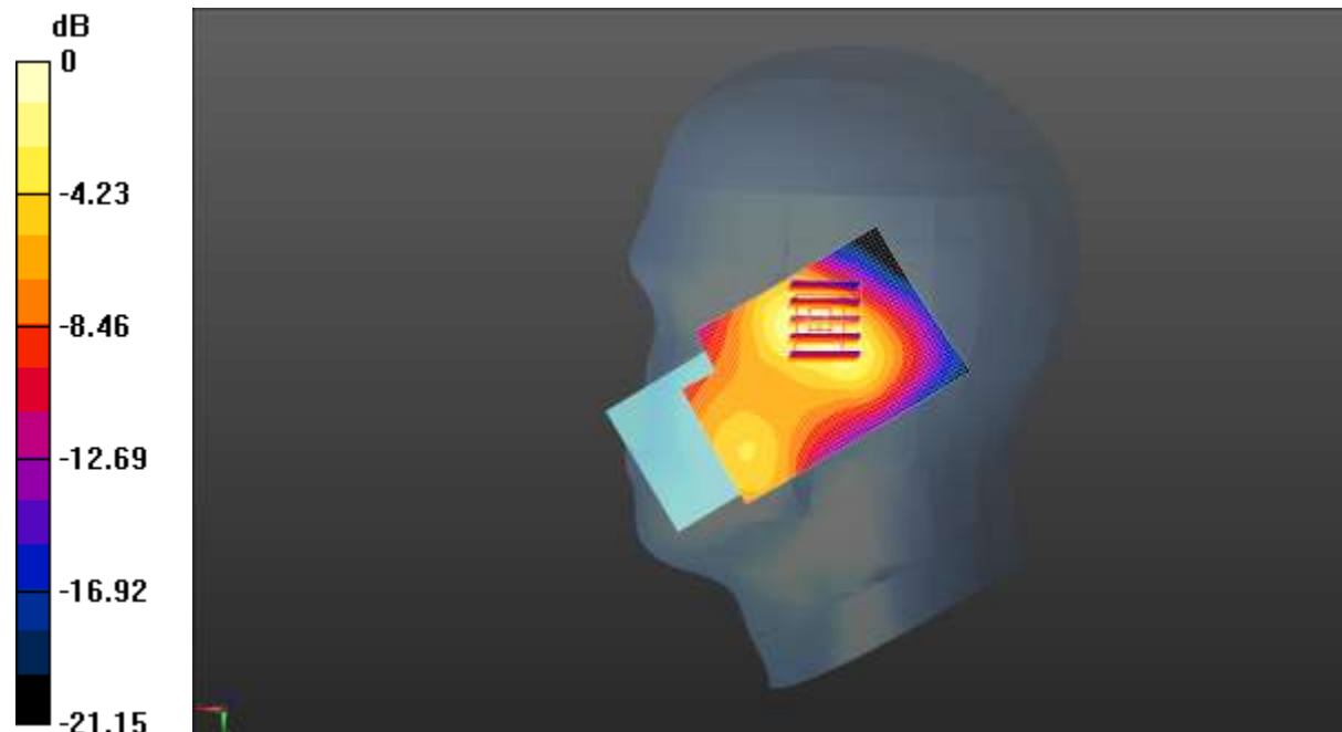
0 dB = 0.379 W/kg = -4.21 dBW/kg
