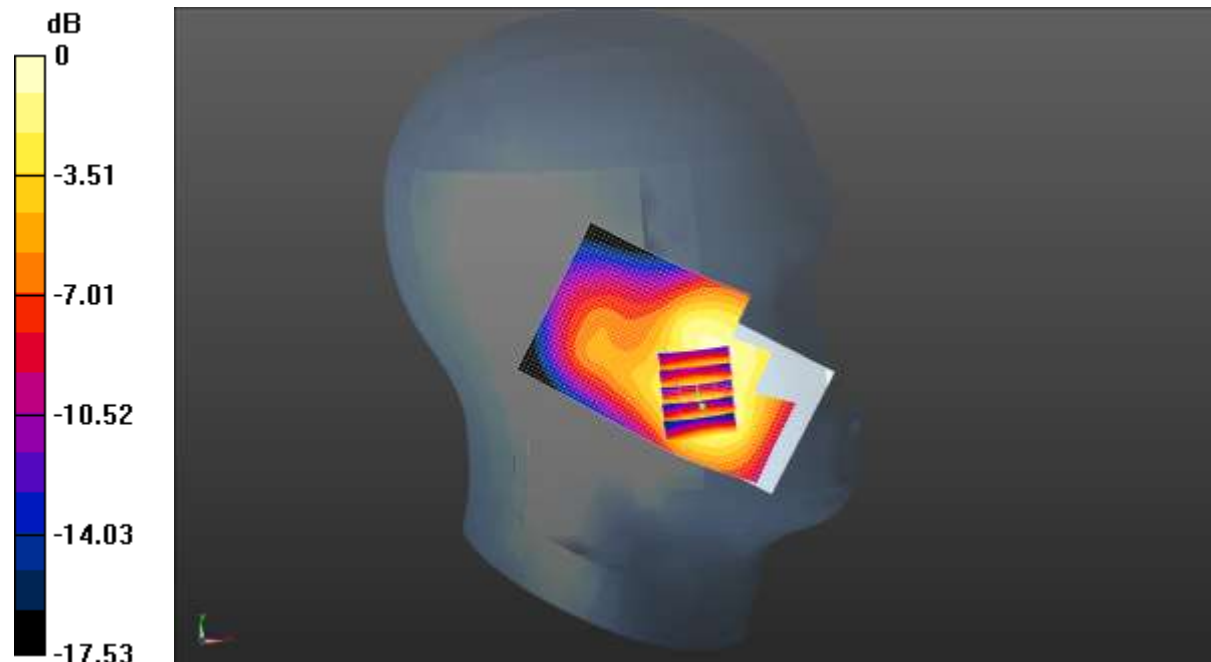
0 dB = 0.596 W/kg = -2.25 dBW/kg
