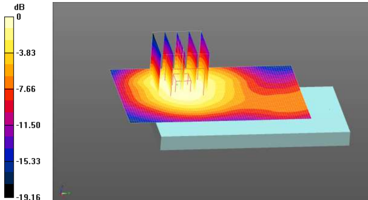
0 dB = 0.627 W/kg = -2.03 dBW/kg
