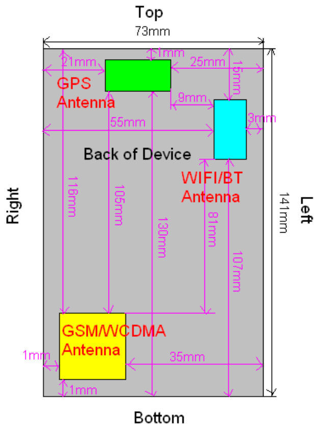
Mobile Hotspot Sides for SAR Testing
