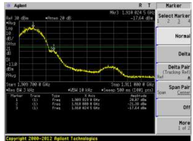
Channel 810 (1909.80MHz)
