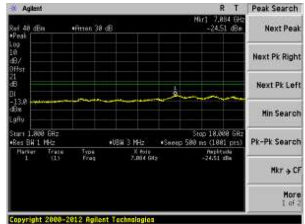
Channel 128 (824.20MHz)
