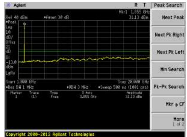
Channel 512 (1850.20MHz)
