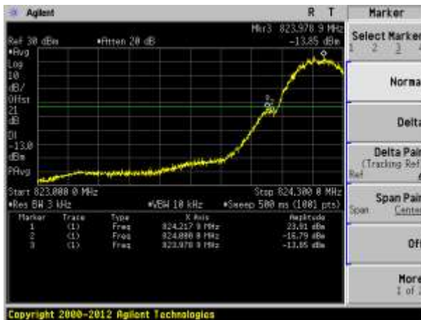
Channel 128 (824.20MHz)
