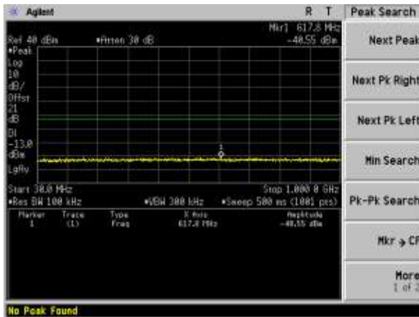
Channel 512 (1850.20MHz)
