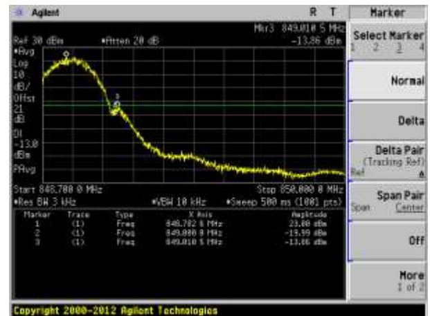
Channel 251 (848.80MHz)
