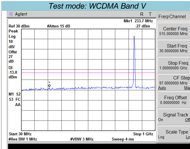
30MHz~1GHz
