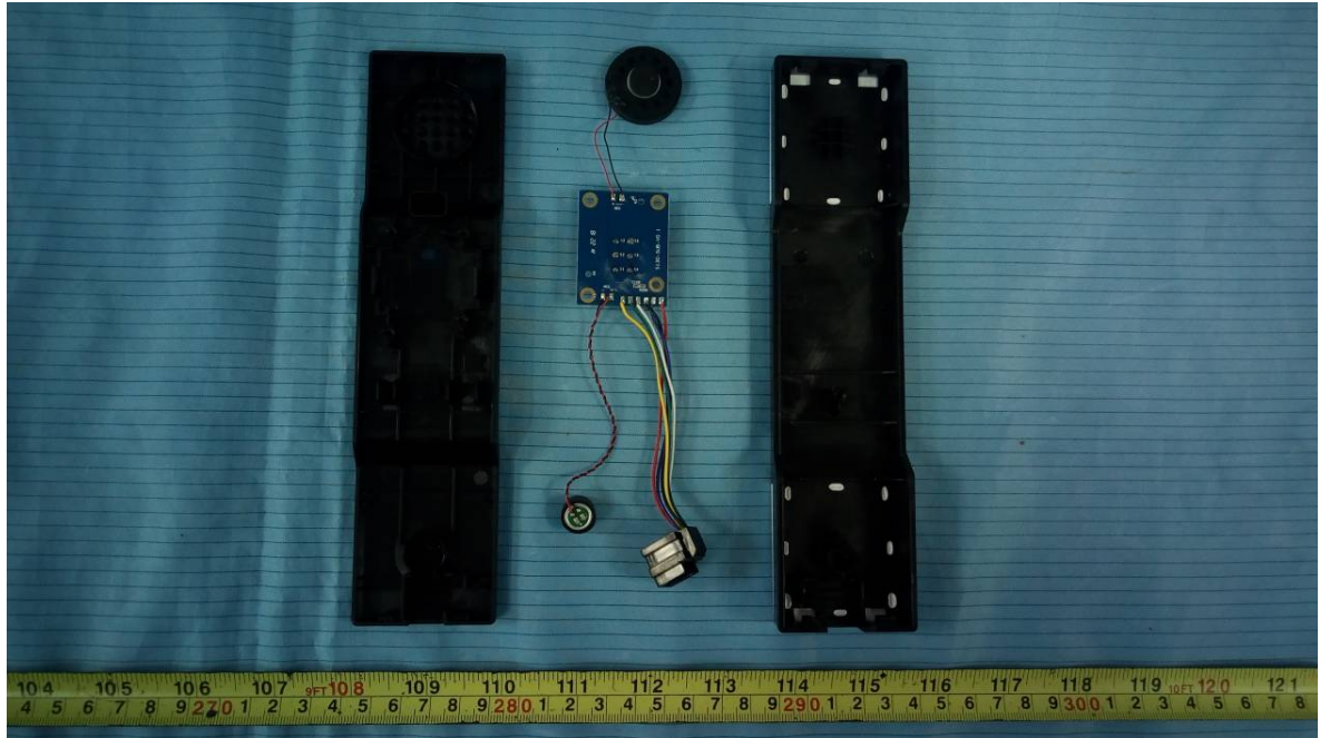
EUT (Handset) – Cover off View
