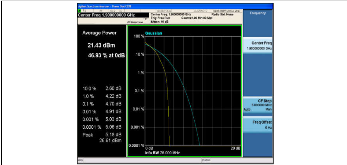
Band2_20MHz_16QAM_19100_1RB#0_4.95_13_PASS
