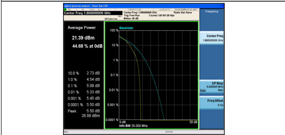
Band2_20MHz_16QAM_18700_1RB#0_5.28_13_PASS
