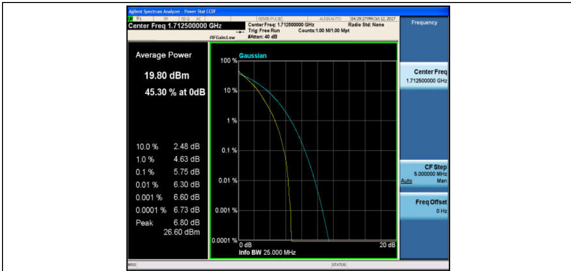
Band4_5MHz_16QAM_19975_25RB#0_6.65_13_PASS
