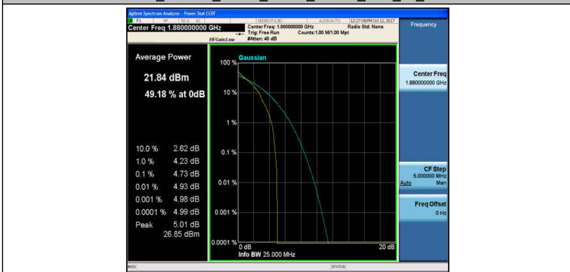
Band2_1.4MHz_16QAM_18900_1RB#0_5.29_13_PASS
