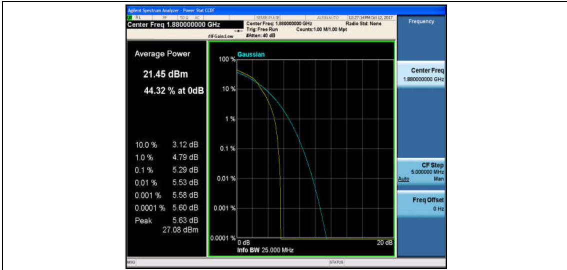
Band2_1.4MHz_QPSK_18900_6RB#0_5.16_13_PASS
