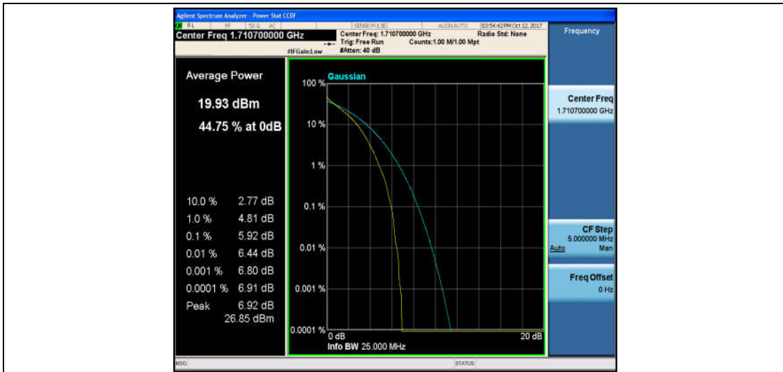
Band4_1.4MHz_16QAM_19957_6RB#0_6.93_13_PASS
