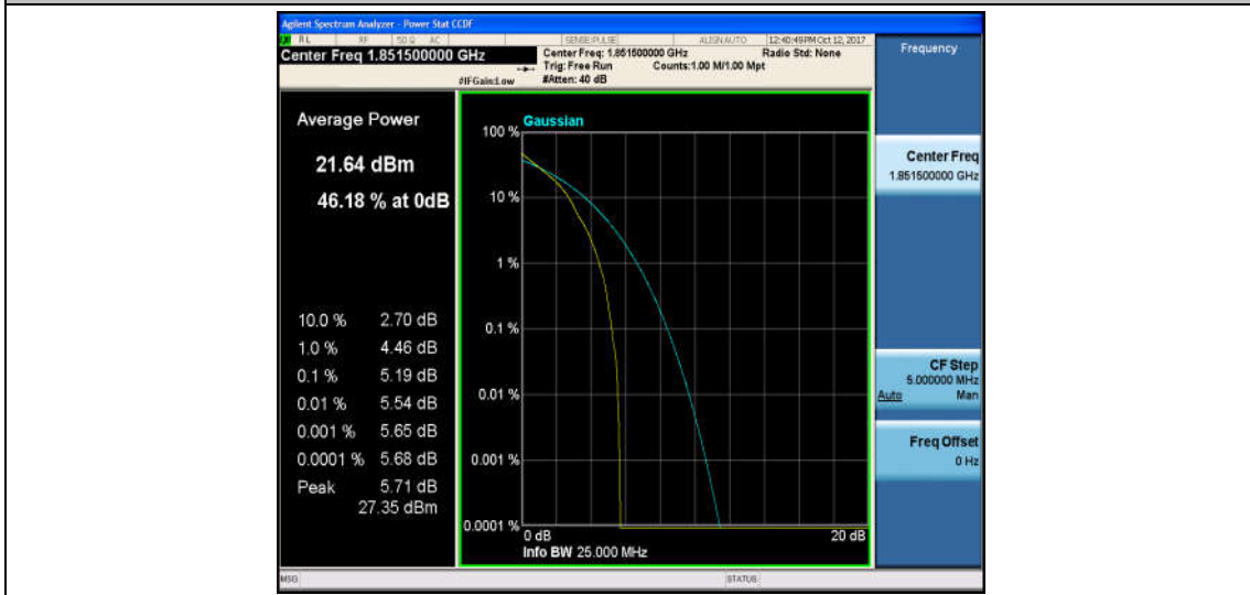
Band2_3MHz_16QAM_18615_1RB#0_6.05_13_PASS
