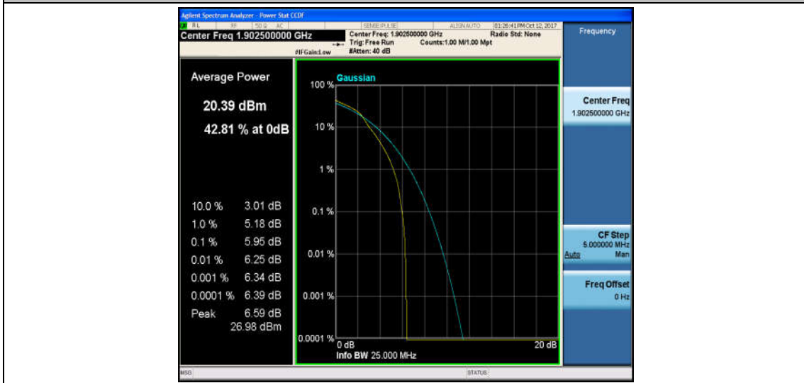
Band2_15MHz_QPSK_19125_75RB#0_5.46_13_PASS
