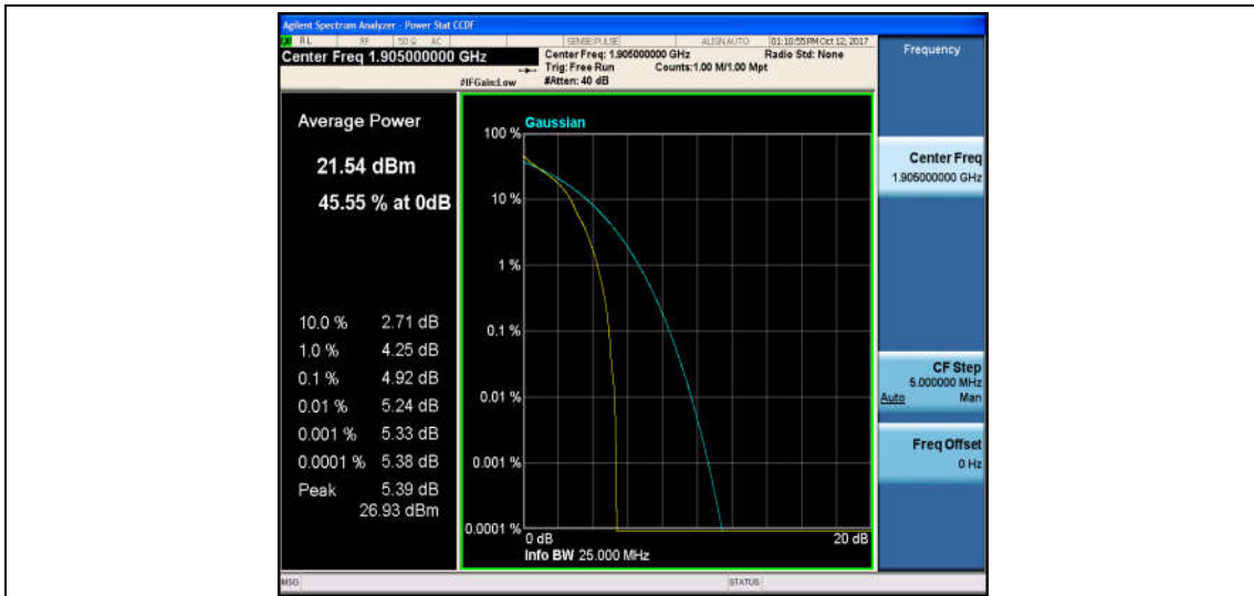
Band2_10MHz_16QAM_19150_1RB#0_5.59_13_PASS
