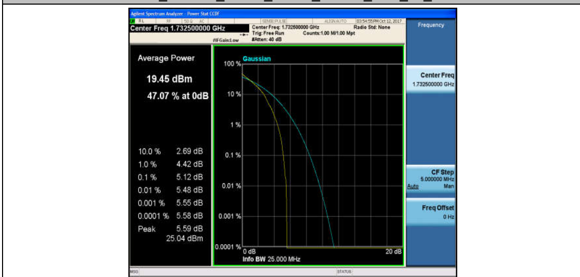
Band4_1.4MHz_16QAM_20175_1RB#0_5.44_13_PASS
