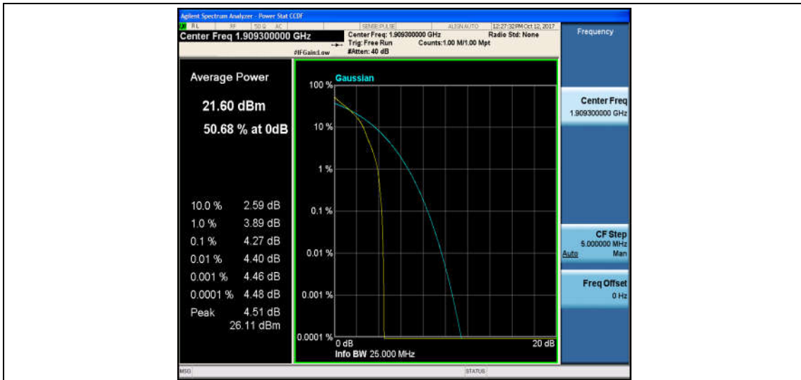
Band2_1.4MHz_16QAM_19193_1RB#0_5.14_13_PASS
