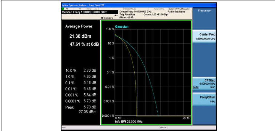
Band2_1.4MHz_16QAM_18900_6RB#0_6.15_13_PASS
