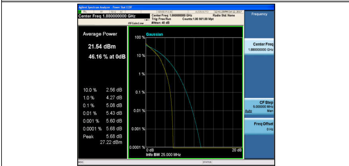
Band2_3MHz_16QAM_18900_15RB#0_6.11_13_PASS
