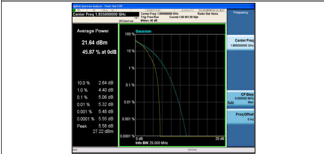
Band2_10MHz_16QAM_18650_1RB#0_6.03_13_PASS
