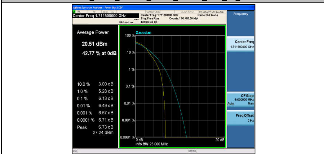
Band4_3MHz_QPSK_19965_15RB#0_5.79_13_PASS
