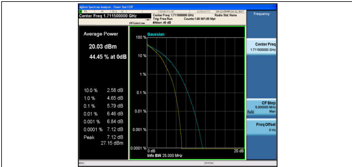
Band4_3MHz_16QAM_19965_15RB#0_6.68_13_PASS
