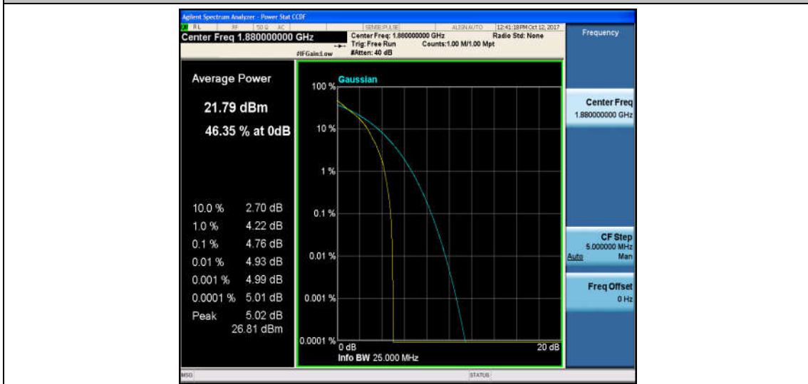
Band2_3MHz_16QAM_18900_1RB#0_4.98_13_PASS
