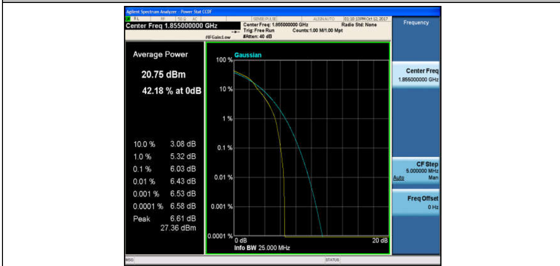
Band2_10MHz_QPSK_18650_50RB#0_5.58_13_PASS
