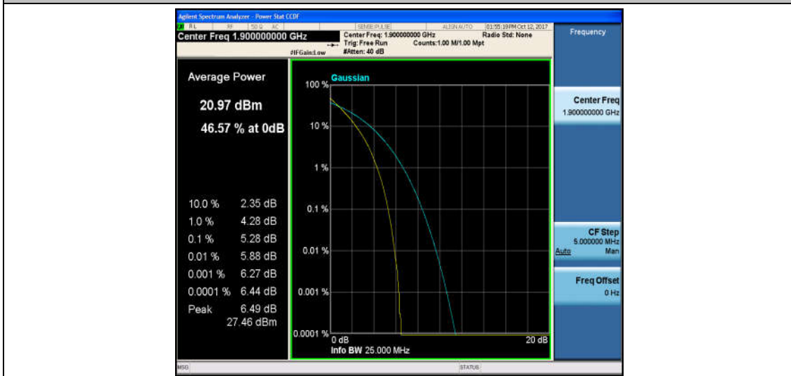
Band2_20MHz_16QAM_19100_100RB#0_6.15_13_PASS
