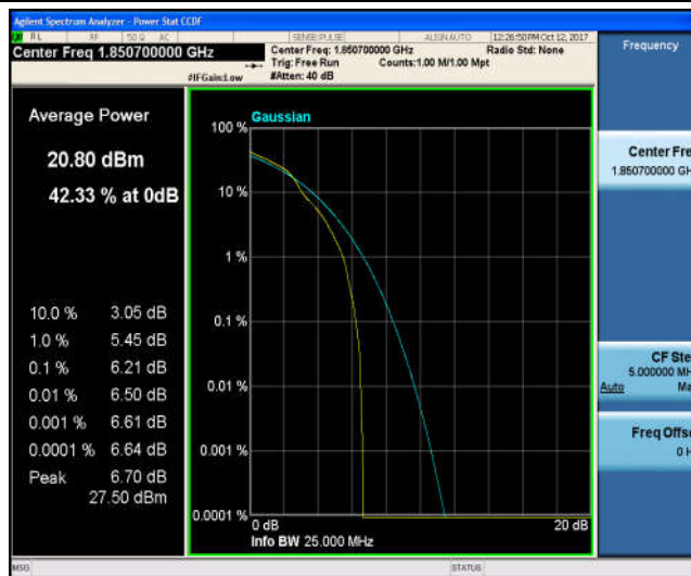
Band2_1.4MHz_QPSK_18607_6RB#0_5.77_13_PASS
