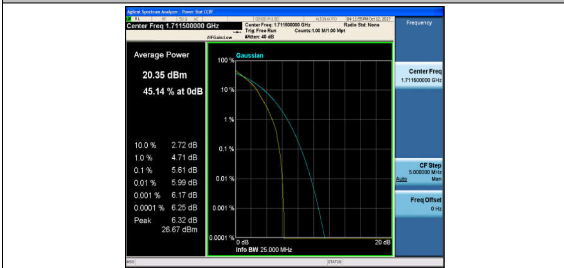
Band4_3MHz_16QAM_19965_1RB#0_6.13_13_PASS
