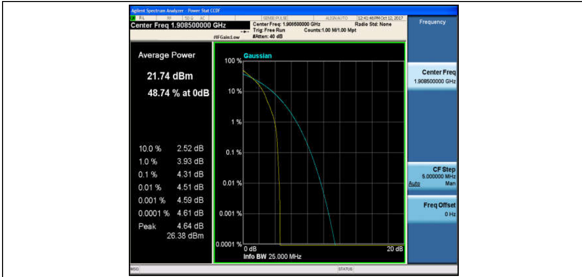
Band2_3MHz_16QAM_19185_1RB#0_4.88_13_PASS
