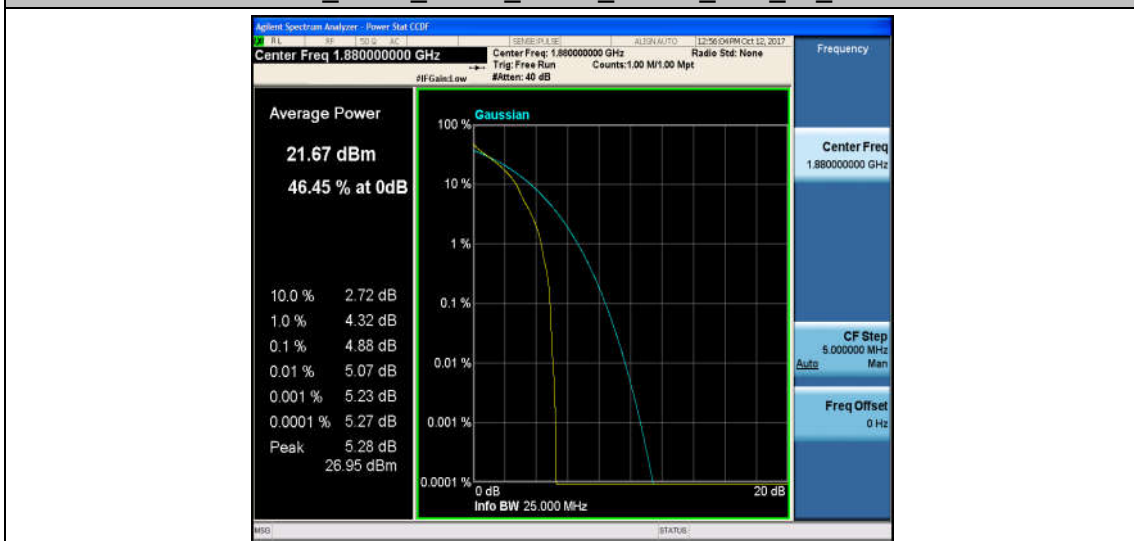
Band2_5MHz_16QAM_18900_1RB#0_5.55_13_PASS
