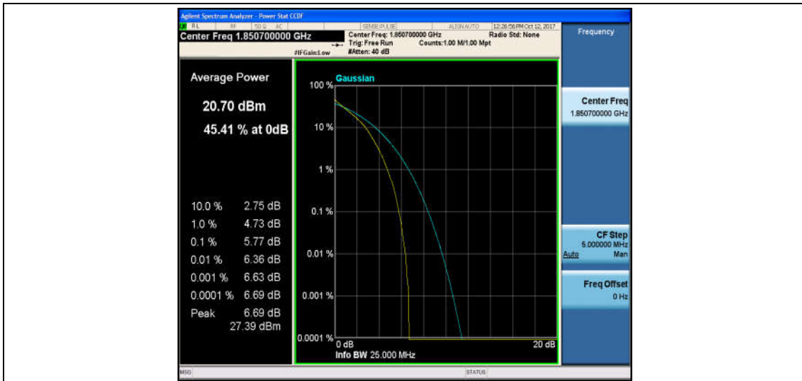
Band2_1.4MHz_16QAM_18607_6RB#0_6.69_13_PASS
