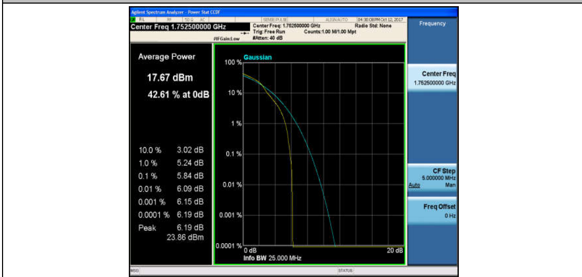
Band4_5MHz_QPSK_20375_25RB#0_5.25_13_PASS
