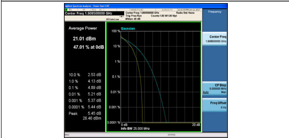
Band2_3MHz_16QAM_19185_15RB#0_5.80_13_PASS
