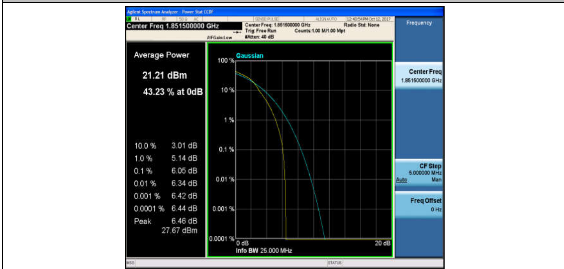
Band2_3MHz_QPSK_18615_15RB#0_5.68_13_PASS
