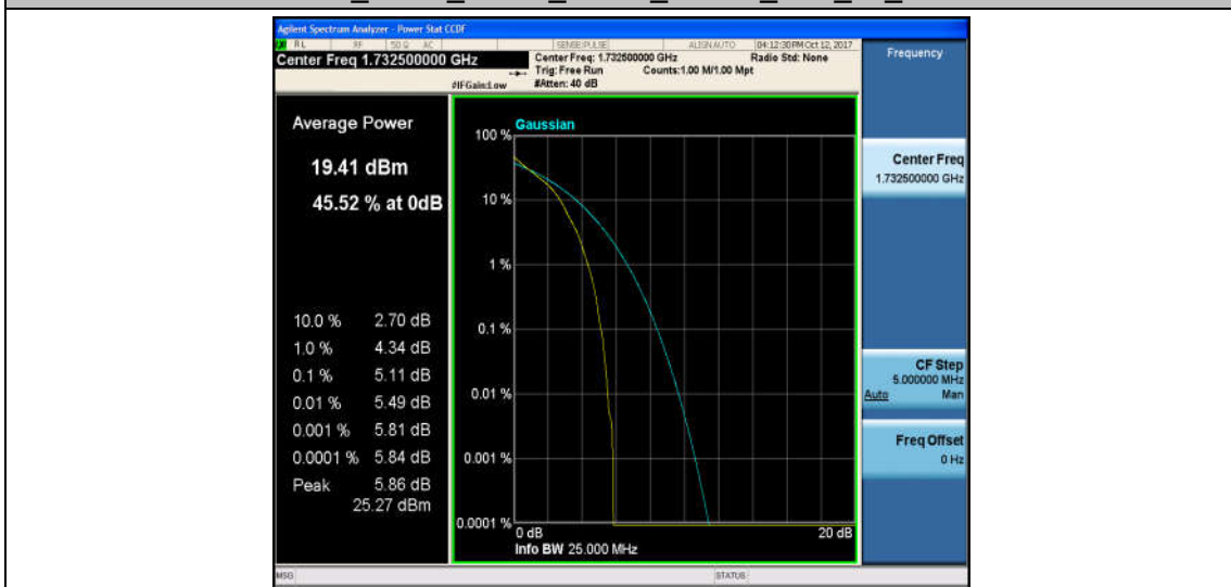
Band4_3MHz_16QAM_20175_1RB#0_5.45_13_PASS
