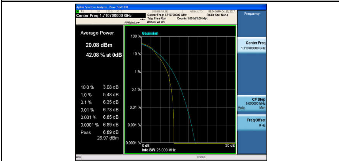
Band4_1.4MHz_QPSK_19957_6RB#0_5.92_13_PASS
