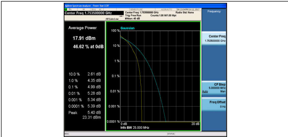
Band4_3MHz_16QAM_20385_1RB#0_5.16_13_PASS
