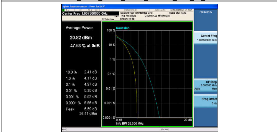
Band2_5MHz_16QAM_19175_25RB#0_5.84_13_PASS
