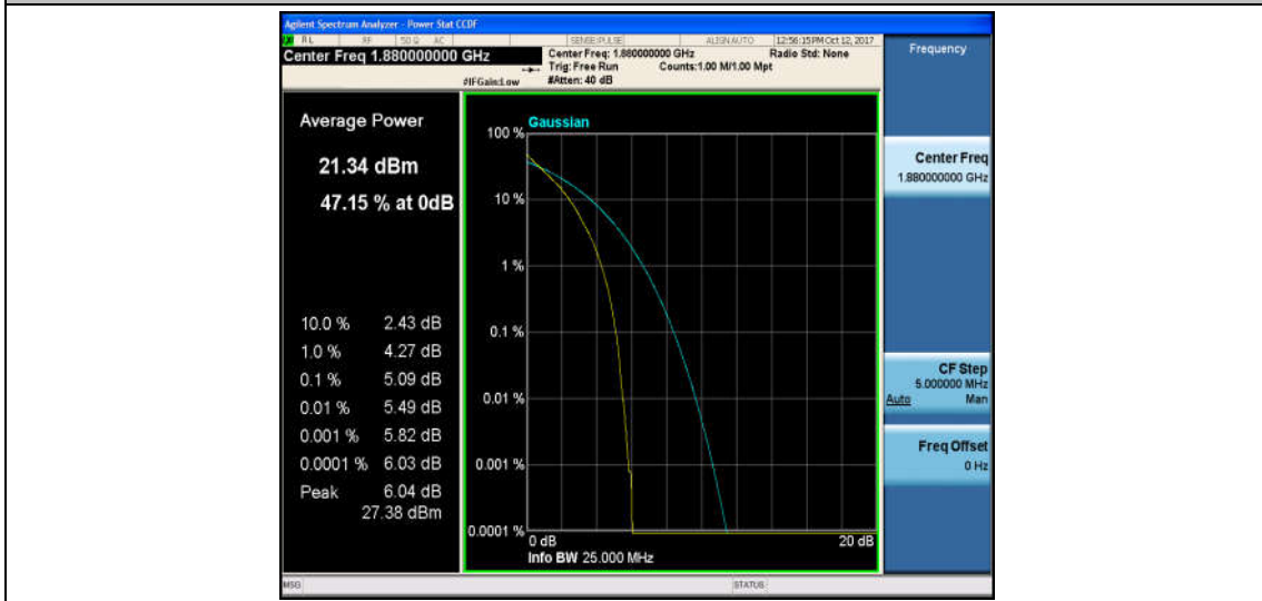
Band2_5MHz_16QAM_18900_25RB#0_5.98_13_PASS
