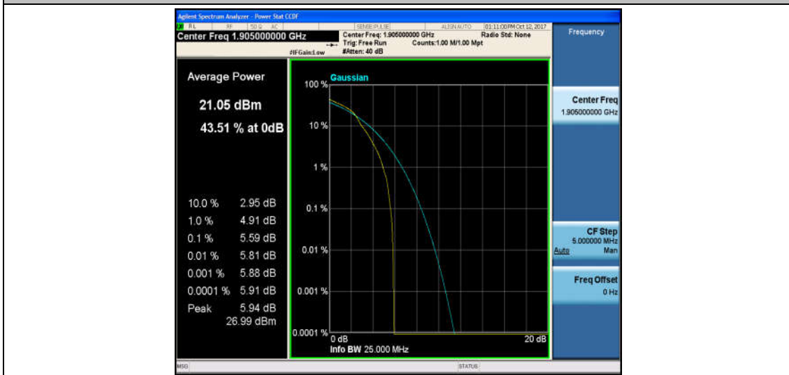
Band2_10MHz_QPSK_19150_50RB#0_5.00_13_PASS
