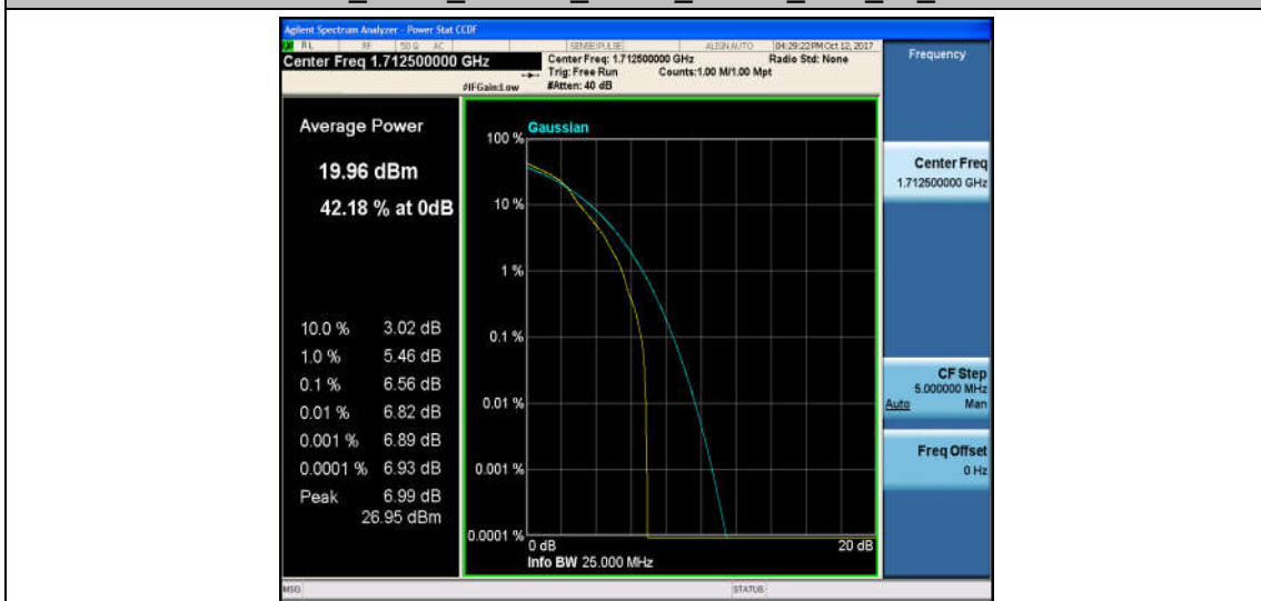
Band4_5MHz_QPSK_19975_25RB#0_5.75_13_PASS
