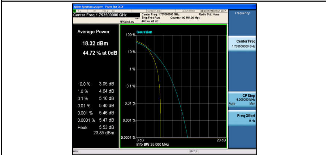
Band4_3MHz_QPSK_20385_15RB#0_5.18_13_PASS
