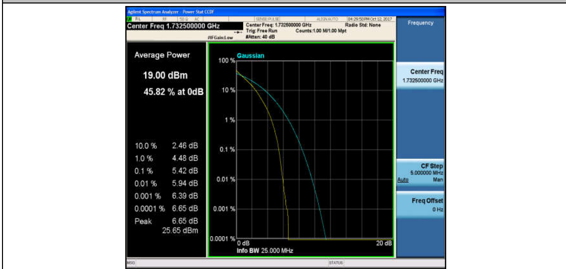
Band4_5MHz_16QAM_20175_25RB#0_6.24_13_PASS
