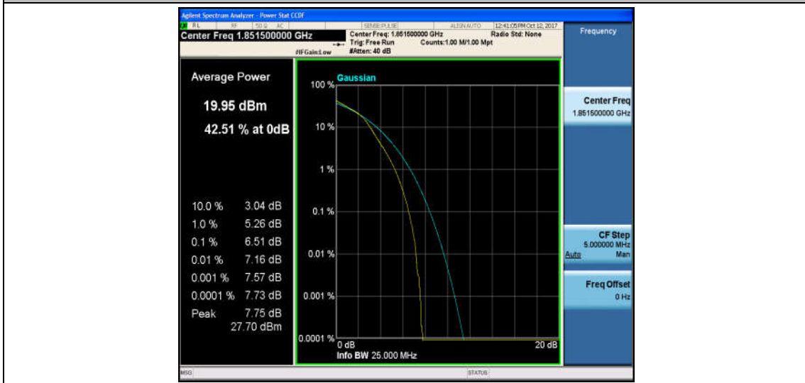
Band2_3MHz_QPSK_18900_1RB#0_4.76_13_PASS
