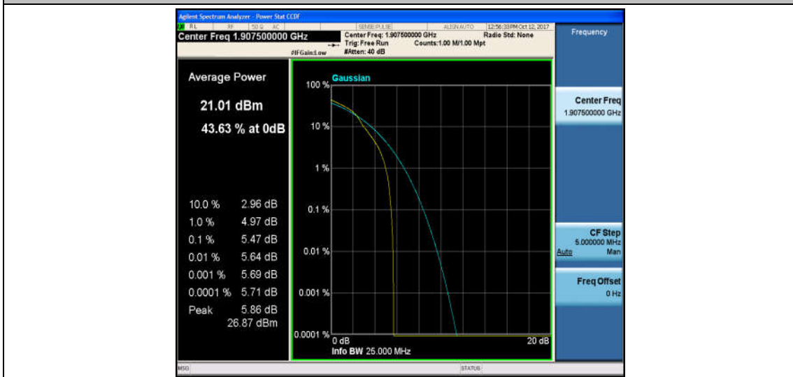
Band2_5MHz_QPSK_19175_25RB#0_4.97_13_PASS
