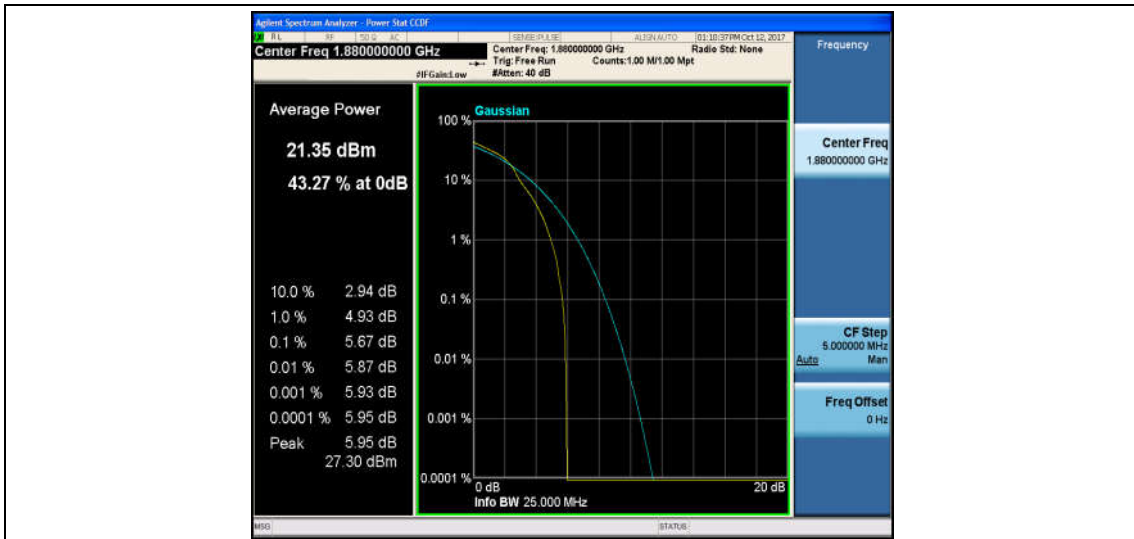
Band2_10MHz_QPSK_18900_50RB#0_5.02_13_PASS
