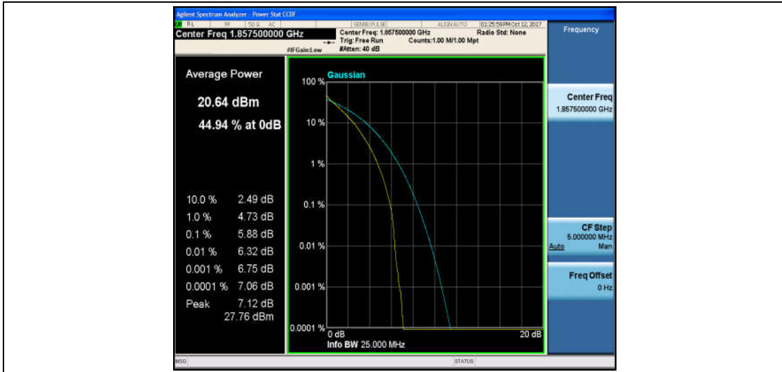
Band2_15MHz_16QAM_18675_75RB#0_6.44_13_PASS
