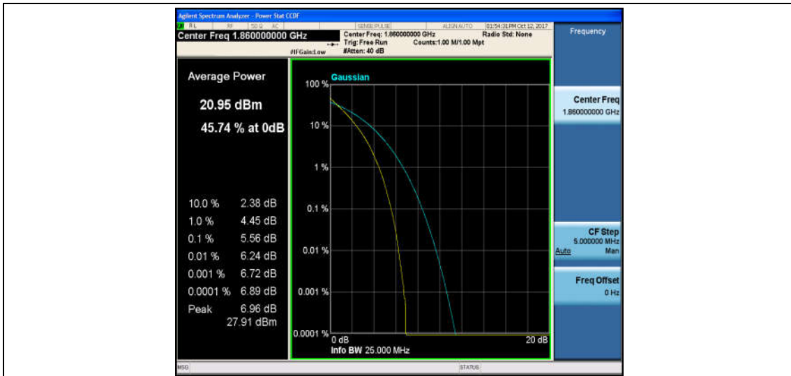
Band2_20MHz_16QAM_18700_100RB#0_6.42_13_PASS
