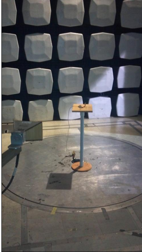
Photograph 3. Radiated Spurious Emissions, Test Setup, 1 GHz – 10 GHz
