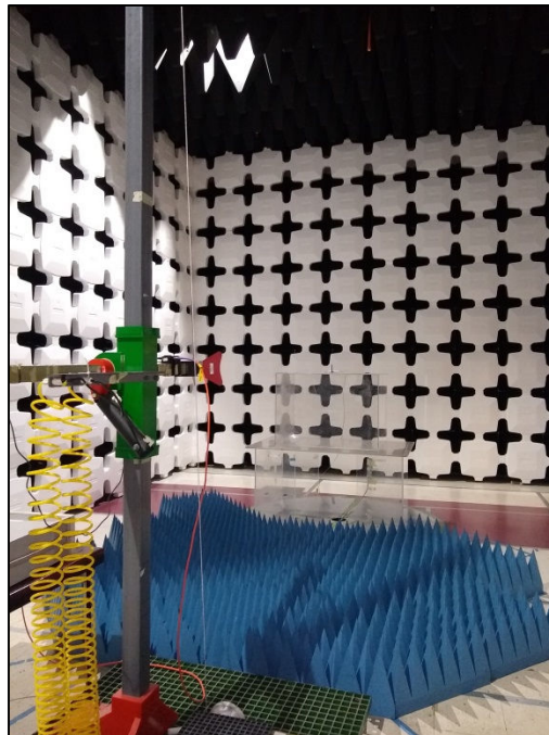
Photograph 2: Radiated Spurious Emissions, Above 1GHz, Chip Antenna Test Setup
