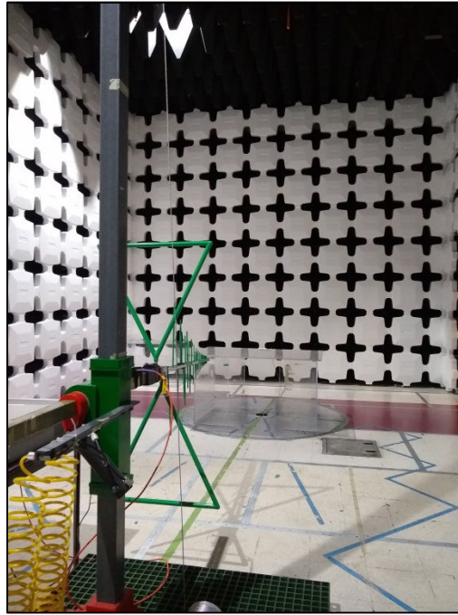
Photograph 1: Radiated Spurious Emissions, Below 1GHz, Chip Antenna Test Setup
