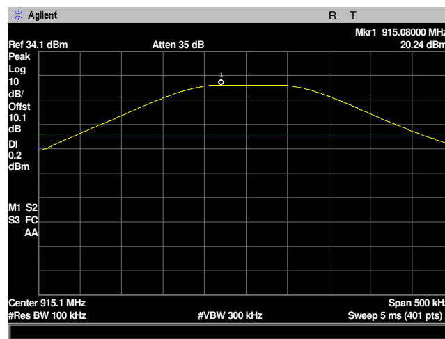
Plot 33: RF Conducted Band Edge, Reference Level Mid Channel
