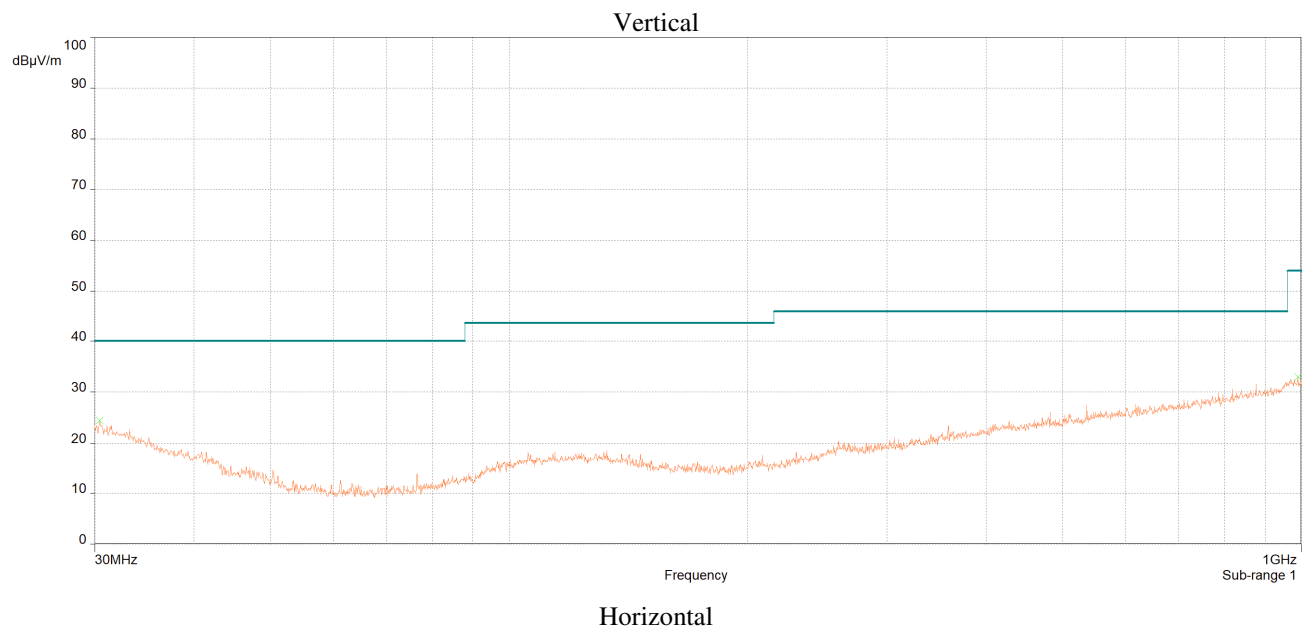
Plot 13: Radiated Emissions, 30 MHz - 1 GHz, (worst case)
