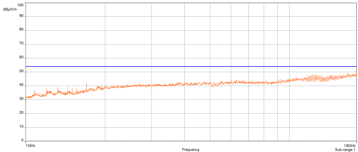
Plot 14: Radiated Spurious Emissions Requirements, Low Channel, Average (Chip Antenna)
