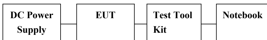
Fig. 2-3 Conduction Emission
