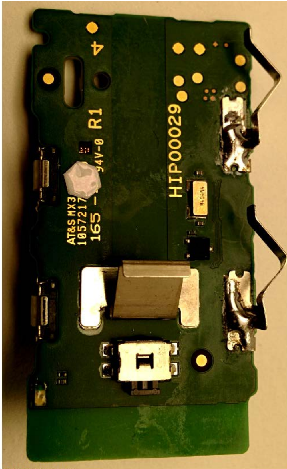
Figure 2: PCB View 2
