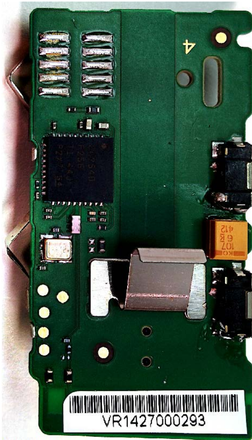
Figure 1: PCB View 1
